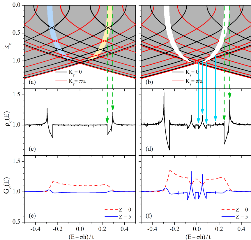
FIG. 4. (color online) Numerical simulations illustrating the situation with reduced Zeeman field h/\Delta_{\text{BCS}} . The figures are the same as Figs. 2(c)–(h) except \Delta_q = 0.025 and a = 20 .
