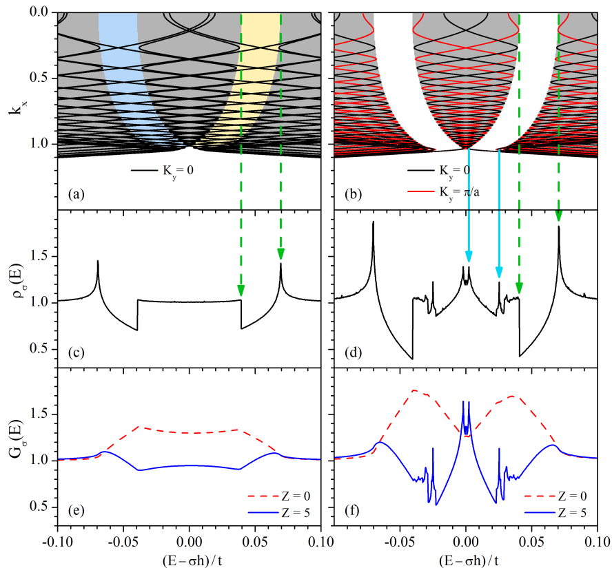
FIG. 3. (color online) Numerical simulations illustrating the situation with weak pairing interaction. The figures are the same as Figs. 2(c)–(h) except \Delta_q = 0.015 and a = 100 . The energy range is changed to [-0.1, 0.1] as a result of the small \Delta_q compared with Fig. 2.
