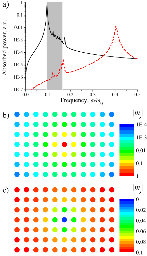
FIG. 9. Spin wave absorption spectra (a) and mode structure ((b) and (c)) in a magnetic dot array in a ferromagnetic (FM) ground state having one defect per 11 \times 11 dots. Dot aspect ratio h/R = 5 , lattice constant a/R = 4 . (a) Solid curve – absorption spectrum for the microwave signal having right in-plane polarization (i.e., \mathbf{b}_e = (b \cos \omega t, b \sin \omega t, 0) ). The main peak at \omega = 0.095 \omega_M corresponds to the FMR frequency of the array. Dashed curve – absorption spectrum for the signal having left in-plane polarization. The peak at \omega = 0.4 \omega_M corresponds to the localized “defect” spin wave mode. Gray area – region of existence of spin wave modes in a perfect (without defect) dot array. (b) and (c) – spatial profiles of the localized ( \omega = 0.4 \omega_M ) and FMR ( \omega = 0.095 \omega_M ) spin wave modes in the dot array with a defect.
