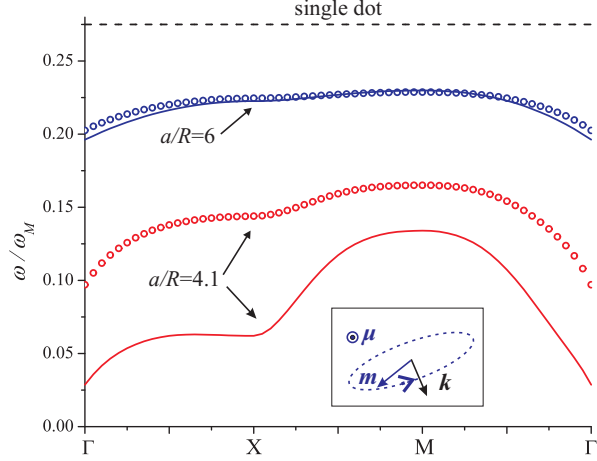
FIG. 5. (Color online) Spectra of collective spin waves of a square array of cylindrical magnetic dots (aspect ratio is h/R = 5 ) in a ferromagnetic (FM) ground state without external magnetic field. The contour \Gamma \rightarrow X \rightarrow M \rightarrow \Gamma is shown in Fig. 4c. Open circles – calculations using Eq. (3.38) with account of the real shape of the nano-dots; solid lines – calculations in point-dipole approximation 24 . The lower pair of curves corresponds to the array's lattice constant a = 4.1R and the upper pair to a = 6R . The upper dashed line shows the resonance frequency of a single dot. Inset: vector structure of the dynamical magnetization \mathbf{m}_{\mathbf{k}} of a spin wave with wavevector \mathbf{k} .
