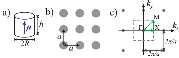
FIG. 4. (Color online) (a) Geometry of the nano-dots. (b) Square lattice of the array. (c) Reciprocal lattice (gray circles) of the array. Dashed line – boundary of the first Brillouin zone in the ferromagnetic state. Green arrows show the contour \Gamma \rightarrow X \rightarrow M \rightarrow \Gamma of the spectrum plot in Fig. 5.
