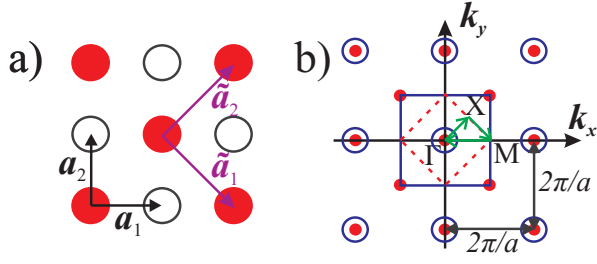
FIG. 6. (Color online) (a) Square array of magnetic dots in a chessboard antiferromagnetic (CAFM) ground state. Empty and filled circles represent the dots with opposite directions of the equilibrium magnetization \boldsymbol{\mu}_j = \pm \mathbf{e}_z . (b) Reciprocal lattice \mathcal{L}^* (larger open circles) and reciprocal superlattice \mathcal{SL}^* (smaller filled circles). The solid (dashed) lines in the middle show the boundaries of the first Brillouin zone for the reciprocal fundamental lattice (reciprocal superlattice). The solid arrows in the middle show the contour \Gamma \rightarrow X \rightarrow M \rightarrow \Gamma of the spectrum plot in Fig. 7.
