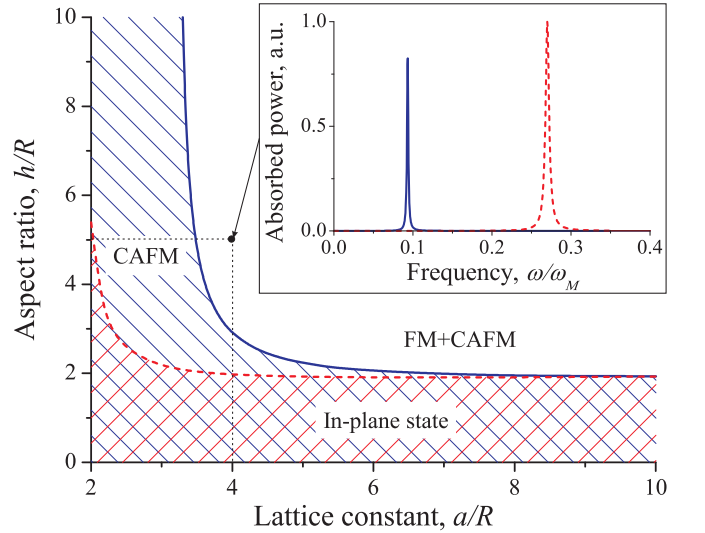
FIG. 8. (Color online) Regions of stability of different ground states of a magnetic dot array in zero applied field: above the solid blue line both the FM and the CAFM ground states are stable; below the solid blue line, but above the dashed red line only the CAFM ground state is stable; below the dashed red line both FM and CAFM states are unstable and array switches to a state with in-plane direction of the dot static magnetization. Black dot indicates the point at which the absorption spectra shown in the inset were calculated. Inset: normalized spin wave absorption spectra of the array of Permalloy cylindrical dots in the FM (solid blue curve) and CAFM (dashed red curve) ground states. Parameters: a/R = 4 , h/R = 5 , \omega_M/2\pi \approx 30 GHz, \alpha_G = 0.01 , polarization of the exciting microwave field – linear in the array’s plane.
