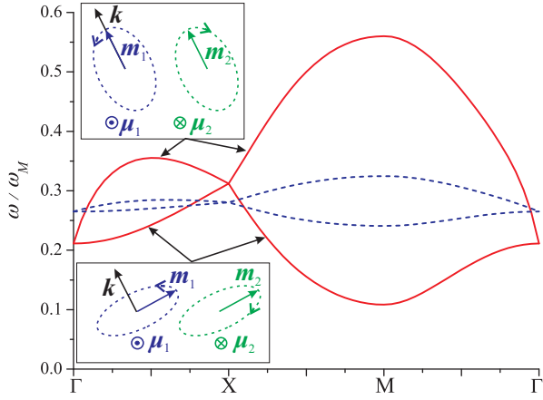
FIG. 7. (Color online) Spectra of collective spin waves of a square array of cylindrical magnetic dots (aspect ratio is h/R = 5 ) in a chessboard antiferromagnetic (CAF) ground state without external magnetic field. The solid (red) lines correspond to the lattice constant a = 2.5R while the blue dashed lines to a = 5R . Insets: vector structures of dynamical magnetization \mathbf{m}_p of the high-frequency (upper inset) and low-frequency (lower inset) spin wave branches.
