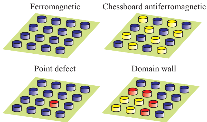
FIG. 1. (Color online) Examples of periodic (upper frames) and aperiodic (lower frames) ground states of an array of magnetic nano-dots. Different colors represent different magnetization direction (for the antiferromagnetic state – the directions are opposite).
