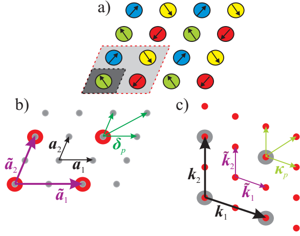
FIG. 3. (Color online) Example of a complex periodic ground state of a magnetic dot array, the so-called non-collinear anti-ferromagnetic state 8 . (a) Equilibrium magnetization distribution forming a periodic superlattice \mathcal{S} . The light gray area shows a unit cell of the superlattice \mathcal{S} , which is P = 4 times larger than the unit cell of the fundamental lattice \mathcal{L} (dark gray area). (b) Direct lattice \mathcal{L} (small gray circles) formed by the basis vectors \mathbf{a}_1, \mathbf{a}_2 and the superlattice \mathcal{S} (large red circles) formed by the vectors \tilde{\mathbf{a}}_1, \tilde{\mathbf{a}}_2 . The lattice \mathcal{L} is P = 4 times denser than the superlattice \mathcal{S} and can be restored by translating the superlattice \mathcal{S} using shift vectors \delta_p (green arrows). (c) Reciprocal lattice \mathcal{L}^* (large gray circles) and reciprocal superlattice \mathcal{S}^* (small red circles) with basis vectors \mathbf{k}_i and \tilde{\mathbf{k}}_i , respectively. The reciprocal superlattice \mathcal{S}^* is denser than \mathcal{L}^* and is restored by translating \mathcal{L}^* using shift wavevectors \kappa_p (green arrows).
