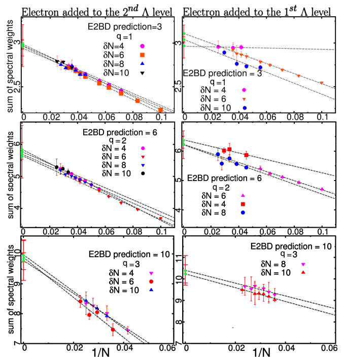
FIG. 6. (Color online) Spectral weight sums as a function of N for q = 1, 2 and 3 . The columns on the right are for a composite fermion added to the lowest \Lambda level, whereas those on the left are for a composite fermion added to the second \Lambda level. The values predicted by the E2BD are shown in the figures. The thermodynamic limits of the sums are consistent with these values in all cases. Here \delta N = N_1 - N_2 .
