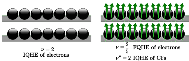
FIG. 1. (Color online) Schematic of \nu = 2/5 state in the composite fermion theory. Only the bulk structure is shown.
