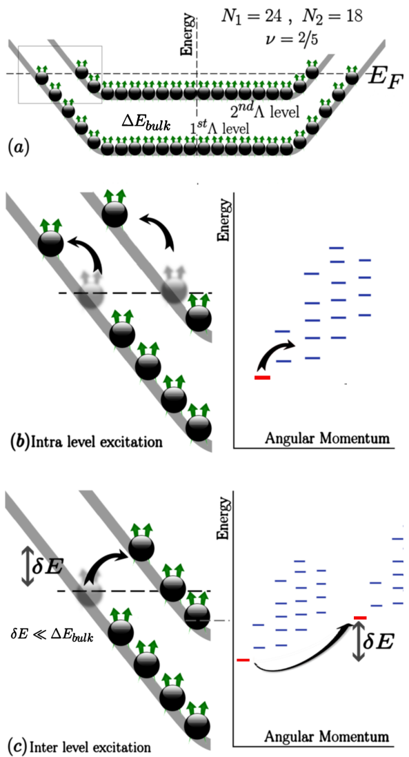
FIG. 2. (Color online) A schematic diagram of \nu = 2/5 edge. Panel (a) shows a compact ground state for the sector with N_1 and N_2 CFs in the lowest and second \Lambda levels respectively. Excitations at the edge can be intra \Lambda level or inter \Lambda level. In an intra \Lambda level excitation (Panel b), the number of electrons in the individual \Lambda levels do not change. In an inter \Lambda level excitation (Panel c), the electron makes a transition from one \Lambda level to another, connecting the state to a neighboring sector as shown in the accompanying spectrum.
