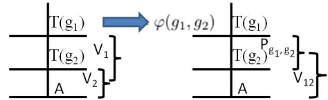
FIG. 8. Two ways of reducing the combination of T(g_2) , T(g_1) and A into A . Only the right projection operators are shown. Their combined actions differ by a phase factor \varphi(g_1, g_2) .
