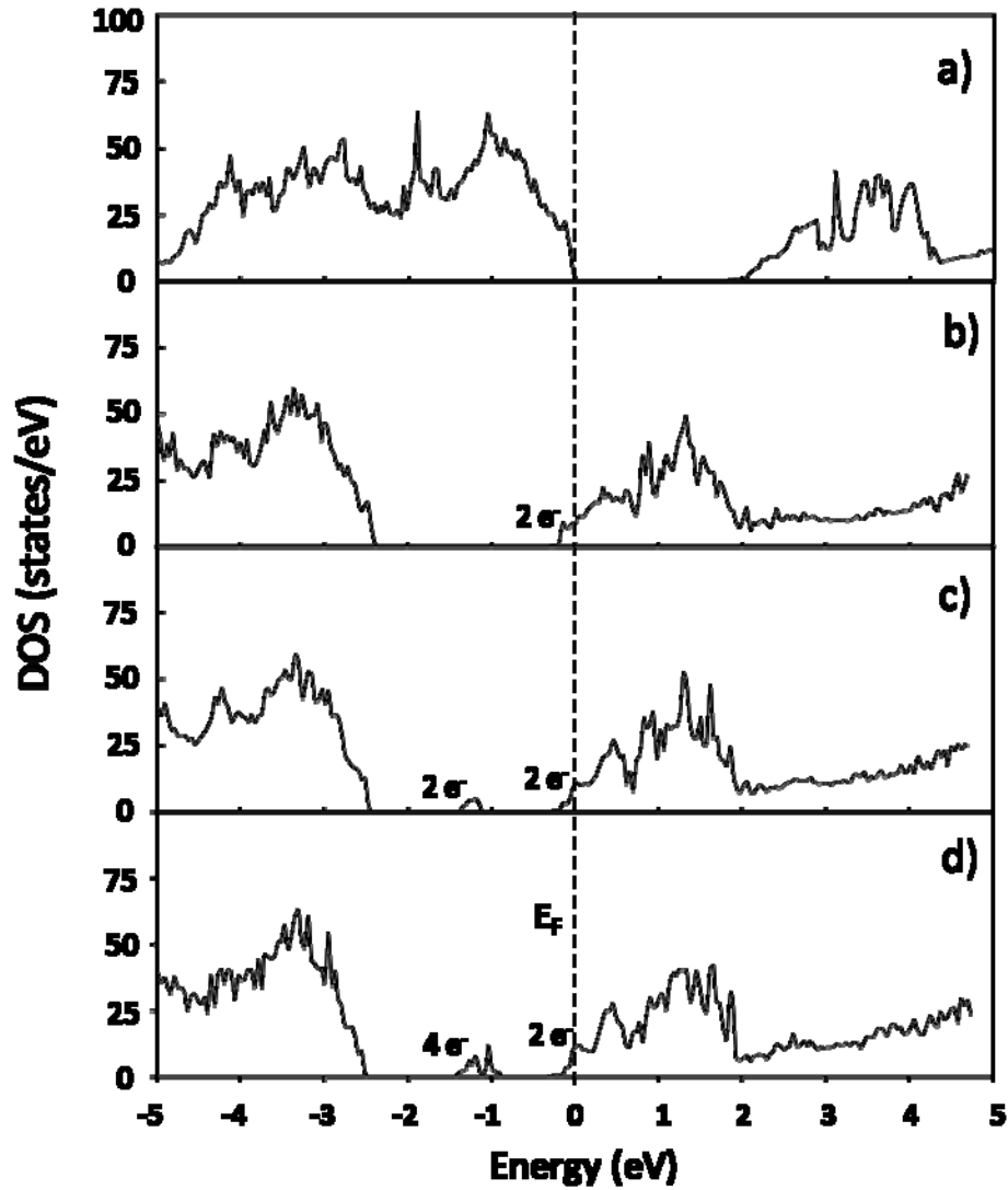
FIG. 9. Density of states of a) \text{SrTi}_{0.6}\text{Nb}_{0.2}\text{Ga}_{0.2}\text{O}_3 , b) \text{SrTi}_{0.6}\text{Nb}_{0.2}\text{Ga}_{0.2}\text{O}_{2.95} , c) \text{SrTi}_{0.6}\text{Nb}_{0.2}\text{Ga}_{0.2}\text{O}_{2.9} , and d) \text{SrTi}_{0.6}\text{Nb}_{0.2}\text{Ga}_{0.2}\text{O}_{2.85} . Fermi energy is set to zero on the energy scale. Numbers of electrons shown in the figure indicate the integrated number of electrons per supercell for the specified DOS area, i.e., states in the band gap and states below the Fermi level.
