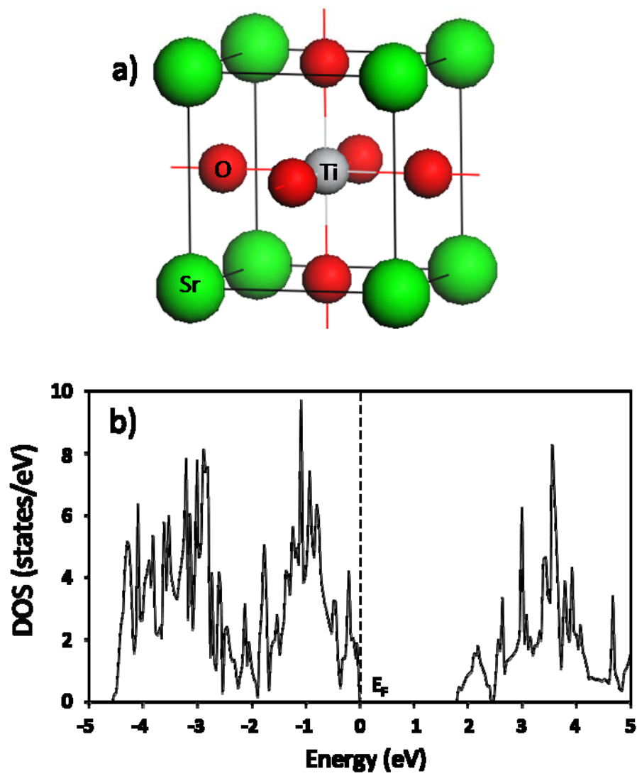
FIG. 1. (Color Online) a) Unit cell of SrTiO 3 perovskite oxide b) Density of states of stoichiometric SrTiO 3 with calculated band gap of 1.80 eV.
