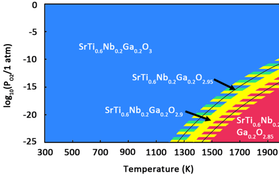
FIG. 8. (Color Online) Calculated phase diagram of 20% Ga- and 20% Nb-doped \text{SrTiO}_3 . Differently shaded areas mark the stability regions of various structures for a given temperature and partial pressure of oxygen. The hatched area describes possible changes in the phase diagram if computed reaction energies shown in Table 1 are off by \pm 0.2 eV (our estimated error bar). Blue, yellow, and red areas symbolize stability of \text{SrTi}_{0.6}\text{Nb}_{0.2}\text{Ga}_{0.2}\text{O}_3 , \text{SrTi}_{0.6}\text{Nb}_{0.2}\text{Ga}_{0.2}\text{O}_{2.9} , and \text{SrTi}_{0.6}\text{Nb}_{0.2}\text{Ga}_{0.2}\text{O}_{2.85} , respectively. The hatched green area symbolizes the stability of a \text{SrTi}_{0.6}\text{Nb}_{0.2}\text{Ga}_{0.2}\text{O}_{2.95} phase.
