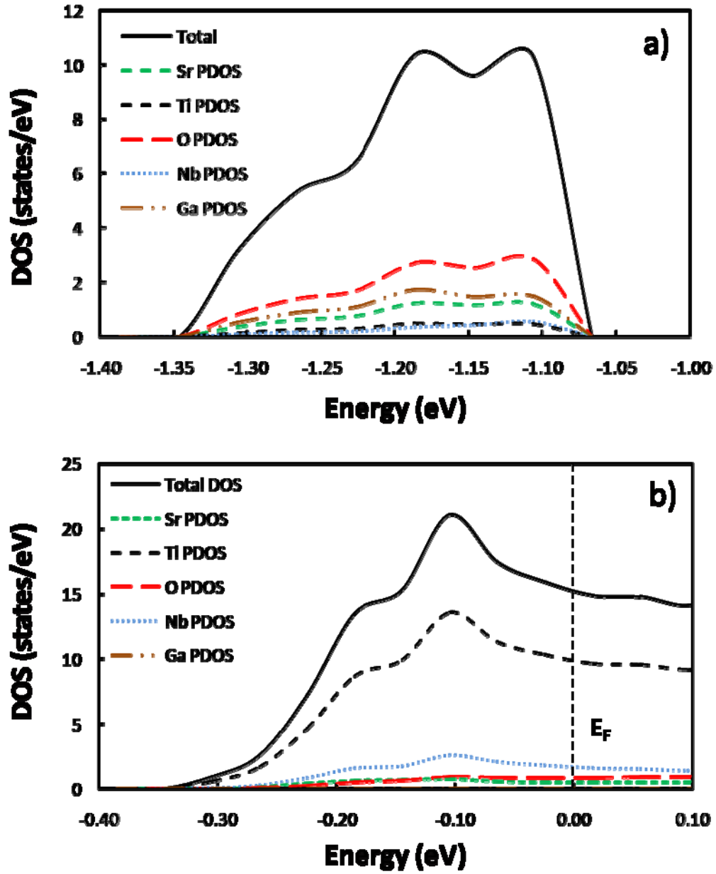
FIG. 7. (Color Online) Partial density of states (PDOS) of a) the gap states between the valence and conduction band and b) the states below the Fermi level in \text{SrTi}_{0.7}\text{Nb}_{0.2}\text{Ga}_{0.1}\text{O}_{2.9} .
