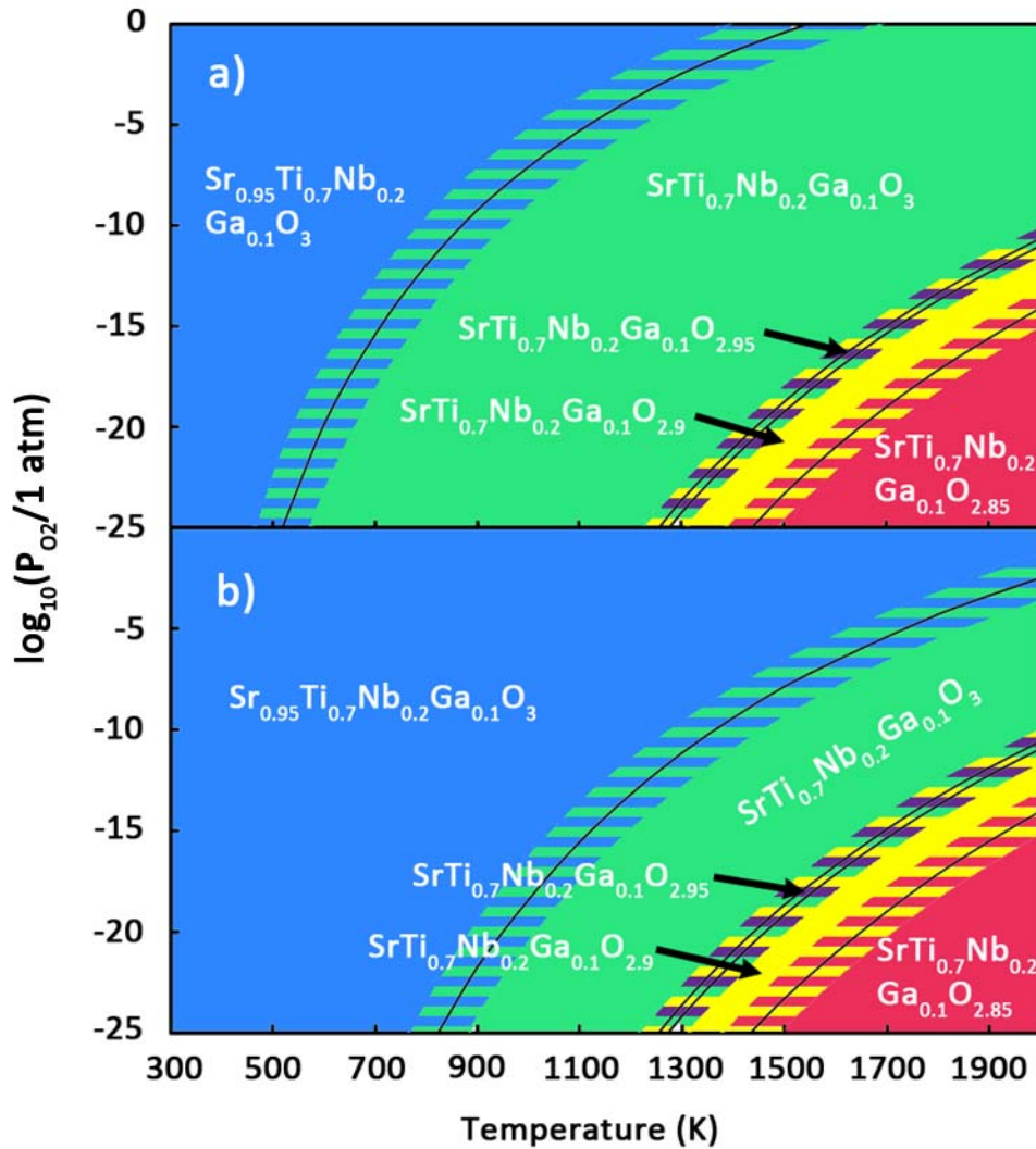
FIG. 5. (Color Online) Calculated phase diagram of 10% Ga- and 20% Nb-doped SrTiO 3 with a) SrO rich phase and b) TiO 2 /Ga 2 O 3 /niobium oxide rich phases. Differently shaded areas mark the stability regions of various structures for a given temperature and partial pressure of oxygen. The hatched area describes possible changes in the phase diagram if computed reaction energies shown in Table 1 are off by \pm 0.2 eV (our estimated error bar). Blue, green, yellow, and red areas symbolize stability of Sr 0.95 Ti 0.7 Nb 0.2 Ga 0.1 O 3 , SrTi 0.7 Nb 0.2 Ga 0.1 O 3 , SrTi 0.7 Nb 0.2 Ga 0.1 O 2.9 , and SrTi 0.7 Nb 0.2 Ga 0.1 O 2.85 , respectively. The hatched violet area symbolizes the possible stability of a SrTi 0.7 Nb 0.2 Ga 0.1 O 2.95 phase.
