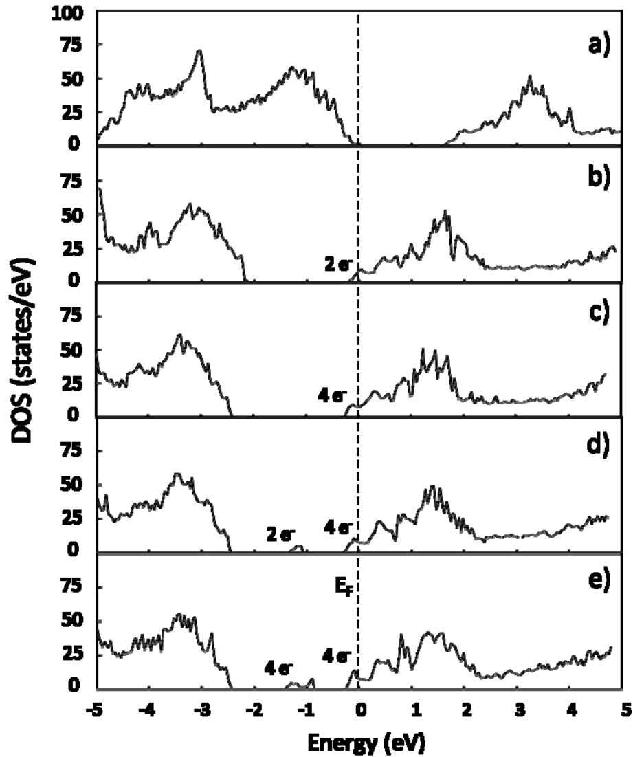
FIG. 6. Density of states of a) \text{Sr}_{0.95}\text{Ti}_{0.7}\text{Nb}_{0.2}\text{Ga}_{0.1}\text{O}_3 , b) \text{SrTi}_{0.7}\text{Nb}_{0.2}\text{Ga}_{0.1}\text{O}_3 , c) \text{SrTi}_{0.7}\text{Nb}_{0.2}\text{Ga}_{0.1}\text{O}_{2.95} , d) \text{SrTi}_{0.7}\text{Nb}_{0.2}\text{Ga}_{0.1}\text{O}_{2.9} and e) \text{SrTi}_{0.7}\text{Nb}_{0.2}\text{Ga}_{0.1}\text{O}_{2.85} . Fermi energy is set to zero on energy scale. Numbers of electrons shown in the figure indicate the integrated number of electrons per supercell for the specified DOS area, i.e., states in the band gap and states below the Fermi level.
