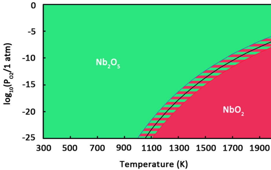
FIG. 2. (Color Online) Calculated phase diagram of \text{Nb}_2\text{O}_5/\text{NbO}_2 . Differently shaded areas mark the stability regions of various structures for a given temperature and partial pressure of oxygen. The hatched area describes possible changes in the phase diagram if computed reaction energies shown in Table 1 are off by \pm 0.2 eV (our estimated error bar). Green and red areas symbolize stability of \text{Nb}_2\text{O}_5 and \text{NbO}_2 , respectively.
