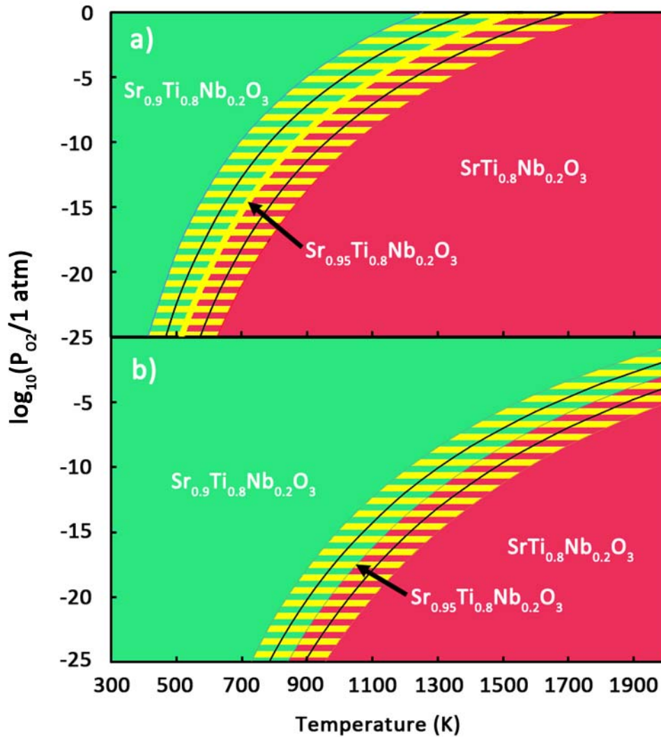
FIG. 3. (Color Online) Calculated phase diagram of 20% Nb-doped SrTiO 3 with a) SrO rich phase and b) TiO 2 /niobium oxide rich phases. Differently shaded areas mark the stability regions of various structures for a given temperature and partial pressure of oxygen. The hatched area describes possible changes in the phase diagram if computed reaction energies shown in Table 1 are off by \pm 0.2 eV (our estimated error bar). Green, yellow, and red areas symbolize stability of \text{Sr}_{0.9}\text{Ti}_{0.8}\text{Nb}_{0.2}\text{O}_3 , \text{Sr}_{0.95}\text{Ti}_{0.8}\text{Nb}_{0.2}\text{O}_3 , and \text{SrTi}_{0.8}\text{Nb}_{0.2}\text{O}_3 , respectively.
