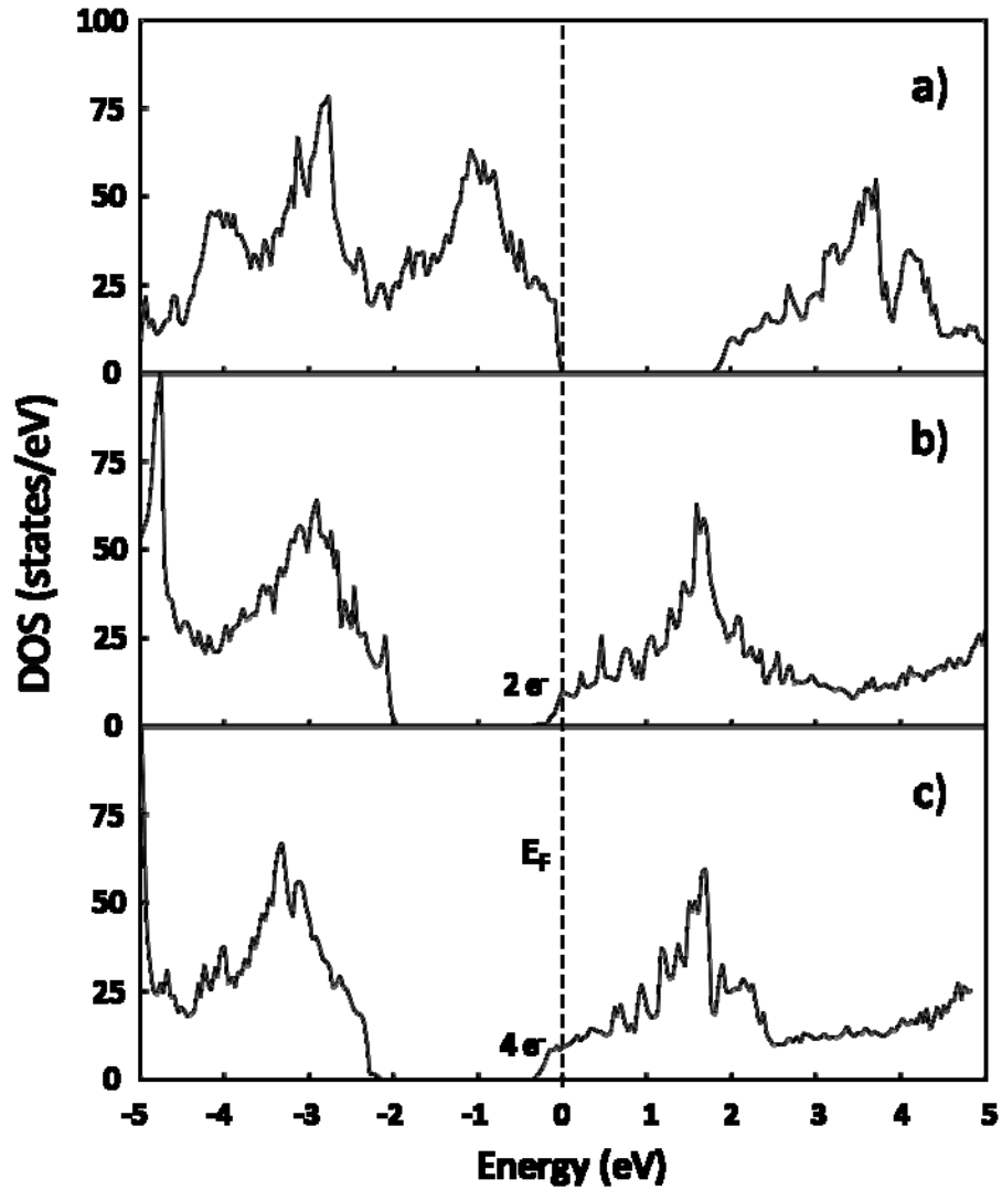
FIG. 4. Density of states of a) \text{Sr}_{0.9}\text{Ti}_{0.8}\text{Nb}_{0.2}\text{O}_3 , b) \text{Sr}_{0.95}\text{Ti}_{0.8}\text{Nb}_{0.2}\text{O}_3 and c) \text{SrTi}_{0.8}\text{Nb}_{0.2}\text{O}_3 . Fermi energy is set to zero on energy scale. Numbers of electrons shown in the figure indicate the integrated number of electrons per supercell for the specified DOS area, i.e., states in the band gap and states below the Fermi level.
