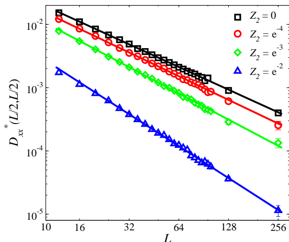
FIG. 13: (Color online) Dimer-dimer correlation function D_{xx}(r) for RVB systems in the W = (0, 0) sector with different fugacities Z_2 of long (fourth-neighbor) bonds (with the short-bond fugacity Z_1 = 1 ). The decay exponents grows with the long-bond fugacity. The values are given in Table I.
