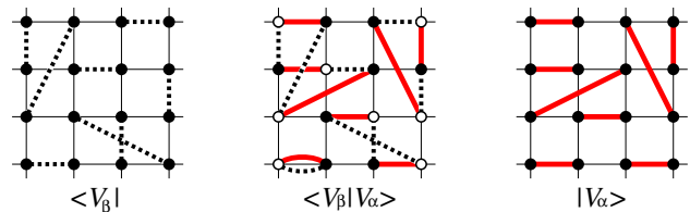
FIG. 3: (Color online) Two valence-bond states (left and right) in two dimensions and their transition graph formed by superimposing the two bond configurations (center). One of the spin configurations compatible with the transition graph is also shown, with open and solid circles for \uparrow and \downarrow spins. Each loop has two such allowed staggered spin configuration, and the overlap of two valence-bond states is thus \langle V_{\beta} | V_{\alpha} \rangle = 2^{n_{\alpha\beta} - N/2} , here with the number of loops n_{\alpha\beta} = 4 and the number of spins N = 16 .
