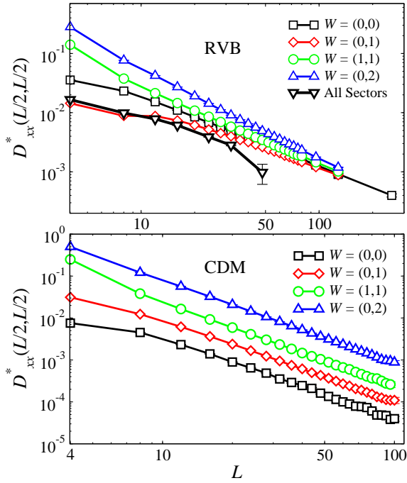
FIG. 7: (Color online) Dimer-dimer correlation function difference (4.1) at the maximal distance versus the lattice size. The upper panel shows results for the quantum RVB in different topological sectors as well as in the grand canonical ensemble (including all winding number sectors, in which case the fluctuations between sectors becomes very slow for large systems, as reflected in the large error bar for L = 48 ). All correlations converge to the same power-law decay as system size increases. The power, based on the W = (0,0) data for large L , is \alpha = -1.191(6) . The lower panel shows results for the CDM, which are consistent with \sim 1/r^2 (shown with the solid line) for all winding number sectors.
