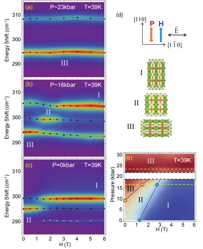
FIG. 13: Contour plots of the T_{2g} phonon mode intensities as functions of energy and applied field ( \mathbf{H}||[110] ) for T=39\text{K} and (a) P=23\text{kbar} , (b) P=16\text{kbar} , and (c) P=0\text{kbar} , where red=maximum counts and blue=0 counts. Filled diamonds represent the T_{2g} mode energies and the dashed lines are guides to the eye. (d) Illustrations of (I) the orthorhombic structure of \text{Mn}_3\text{O}_4 with magnetic easy axis along [110] , (II) the tetragonal structure of \text{Mn}_3\text{O}_4 , and (III) the orthorhombic structure of \text{Mn}_3\text{O}_4 with magnetic easy axis along [\bar{1}\bar{1}0] . (e) PH -phase diagram inferred from results in (a)-(c). Orange circles represent measured critical pressures between magnetostructural phase regions III (red) and II (gray), while blue circles represent measured critical pressures between magnetostructural phase regions II (gray) and I (blue). Dashed yellow lines indicate pressures at which magnetic field sweeps were obtained, and the white area is a region in which the detailed phase behavior is unknown.
