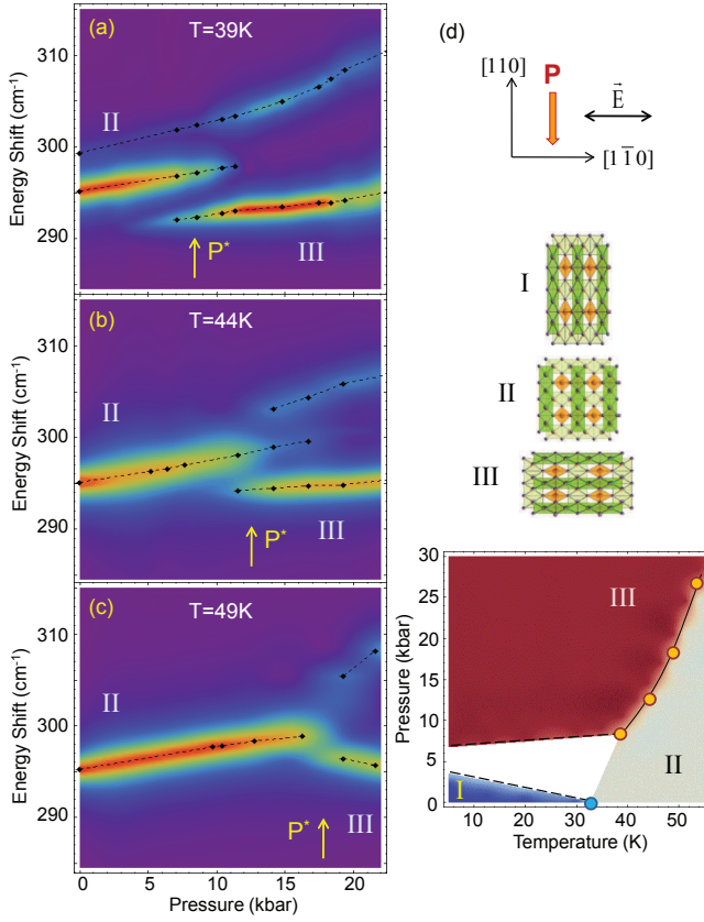
FIG. 12: Contour plots of the T_{2g} phonon mode intensities as functions of energy and applied pressure ( \mathbf{P}||[110] ) for H=0\text{T} and (a) T=39\text{K} , (b) T=44\text{K} , and (c) T=49\text{K} , where red=maximum counts and blue=0 counts. Filled diamonds represent the T_{2g} mode energies and the dashed lines are guides to the eye. (d) Illustrations of (I) the orthorhombic structure of \text{Mn}_3\text{O}_4 with magnetic easy axis along [110] , (II) the tetragonal structure of \text{Mn}_3\text{O}_4 , and (III) the orthorhombic structure of \text{Mn}_3\text{O}_4 with magnetic easy axis along [\bar{1}\bar{1}0] . (e) PT -phase diagram inferred from results in (a)-(c). The blue circle represents the measured critical temperature between magnetostructural phase regions I (blue) and II (gray), while the orange circles represent measured critical pressures between phase regions III (red) and II (gray). Dashed lines are estimated phase boundary lines, and the white area is a region in which the detailed phase behavior is unknown.
