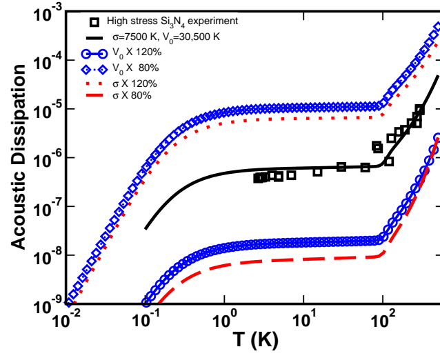
FIG. 7. (Color online) Acoustic dissipation Q^{-1} vs. temperature for various values of \sigma and V_0 . The black squares are the experimental data points for high stress \text{Si}_3\text{N}_4 from 4 . The black solid line shows the fit to the data. We have varied \sigma and V_0 by 20% above and below the fit values to show the sensitivity of the fit to the values of the parameters. The values of the other parameters are given in Table 1.
