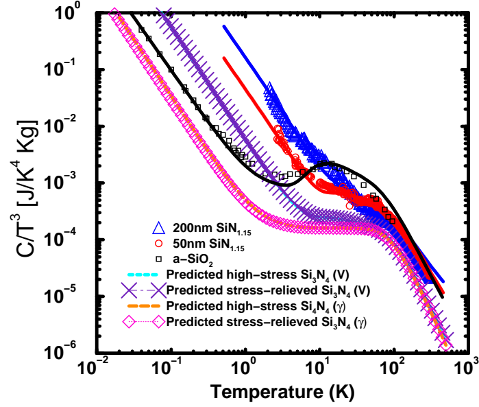
FIG. 1. (Color online) C(T)/T^3 vs. T for amorphous \text{SiO}_2 and silicon nitride. Experimental data points are shown for 50 nm and 200 nm thick \text{SiN}_{1.15} 25 and \text{SiO}_2 . The \text{SiO}_2 C(T) data are from 1,26 . The solid lines through the points are theoretical fits. Our predictions where stress affects V or \gamma are indicated in the legend by (V) and ( \gamma ), respectively. C(T)/T^3 curves for high stress and stress relieved \text{Si}_3\text{N}_4 lie on top of each other for the barrier height model. Similarly for the \gamma model.
