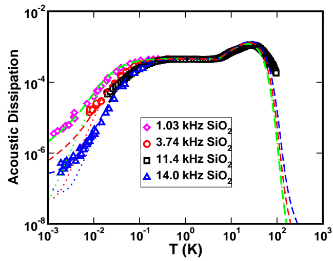
FIG. 4. (Color online) Acoustic dissipation Q^{-1} vs. temperature for \text{SiO}_2 at various frequencies. The data for \text{SiO}_2 at 11.4 kHz is from 17 while the rest of the \text{SiO}_2 data is from 23 . The fits to the \text{SiO}_2 data with the linear term bT are given by dashed lines while the fits without the linear term added are shown as dotted lines.
