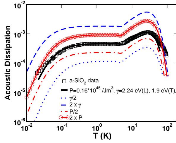
FIG. 5. (Color online) Acoustic dissipation Q^{-1} vs. temperature for various values of the deformation potential \gamma and the TLS density of states \bar{P} . The black squares are the \text{SiO}_2 data measured at 11.4 kHz from Tielburger et al. 17 . The black solid line is the fit using the values in Table 1 with \bar{P} = 0.16 \times 10^{45} / \text{Jm}^3 , longitudinal \gamma = 2.24 eV and transverse \gamma = 1.9 eV. The dotted blue line comes from using values of \gamma that are half as large while the dashed blue line comes from multiplying the values of \gamma by 2. The red dot-dashed line is the result of using a value of \bar{P} that is half as large, while the solid red line with open circles uses a value of \bar{P} that is twice as large.
