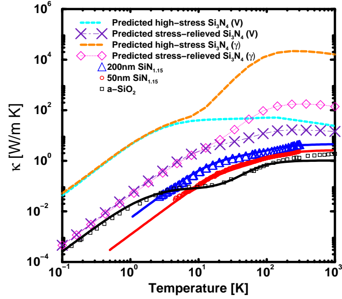
FIG. 2. (Color online) \kappa(T) vs. T for amorphous \text{SiO}_2 and silicon nitride. Experimental data points are shown for 50 nm and 200 nm thick \text{SiN}_{1.15} 25 and \text{SiO}_2 . The \text{SiO}_2 \kappa(T) data are from 27,28 . The solid lines through the points are theoretical fits. Our predictions where stress affects V or \gamma are indicated in the legend by (V) and (\gamma) , respectively. At low temperatures \kappa(T) for high stress \text{Si}_3\text{N}_4 is the same for the V and \gamma models. Similarly for stress relieved \text{Si}_3\text{N}_4 .
