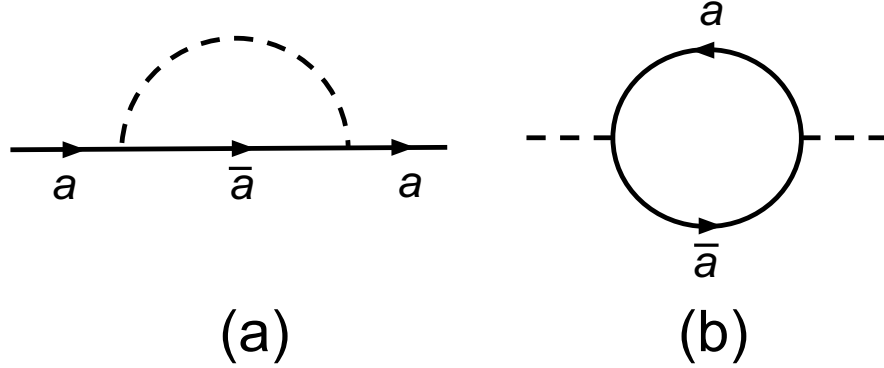
FIG. 3: (a) Fermion and (b) boson self-energies in the rainbow approximation. Solid lines are fermion Green's functions, while dashed lines are \phi Green's functions. All internal lines are full self-consistent propagators. In this section we are dropping the hot-spot index \ell , and so \psi_1 \equiv \psi_1^1 and \psi_{\bar{1}} \equiv \psi_2^1 .
