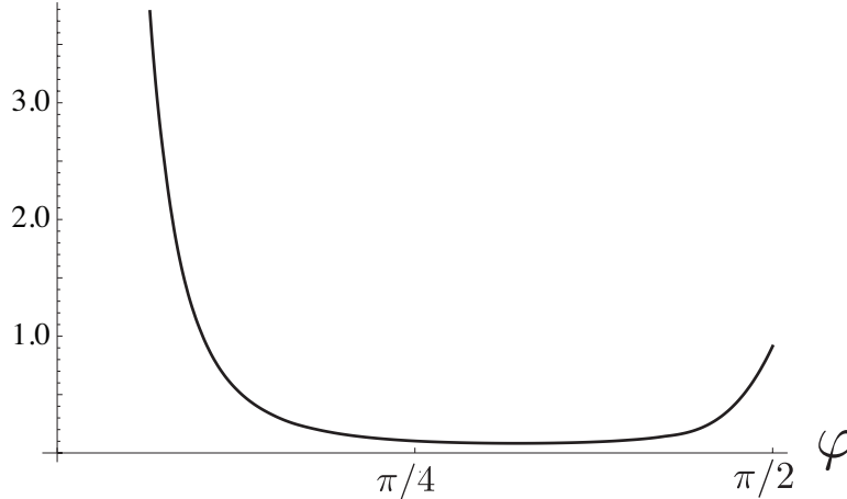
FIG. 8: The constant contribution to the conductivity as a function of the angle 2\varphi between the Fermi surfaces.
