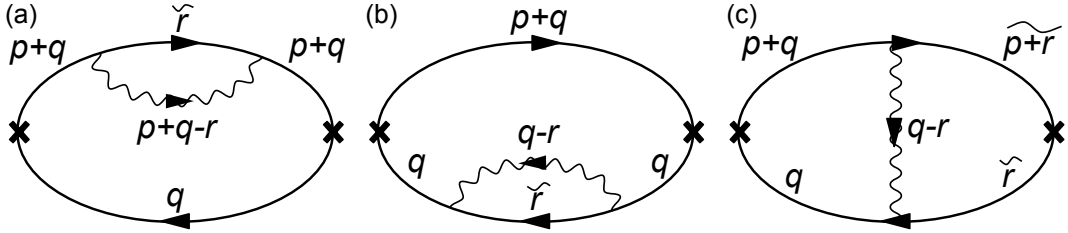
FIG. 14: The three leading order corrections in \lambda_3 to the conductivity due to cold fermions. Tildes over momenta indicate that the fermion propagator in question corresponds to the opposite patch. The hot operator \mathcal{O} is now complex and so its propagators carry an arrow.
