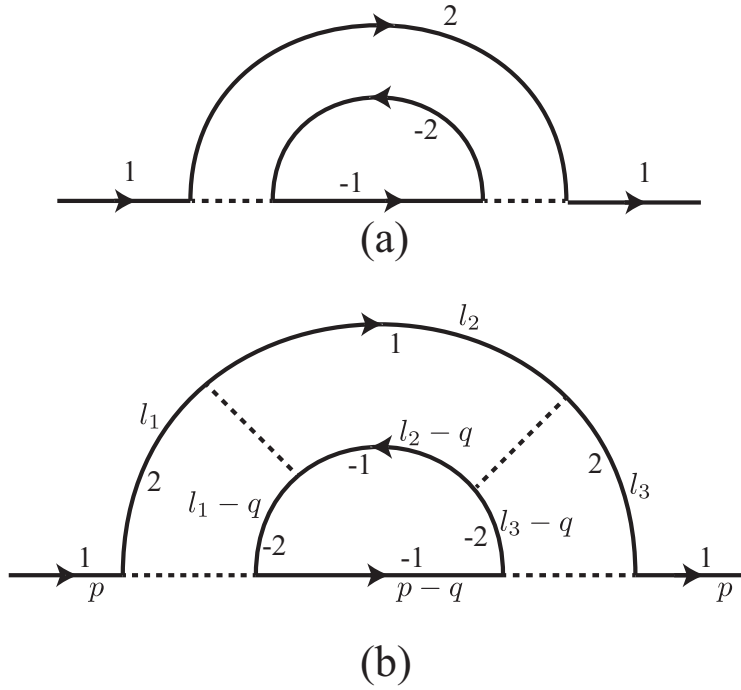
FIG. 17: Fermion self energy in the 2k_F channel. The scattering processes are those shown in Fig. 13; The 1 fermion refers to \psi_1^1 , the 2 to \psi_2^1 , the -1 to \psi_1^3 and the -2 to \psi_2^3 . These fermions are also referred to as \psi_1 , \psi_{\bar{1}} , \psi_{-1} , and \psi_{-\bar{1}} respectively. The momentum labels in (b) correspond to the expression in Eq. (D1).
