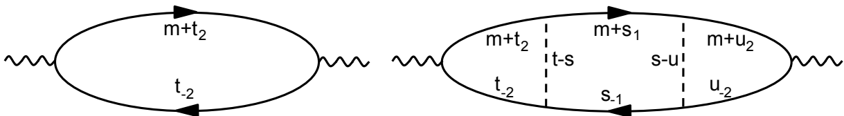
FIG. 19: Tree level (left) and leading correction (right) to the propagator for the operator \psi_2^{1\dagger}\psi_2^3 . The subscripts show the hot spot involved. 1 and -1 correspond to the a = 1 hot spots of the \ell = 1 and \ell = 3 pair of hot spots, respectively. Similarly, 2 and -2 correspond to the a = 2 hot spots of the \ell = 1 and \ell = 3 pair.
