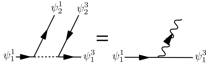
FIG. 12: Generating a local interaction of lukewarm fermions \psi = \psi_1^3 and \tilde{\psi} = \psi_1^1 with the operator \mathcal{O} = \psi_2^{\dagger}\psi_2^3 . The intermediate ‘fundamental’ boson on the left hand side is necessarily very off shell. Wavy lines are propagators for the operator \mathcal{O} , as in Fig. 9.
