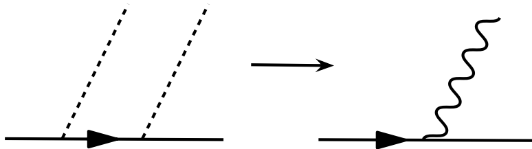
FIG. 9: Generating a local interaction between cold fermions and \mathcal{O} = \phi^2 . As in Fig. 4, a full line is a fundamental fermion \psi , and a dashed line is a ‘fundamental boson’ \phi . A wavy line represents a propagator for the operator \mathcal{O} . The intermediate fermion on the left hand graph is necessarily very off shell.
