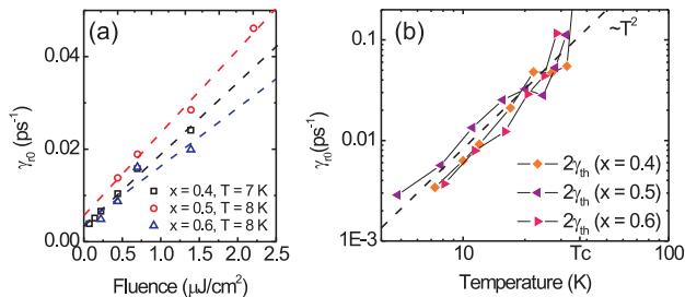
FIG. 5. Decay-rate analysis of data with a view towards gap symmetry. (a) The initial decay rate ( \gamma_{r0} ) as a function of pump fluence at 7, 8 K for x = 0.4 - 0.6 . The linear dependence of recombination rate on initial population is a hallmark of bimolecular recombination. Dashed lines show linear fits to data. The thermal decay rate at each temperature was obtained by extrapolating the fits to zero fluence. There is little significant difference between the various dopings. (b) The thermal relaxation rate \gamma_{th} plotted as a function of temperature for x = 0.4 - 0.6 . The dashed line shows \sim T^{-2} dependence as a guide along for all doping levels, suggesting a negligible change in Fermi surface topology between differently doped samples.
