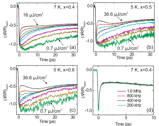
FIG. 2. Fast, intensity-dependent relaxation of the normalized reflectivity transients (\Delta R/R)_{norm} in the superconducting state. (a) The decay rate of (\Delta R(t)/R)_{norm} in the optimally doped compound ( x = 0.4 ) systematically decreases with decreasing intensity at 7 K (from bottom to top: \Phi = 0.7 \mu\text{J}/\text{cm}^2 (light green), 2.2, 4.4, 7.0, 8.9, 12.8 to 16.1 \mu\text{J}/\text{cm}^2 (black)). Raw traces from the overdoped hole-doped samples \text{Ba}_{1-x}\text{K}_x\text{Fe}_2\text{As}_2 for (b) x = 0.5 and (c) x = 0.6 at T = 5 K are qualitatively identical to those for the optimally doped sample in panel (a). In both of these plots, the absorbed fluences are, from bottom to top, \Phi = 0.7 \mu\text{J}/\text{cm}^2 (blue), 1.4, 2.2, 4.4, 7.0, 12.7, 20.1, and 36.6 \mu\text{J}/\text{cm}^2 (black). (d) (\Delta R/R)_{norm} measured at four different repetition rates are identical, verifying the absence of cumulative heating ( \Phi = 37 \mu\text{J}/\text{cm}^2 , T = 7 K).
