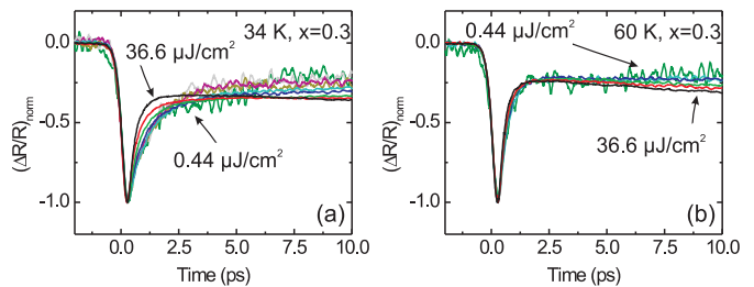
FIG. 10. Raw traces in the underdoped hole-doped pnictide \text{Ba}_{0.7}\text{K}_{0.3}\text{Fe}_2\text{As}_2 ( T_c = 32 K) above T_c . In (a), we note that there is some residual intensity dependence of the signal, where the initial recovery of the fast component is quicker at the highest fluences than at lower ones. This is identical to the superconducting state, despite the fact that at T = 34 K, the sample is in the normal state and the SDW state does not exhibit intensity dependent recombination (see below). After the initial electronic recovery, the amplitude of the acoustic wave is diminished at lower fluences. (b) In contrast, the fluence dependence of the electronic recovery has all but disappeared at 60 K. In both plots, the absorbed fluences are \Phi = 36.6, 20.1, 12.7, 7.0, 4.4, 2.2, 1.4, 0.7, and 0.44 \mu\text{J}/\text{cm}^2 .
