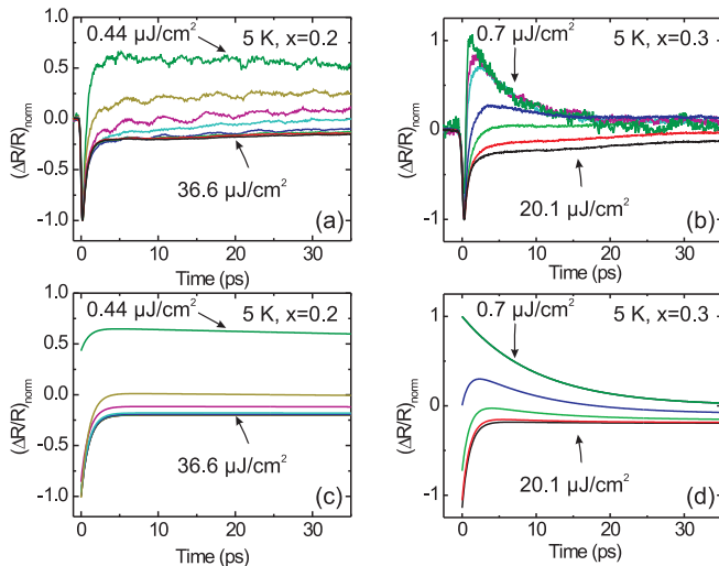
FIG. 8. Raw traces in the underdoped hole-doped samples \text{Ba}_{1-x}\text{K}_x\text{Fe}_2\text{As}_2 for (a) x = 0.2 ( T_c = 22 K, T_{SDW} \sim 100 K) and (b) x = 0.3 ( T_c = 22 K) at T = 5 K. The absorbed fluences are \Phi = 36.6 (black – (a) only), 20.1, 12.7, 7.0, 4.4, 2.2, 1.4, and 0.7 (blue) \mu\text{J}/\text{cm}^2 . Also shown are simulated results for \Delta R(t)/R at various values of \Phi using a simple two-component model in the (c) x = 0.2 sample and the (d) x = 0.3 sample at the same fluences. The simulations, which are performed without free parameters, show excellent qualitative agreement with the data.
