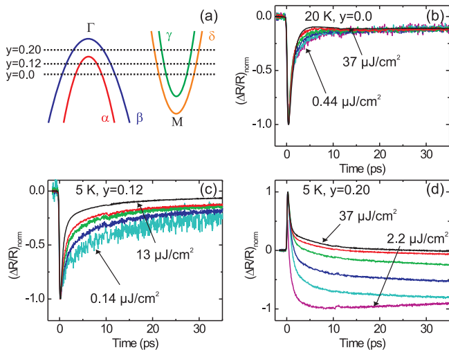
FIG. 11. (a) Schematic representation of the band structure of the Ba-122 pnictides. Although this is somewhat of a simplification that ignores the change in k_z dependence with doping 47 , the predominant effect is a shift of the Fermi level up with the addition of electrons 45 : in the parent compound, \alpha and \gamma, \delta nest, leading to SDW behavior. In the underdoped regime ( y = 0.12 ), \alpha does not nest appreciably with \gamma, \delta . With the addition of more holes, the \alpha band is submerged below the Fermi level when the doping reaches y = 0.15 , as measured by Sekiba et al. 46 (b) Raw (\Delta R/R)_{norm} traces for the parent compound at 20 K. The moderate amount of intensity dependence in these traces at short times is due to acoustic suppression from the diminished thermal expansion parameter at lower temperatures/fluences. (c) Reflectivity transients in the underdoped sample ( y = 0.12 , T_c = 12 K) show a mild amount of intensity dependence of the faster relaxation with increasing fluence, similar to that seen in the hole-doped samples. (d) Fluence dependence of the optimally doped sample ( y = 0.2 , T_c = 22.5 K) indicates entirely different relaxation dynamics with fluence. While there appears to be intensity dependence present here, the slope of the initial transient, \gamma_0 is identical for all fluences. The differences between the various fluences and the origin of this non-uniformity of the relaxation dynamics are due to a temperature effect, as described in the text.
