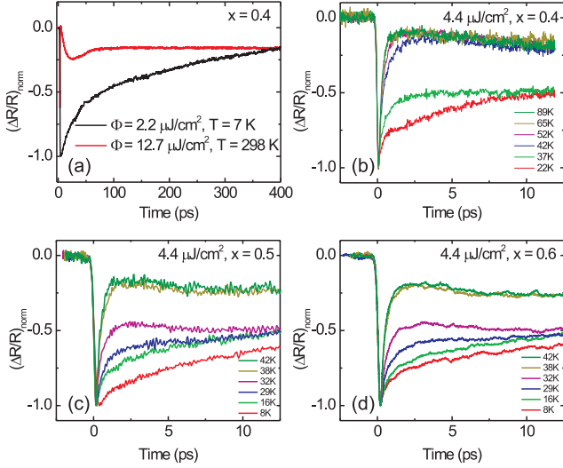
FIG. 3. Slow relaxation of (\Delta R/R)_{norm} in the superconducting state. (a) (\Delta R/R)_{norm} at 7 K and at room temperature. The slow, excitation density independent portion (black) switches off to become a nearly flat response in the normal state, which clearly shows the first oscillation due to stimulated Brillouin scattering. (b-d) A more complete view of the temperature dependence of (\Delta R/R)_{norm} near T_c obtained at \Phi = 4.4 \text{ J/cm}^2 in the x = 0.4 - 0.6 samples. We note a sharp decrease in the offset across the transition (i.e. 37 K to 42 K) due to switching off of the long-time component with loss of superconductivity. Above T_c there is an upturn of the signal evident at short times due to stimulated Brillouin scattering 39 .
