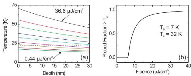
FIG. 9. (a) Simulated temperature profile as a function of depth for the fluences used in this study. The dotted lines indicate the values of transition temperature for the x = 0.2 ( T_c = 22 K) and the x = 0.3 ( T_c = 32 K) samples. (b) Fraction of the sample heated into the normal state as interrogated by the penetration depth of the probe for the x = 0.3 sample.
