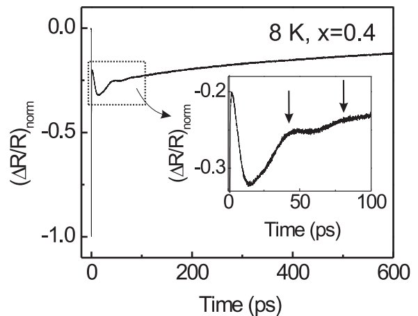
FIG. 7. Dynamics of the decay measured for a longer time window at T = 8 K and \Phi = 37 \mu\text{J}/\text{cm}^2 . Highly damped oscillations are observed with a period of \sim 40 ps (inset).
