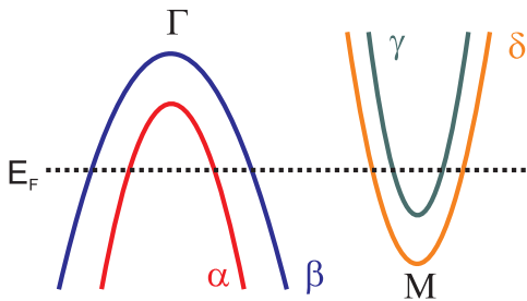
FIG. 6. Schematic representation of the pnictide band structure. While five bands have been observed by ARPES, the inner hole band is nearly doubly degenerate and so is represented by the single band \alpha .
