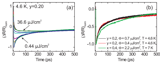
FIG. 12. Evolution of (\Delta R/R)_{\text{norm}} in \text{BaFe}_{1.8}\text{Co}_{0.2}\text{As}_2 for absorbed fluences of \Phi = 36.6 (black), 20.1, 12.7, 7.0, 4.4, 2.2, 1.4, 0.7, and 0.44 (blue) \mu\text{J}/\text{cm}^2 . As the fluence is increased, the recovery to equilibrium seems to slow due to a greater fraction of the probed sample being heated above T_c , especially at these long time scales. Proper scaling of the various traces yields a common, bottlenecked decay, reached by the sample when the entire probed region has cooled below T_c due to thermal diffusion. (b) Comparison of long-time traces of the optimally-doped hole-doped sample ( \text{Ba}_{0.6}\text{K}_{0.4}\text{Fe}_2\text{As}_2 ) and the optimally electron-doped ( \text{BaFe}_{1.8}\text{Co}_{0.2}\text{As}_2 ) material at fluences of 0.7 and 0.4 \mu\text{J}/\text{cm}^2 . Even though the Fermi surface topologies and gap energies of the two samples differ markedly, we note that the relaxation dynamics are nearly identical, indicating a common underlying relaxation mechanism, i.e., bottlenecked quasiparticle recombination in the outer hole band ( \beta ). This slow relaxation switches off at the respective values of T_c of both samples.
