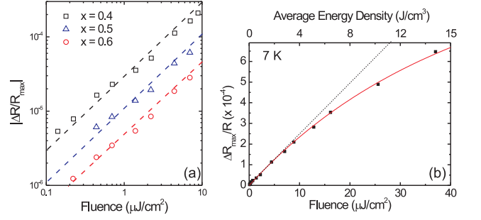
FIG. 4. (a) |(\Delta R/R)_{max}| plotted as a function of \Phi at T = 7 \text{ K} for the x = 0.4 - 0.6 samples, each offset for clarity. Dashed lines show a slope of one. Linear behavior in the low fluence regime is an indication that the optically accessed excitations are fully gapped, as described in the text. (b) The absolute value of the maximum change in reflectivity versus both \Phi and the average energy absorbed within a penetration depth for the x = 0.4 sample. The red curve is a fit to a simple saturation model yielding \Phi_{sat} = 25 \text{ } \mu\text{J/cm}^2 at an initial temperature of 7 K.
