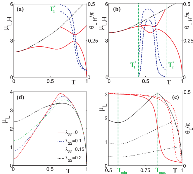
FIG. 1: Masses \mu_{L,H} of the composite gap function fields for (a) \gamma_F = 1 and \lambda_J = 0.005 , (b) \gamma_F = 0.5 and \lambda_J = 0.0025 . The position of branch cut is shown by black dashed line. The mixing angles \theta_{L,H} are shown by blue dashed and dash-dotted lines correspondingly. (c) Temperature dependence of the mass \mu_L(T) (black curves) and the corresponding mixing angle \theta_L determined by Eq.(11) (red curves) for \gamma_F = 1; 2; 5 (solid, dashed and dash-dotted curves). The coupling parameters are \lambda_{11} = 0.25 , \lambda_{22} = 0.213 and \lambda_J = 0.005 . (d) Temperature dependence of the mass \mu_L(T) for different values of coupling constant \lambda_{22} .
