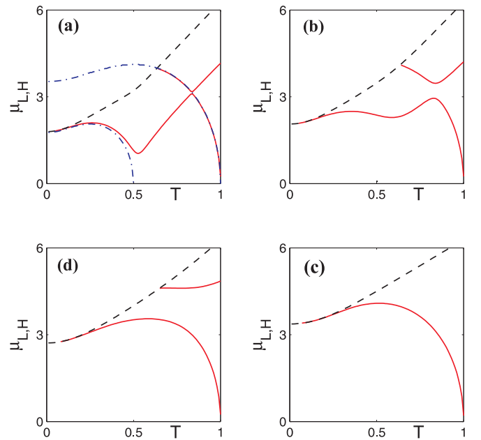
FIG. 2: Masses \mu_L and \mu_H (red solid lines) of the composite gap function fields for the different values of interband Josephson coupling \lambda_J and \gamma_F = 1 . In the sequence of plots (a)-(d) the transformation of masses is shown for \lambda_J decreasing from the small values \lambda_J \ll \lambda_{11}, \lambda_{22} to the values comparable to intraband coupling \lambda_J \sim \lambda_{11}, \lambda_{22} . The particular values of coupling constants are \lambda_{11} = 0.25 , \lambda_{22} = 0.213 and \lambda_J = 0.0005; 0.0025; 0.025 ; \lambda_{22} for plots (a-d) correspondingly. By black dash-dotted lines the branch cuts are shown. In (a) with blue dash-dotted lines the masses of modes are shown for the case of \lambda_J = 0 . Note that at \lambda_J = 0 the two masses go to zero at two different temperatures. Because 1/\mu_{L,H} are related to the coherence length, this reflects the fact that for U(1) \times U(1) theory there are two independently diverging coherence lengths. Note that for finite values of interband coupling only one mass \mu_L goes to zero at one T_c .
