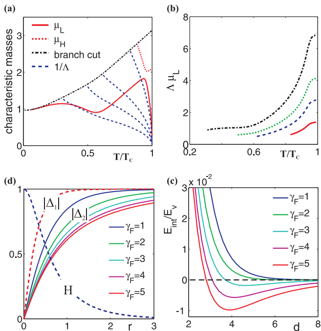
FIG. 3: (a) Masses \mu_L and \mu_H (red solid and dotted lines) of the composite gap function fields and inverse London penetration (blue dashed lines) for the different values of \Lambda \mu_L(T_c)/\sqrt{2} = 1; 2; 3; 5 . The position of branch cut is shown by black dash-dotted line. (b) The temperature dependence of the quantity \Lambda \mu_L for \Lambda \mu_L(T_c)/\sqrt{2} = 1; 2; 3; 5 (red solid, blue dashed and black dash-dotted lines). (c) Distributions of magnetic field H(r)/H(r=0) , gap functions |\Delta_1|(r)/\Delta_{10} (dashed lines) and |\Delta_2|(r)/\Delta_{20} (solid lines) for the coupling parameters \lambda_{11} = 0.25 , \lambda_{22} = 0.213 and \lambda_{21} = 0.0025 and different values of the band parameter \gamma_F = 1; 2; 3; 4; 5 . (d) The energy of interaction between two vortices normalized to the single vortex energy as function of the intervortex distance d . In panels (c,d) the temperature is T = 0.6 .
