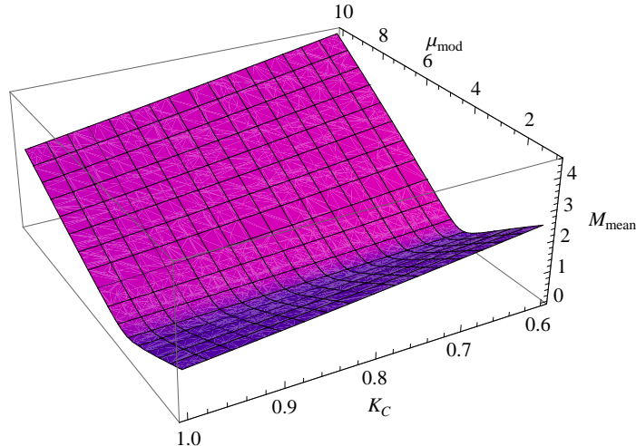
FIG. 6: (Color online) The mean-field value of \bar{M}_{\text{mean}} [meV] of the single-particle gap as a function of the parameters K_c and \mu_{\text{mod}} in the range 0.6 \leq K_c \leq 1.0 , for K_s = 1.1 and with \lambda_R = -2 meV, \nu = 0.04 , \Lambda = 100 meV, and 1 \text{ meV} \leq \mu_{\text{mod}} \leq 10 meV.
