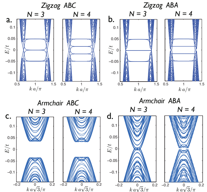
FIG. 2: Band structures of ABC and ABA stacked zigzag and armchair terminated trilayer and tetralayer ribbons in the presence of a uniform electric field. (a) ABC stacked layers with zigzag edges; (b) ABA stacked layers with zigzag edges; (c) ABC stacked layers with armchair edges and (d) ABA stacked layers with armchair edges. In each subfigure, the left and right panels represent trilayer and tetralayer ribbons, respectively. For ABC stacking the electric field opens a bulk band gap containing edge states in the zigzag case but not in the armchair case. The number of edge state branches is independent of the ribbon width, whereas the number of bulk state branches is proportional to ribbon width. In the case of ABA stacking, ribbons are metallic in the trilayer whereas a small gap opens in the tetralayer geometry.
