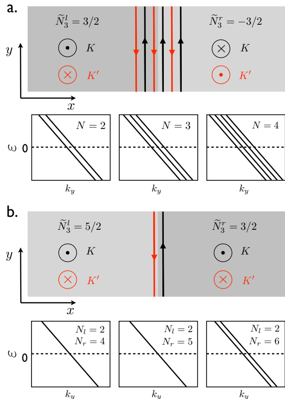
FIG. 1: Schematic illustration of the relationship between valley Hall effects and 1D conduction channels at interfaces expected on the basis of continuum model considerations. The number of 1D modes per valley is an integer n evaluated from differences between valley Chern numbers n = \left| \tilde{N}_3^l - \tilde{N}_3^r \right| . When the layer number N is odd, the integral of the Berry curvatures is half-odd-integer, a property that is related to the half-quantized Hall effect of Dirac systems. We find that the number of 1D channels is then usually reduced to the integer part of the integrated Berry curvature difference. The sense of the arrows directed perpendicular to the page indicates the sign of the Chern number associated with each valley. Upper panel: Illustration of ABC trilayer graphene with opposite electric field signs in left and right regions with three 1D modes per valley. Lower panel: Junction formed between pentalayer and trilayer regions under a uniform bias potential. In this case the valley Hall conductivities have the same sign but different magnitude on opposite sides of the interface and the number of 1D channels is expected to be proportional to the difference of the individual Berry curvature integrals. The continuum model picture illustrated here can be invalidated by atomic scale physics at the interface, particularly when the number of layers on opposite sides of the interface is different.
