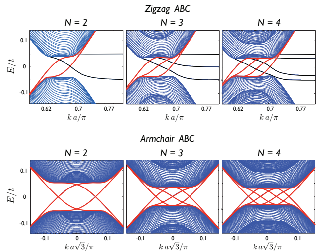
FIG. 3: (Color online) Upper Panel : Band structure of bilayer, trilayer and tetralayer graphene zigzag ribbons with an electric field sign change at the ribbon center. We can clearly observe two, three and four 1D valley Hall kink states with a common sign of velocity located around the valley point. The branches which correspond to wavefunctions localized at the ribbon center are plotted in red. The other branches that cross the bulk gap are doubly-degenerate edge states. Lower Panel : Band structure of bilayer, trilayer and tetralayer graphene armchair ribbons with an electric field sign change at the ribbon center. As in the zigzag case we can clearly identify two, three and four three 1D kink state branches. In armchair edges we do not find 1D edge state channels.
