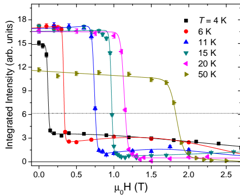
FIG. 3: (color online) Integrated intensity of the (1 0 0) peak as a function field. The data were taken while increasing field. Lines are a guide to the eye. The dotted horizontal line represents the expected intensity at 2 K in zero field.
