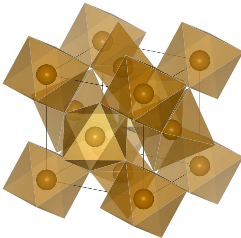
FIG. 1. (Color online) Unit cell of pyrite \text{FeS}_2 . The spheres at fcc sites are Fe atoms. Each Fe atom sits in a slightly distorted octahedral environment of S atoms, which are located at the octahedral vertices.
