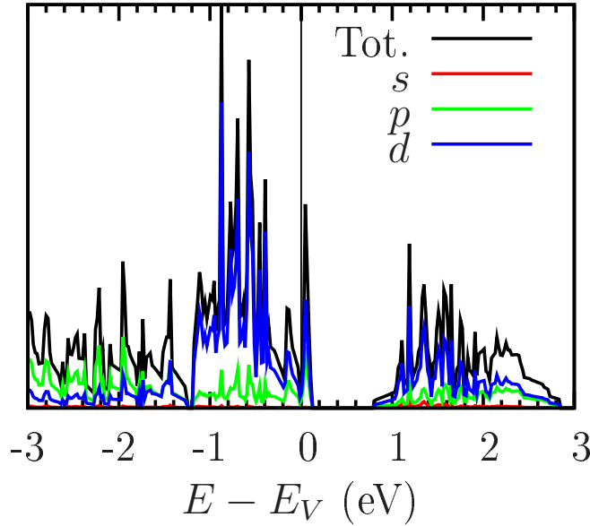
FIG. 18. DOS of pyrite (100) with Cl-adsorbates. The intrinsic surface state at the CB edge in Fig. 9(b) is depleted due to surface passivation.
