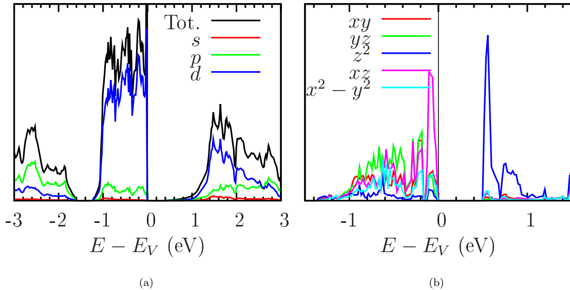
FIG. 9. (Color online) GGA-PBE DOS of pyrite (a) bulk; (b) (001) surface. In (a), both the total DOS and s - p - d decomposed DOS are shown. The CB and VB are dominated by Fe d states. We have verified that these d states within the CB and VB are e_g and t_{2g} , respectively. Due to the presence of a S p state, the CB tail extends to 0.4 eV above the VB edge. In (b), the DOS of d -orbitals are shown to identify the character of intrinsic surface states. The intrinsic surface state appears at the CB edge, not within the band gap, and is characterized to be of d_{z^2} character. However, ligand field splitting in the VB is not observed and d_{xy} surface states are not found, contrary to the prediction of Bronold and coworkers. 5
