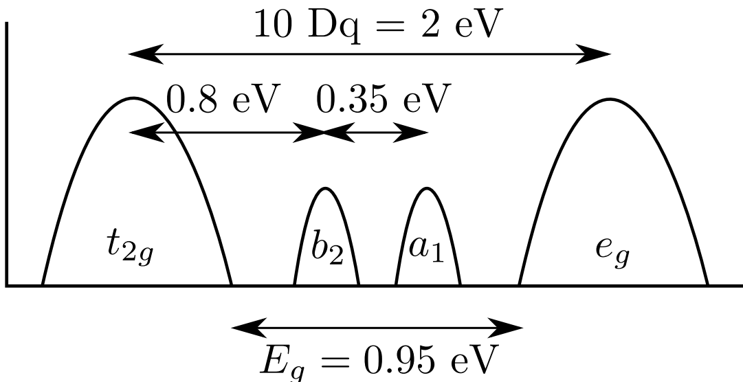
FIG. 4. Schematic of the ligand field model developed by Bronold et al. 5 The CB and VB are dominated by e_g and t_{2g} states, respectively. As a result of symmetry reduction, a_1 and b_2 states, which correspond to d_{z^2} and d_{xy} states, are introduced within the band gap.
