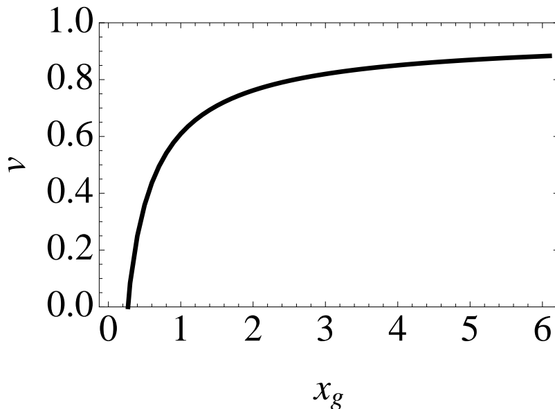
FIG. 19. Voltage ratio ( v = qV_{oc}/E_g ) as a function of x_g = E_g/kT_s \approx 1.93E_g , where T_s = 6000 K is the temperature of the sun, predicted by Shockley-Queisser theory. 60
