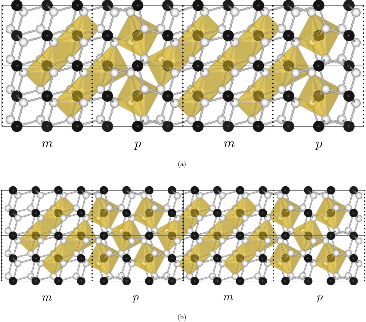
FIG. 12. (Color online) Structures of the pyrite (001)-marcasite (101) interface for \theta = 270^\circ and (a) N = 3 ; (b) N = 4 . Black (white) spheres are Fe (S) atoms. Pyrite and marcasite phases are labeled by p and m , respectively, where the interfaces are marked by vertical dotted lines. For clarity, the supercell (enclosed in black rectangle) is repeated along the [010] (downward) and [001] (rightward) directions, and octahedra are drawn for Fe atoms in the inner-most layer only. Note the octahedra are edge-sharing in bulk marcasite but corner-sharing in bulk pyrite. At the interface, the octahedra are edge-sharing when N is odd (a), but can be corner-sharing when N is even (from left to right, the second dotted line in (b)), showing that different interfacial energies may result depending on the parity of N . Consecutive 90^\circ rotations of one phase with respect to the other about the rightward axis can create more variations (not shown). It is verified that the corner-sharing type interface with \theta = 270^\circ is the most energetically favorable.
