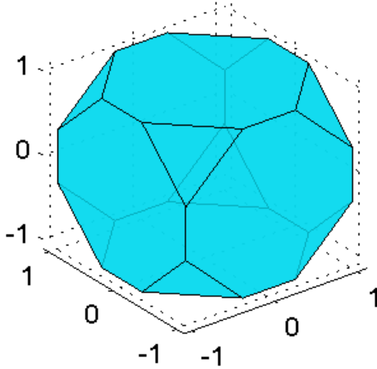
FIG. 8. (Color online) Wulff shape of pyrite within GGA-PBE. Surface energies are taken from Table I. The dominant surface is \{100\} . \{111\} facets are also observed. The equilibrium shape is cubo-octahedral.
