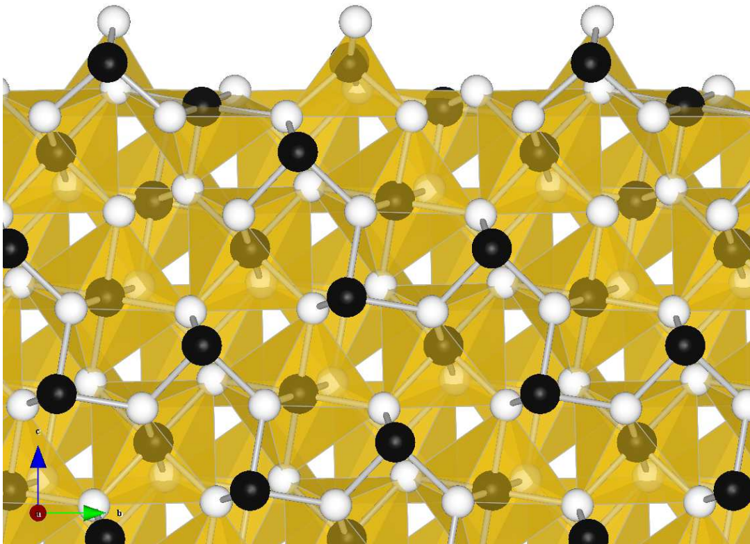
FIG. 7. (Color online) Side view of pyrite (210) surface. Black (white) spheres are Fe (S) atoms. The surface is non-polar and S-terminated.
