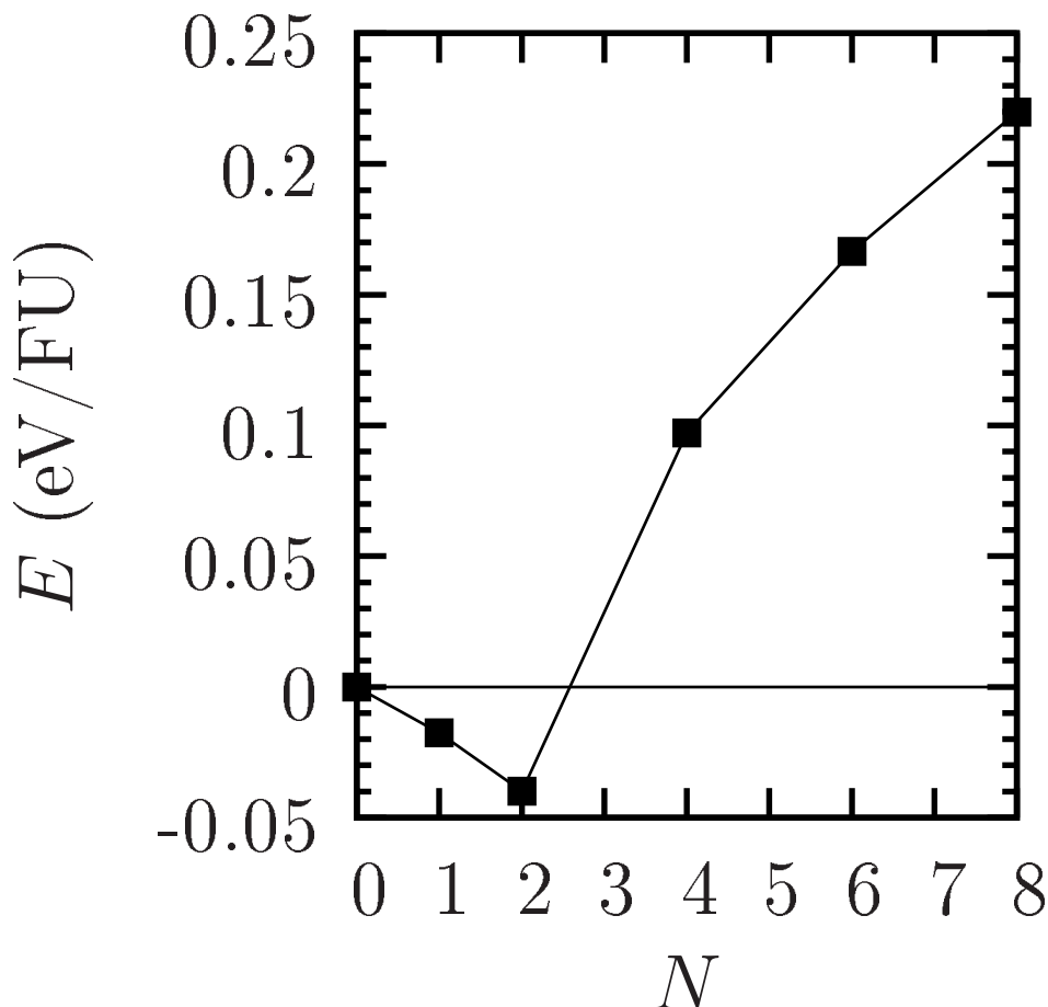
FIG. 14. Total energy (per formula unit) of pyrite (100)-marcasite (101)-vacuum supercell as a function of the number of epitaxial layers of marcasite, N . The total energies are referenced to a clean pyrite (100) surface ( N = 0 ). The global minimum is obtained when N = 2 .
