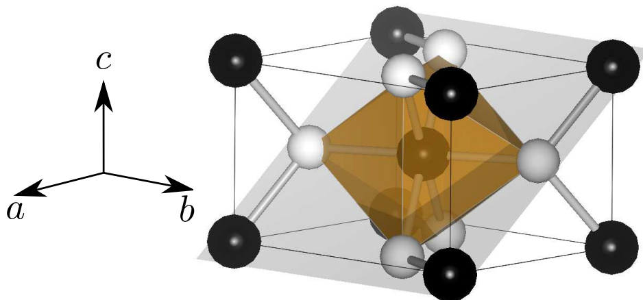
FIG. 2. Unit cell of marcasite \text{FeS}_2 . Black (white) spheres represent Fe (S) atoms. The (101) plane is highlighted in grey. The octahedra is edge-shared by the S atoms on the (001) faces.
