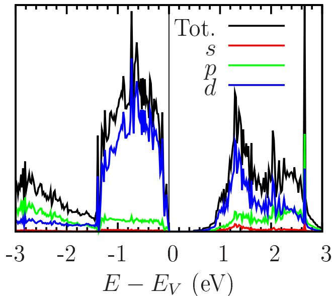
FIG. 17. (Color online) DOS of the lowest energy pyrite(001)-marcasite(101) interface (corner-sharing, \theta = 270^\circ ) within GGA-PBE. By comparing to Fig. 9, two key observations are made: (i) the band gap is not reduced; (ii) gap states are not found.
