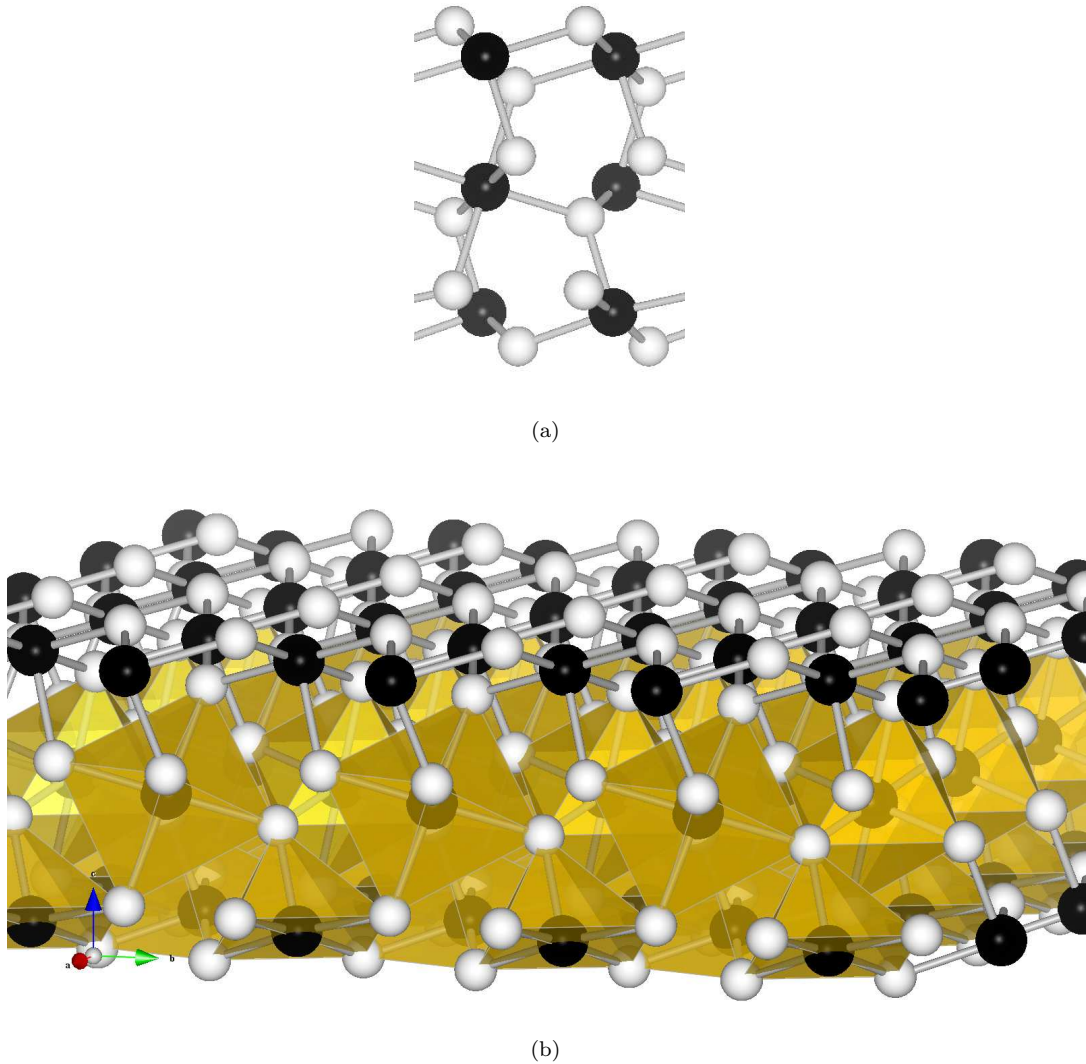
FIG. 3. (Color online) (a) Side view of the unique, non-polar pyrite (100) surface. Looking along the surface normal direction (upwards), the atomic layers have the repetitive pattern [S–Fe–S]. Other possible terminations result in repeating layers of [S–S–Fe] or [Fe–S–S]. In both cases, polar surfaces result. Hence, this S-terminated surface is the only possible non-polar (100) surface. In (b), note the octahedral environment around bulk Fe atoms, and the square pyramidal environment around surface Fe atoms. Polyhedra are not shown in the top-most layer. Black (white) spheres are Fe (S) atoms.
