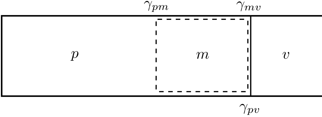
FIG. 11. Schematic of marcasite overgrowth on pyrite. Pyrite, marcasite, and vacuum are labeled as p , m , and v , respectively. By growing marcasite (enclosed in dashed region), the top bulk layers of pyrite are replaced, resulting in a difference in bulk energy \Delta g . Moreover, the pyrite (001) surface energy \gamma_{pv} is replaced with the marcasite (101) surface energy \gamma_{mv} plus an interfacial energy between the two phases \gamma_{pm} .
