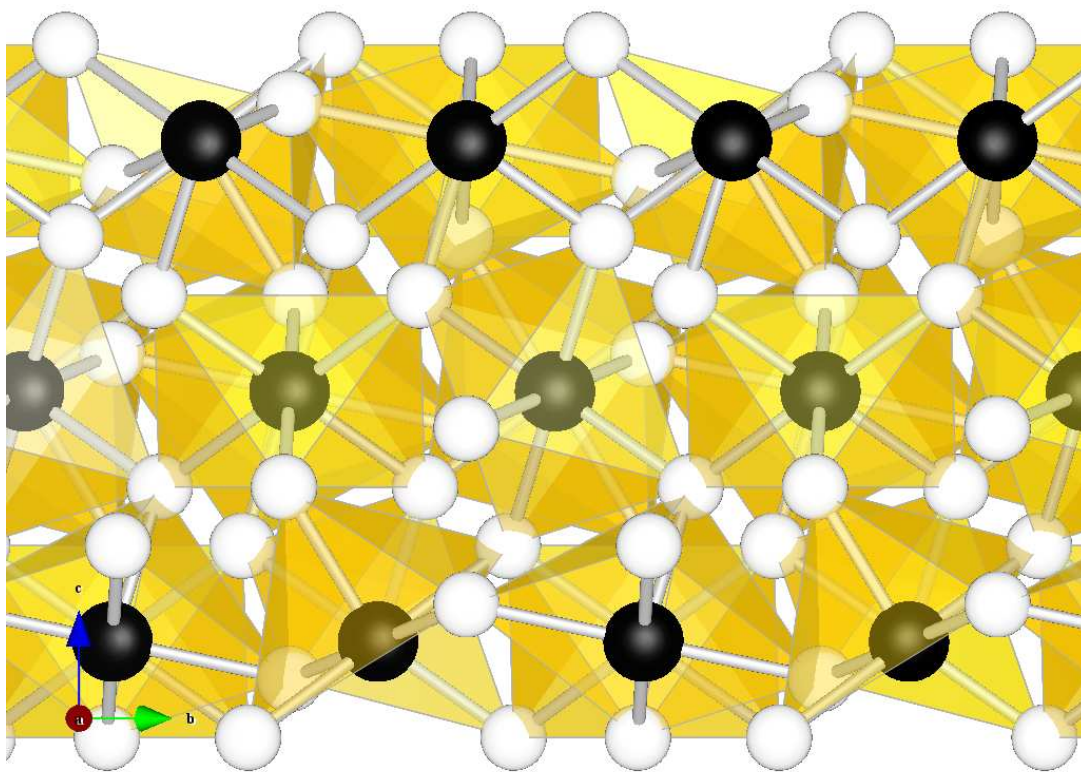
FIG. 6. (Color online) Side view of pyrite (111) surface. Black (white) spheres are Fe (S) atoms. The surface is non-polar and S-terminated.
