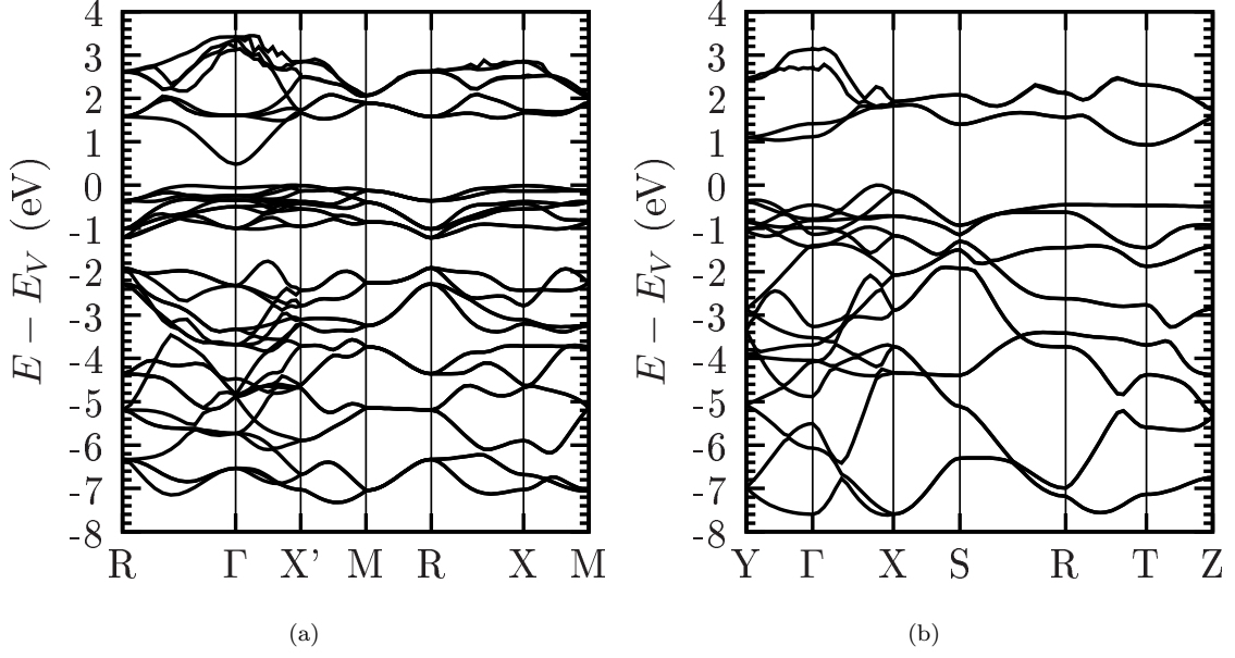
FIG. 15. PBE band structure of (a) pyrite and (b) marcasite. Both of them are indirect gap materials. High symmetry points correspond to those in Ref. 27. The LDA and AM05 band structures look very similar and are not shown.
