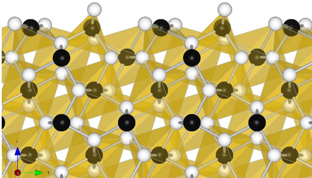
FIG. 5. (Color online) Side view of pyrite (110) surface. Black (white) spheres are Fe (S) atoms. The surface is non-polar and S-terminated.
