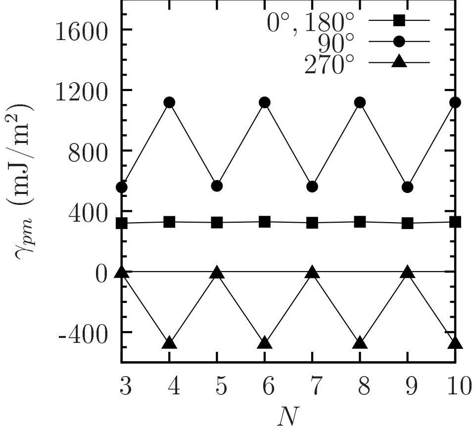
FIG. 13. The pyrite(001)–marcasite(101) interfacial energy, \gamma_{pm} , within GGA-PBE. The interfacial energy depends on the relative orientation between the two phases and the parity of N .
