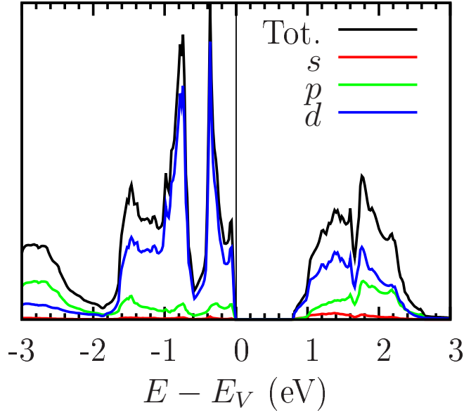
FIG. 16. (Color online) DOS of bulk marcasite within GGA-PBE. Contrary to pyrite, there are no pronounced tail states at the CB in marcasite.
