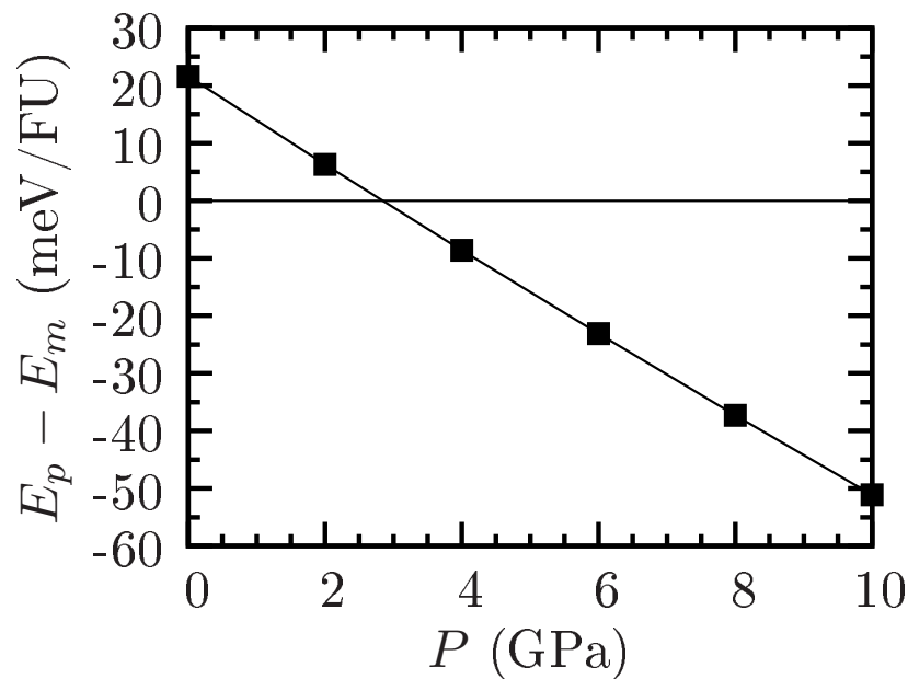
FIG. 20. Relative stability of pyrite and marcasite as a function of applied pressure within GGA-PBE. The cross-over occurs at 2.8 GPa. To reach the same relative stability predicted by LDA and AM05 ( E_p - E_m = -8.6 meV/FU), a pressure of 4 GPa is needed.
