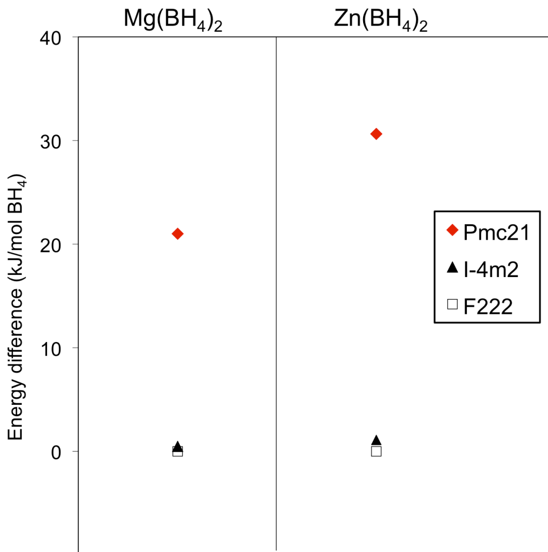
Fig. 3. DFT energies for three different crystal structures ( Pmc2_1 , I\bar{4}m2 and F222 ) for Mg(BH_4)_2 and Zn(BH_4)_2 . For both materials, Pmc2_1 has higher energy, whereas, I\bar{4}m2 and F222 are the low energy structures and are nearly degenerate. Energies are in units of kJ/mol BH_4 and are given relative to that of the lowest-energy F222 structure.
