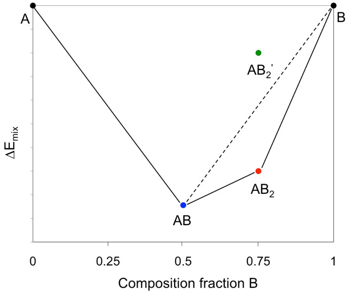
Fig. 1 Phase stability of two compounds A and B. Points AB and AB_2 represent mixing energy of A and B in 1:1 and 1:2 composition respectively. A convex hull passing through A, AB, AB_2 and B represents the stability of phases AB and AB_2 . In case mixing energy of phase AB_2 is represented by AB'_2 , which lies above the convex hull formed between A, AB and B, then the phase AB'_2 is unstable with respect to AB and B.
