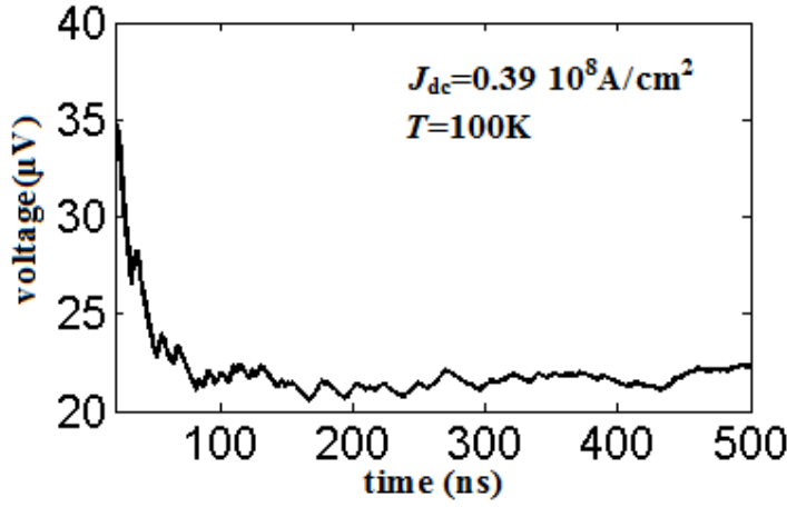
FIG. 6: Time evolution of dc voltage computed for J_{dc}=0.39\times 10^8\text{A/cm}^2 , T=100\text{K} , J_M=0.1\times 10^8\text{A/cm}^2 and f_{AC}=2.50\text{GHz} .
