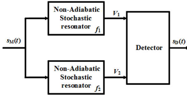
FIG. 8: A simplified schematic block diagram of a receiver for frequency-shift keying (FSK) modulation based on non-adiabatic stochastic resonance phenomenon.
