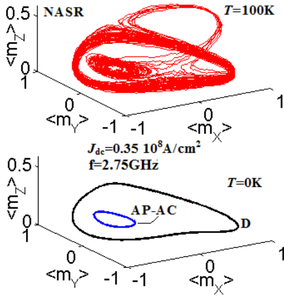
FIG. 7: (Color online)(a) Trajectory of the average magnetization vector at the non-adiabatic stochastic resonance (NASR) for J_{dc}=0.35\times 10^8\text{A/cm}^2 , T=100\text{K} , J_M=0.1\times 10^8\text{A/cm}^2 and f_{AC}=2.75\text{GHz} . (b) Zero-temperature magnetization trajectories in the D and the AP (AP-AC) states for the drive frequency of f_{AC}=2.75\text{GHz} .
