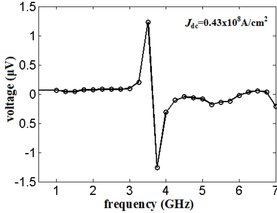
FIG. 2: Direct voltage as a function of frequency of the ac current in the D state calculated for J_{dc}=0.43\times 10^8 A/cm 2 and J_M= 0.1\times 10^8 A/cm 2 .
