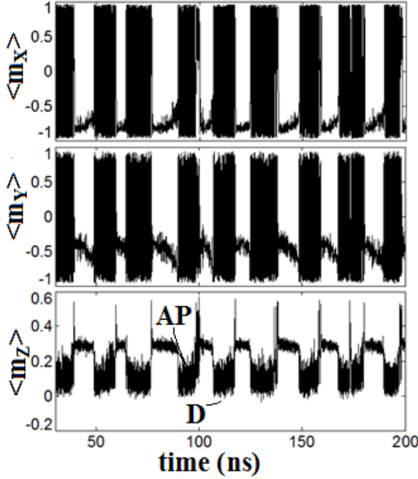
FIG. 4: Example of time traces (x, y and z average component of the magnetization) corresponding to ASR ( J_{dc}=0.43\times 10^8 A/cm 2 , T=100 K, J_M=0.1\times 10^8 A/cm 2 and f_{AC}=50 MHz).
