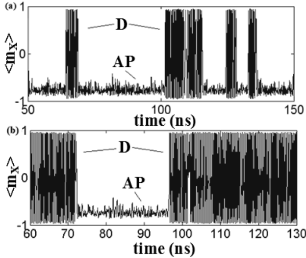
FIG. 3: Time traces of the normalized average x-component of the magnetization for (a) J_{dc} = 0.38 \times 10^8 \text{ A/cm}^2 at 150 K and (b) J_{dc} = 0.46 \times 10^8 \text{ A/cm}^2 at 100 K.
