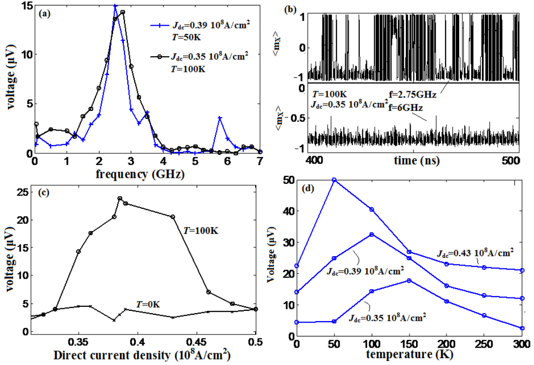
FIG. 5: (Color online) (a) Dc voltage as function of frequency of the applied alternating current calculated for two direct current densities and temperatures, J_{dc} = 0.35 \times 10^8 \text{ A/cm}^2 ( T = 100 \text{ K} ) and J_{dc} = 0.39 \times 10^8 \text{ A/cm}^2 ( T = 50 \text{ K} ); (b) time traces of the average x-component of the magnetization for J_{dc} = 0.35 \times 10^8 \text{ A/cm}^2 ( T = 100 \text{ K} ) at two different ac current frequencies, f_{AC} = 2.75 \text{ GHz} (top) and f_{AC} = 6 \text{ GHz} (bottom); (c) V_{\text{DC-max}} as function of the direct current density calculated at T = 100 \text{ K} and T = 0 \text{ K} ; (d) Temperature dependence of V_{\text{DC-max}} for three direct current densities, J_{dc} = 0.35, 0.39, and 0.43 \times 10^8 \text{ A/cm}^2 (the curves are vertically offset by 10 \mu\text{V} for clarity).
