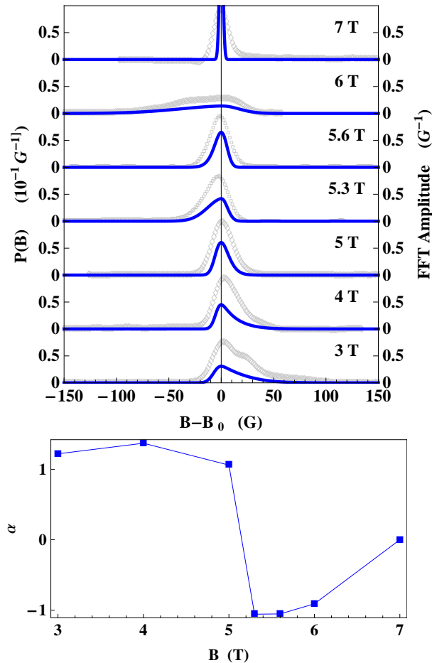
FIG. 2: (color online) (upper panel) Probability field-distribution lines, P(B) , for \text{LuNi}_2\text{B}_2\text{C} (solid lines) at different external magnetic fields, derived by deconvoluting the FFTs (open symbols) of the \mu\text{SR} signals. Measurements at H = 3, 4, 5 , and 6 T were done after field-cooling to 2.3 K at 3 T, whereas at H = 5.3 and 5.6 T were performed after degaussing at 2.7 K. The lines were displaced vertically for clarity and horizontally for comparison. The reference data used in the deconvolution were measured on the same sample above T_c at T = 20 K. The shoulder seen on the 3 T FFT curve around 25 G is due to muons which missed the SC sample. (lower panel) Field-dependence of the skewness parameter, \alpha (see text), as calculated from the field distributions shown in the upper panel. The line connecting the data points is a guide to the eyes.
