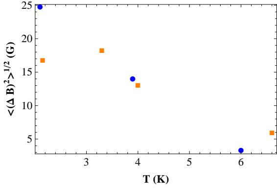
FIG. 5: (color online) Temperature dependence of the field distribution width, measured after 3T (orange squares) and 0.5T (blue circles) cooldowns. For each cooldown, the measurements were done at a certain field, 4.5T for the 0.5T cooldown, and 3T for the 3T cooldown.
