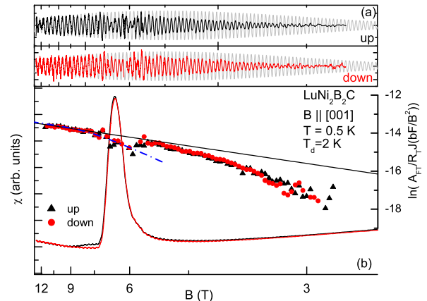
FIG. 1: (color online) (a) dHvA oscillation signals, for upward and downward field-sweeps respectively, measured on \text{LuNi}_2\text{B}_2\text{C} after background subtraction, and (b) the corresponding Dingle plots (triangles and circles respectively). The gray oscillatory lines in (a) represent the extrapolated dHvA signal, based on the normal state Lifshitz-Kosevich formula, whereas the solid straight line in (b) is the corresponding Dingle plot. The total magnetization for both field-sweeps (solid curves) are also shown in (b). The dash-dotted line in (b) represents the result of a calculation based on the random vortex distribution model with the zero field order parameter \Delta_0 = 4\text{ meV} and mean-field H_{c2} = 8\text{ T} . Measurements were done at 0.5 K.
