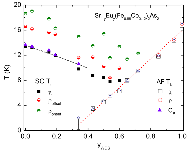
FIG. 12: T-y phase diagram of \text{Sr}_{1-y}\text{Eu}_y(\text{Fe}_{0.88}\text{Co}_{0.12})_2\text{As}_2 single crystals. Black dashed line is the fit to AG theory. Red dashed line highlights T_N(y) and is just a guide to the eye.
