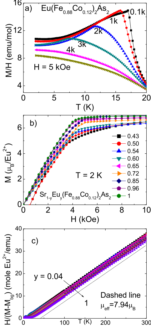
FIG. 9: a) Field dependence of the temperature dependent magnetization divided by applied field for y = 1 for H \parallel ab plane; b) M(H) normalized by yW_{DS} ; c) Inverse magnetic susceptibility, H/M normalized by the actual \text{Eu}^{2+} concentration yW_{DS} .
