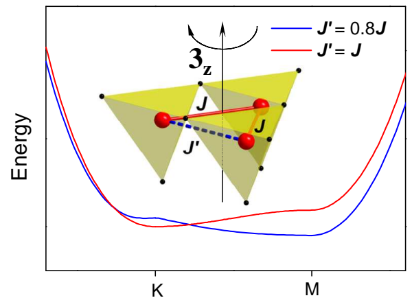
FIG. 9: (Color online) Dispersion relations for low energy mean-field ordered states in the case of equivalent ( J = J' ; three-fold symmetry is preserved) and two non-equivalent ( J \neq J' ; three-fold symmetry is broken) exchange parameters in the system (see Ref. 30 for details of the mean-field approach).
