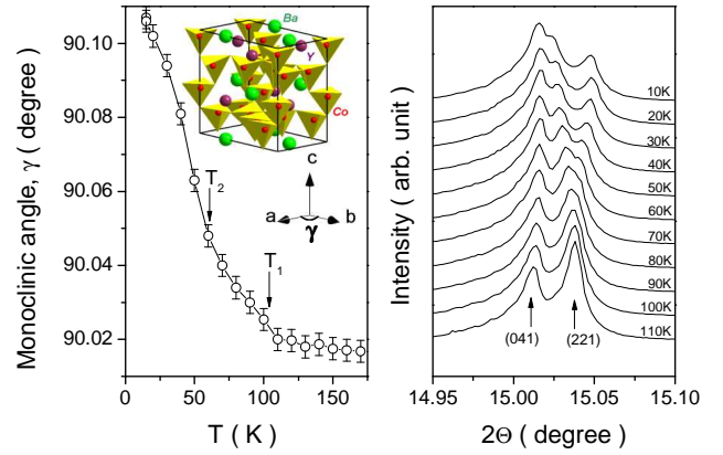
FIG. 5: (Color online) Monoclinic angle as a function of temperature (left panel). The inset shows the orthorhombic unit-cell and the angle \gamma which deviates from 90^\circ in the monoclinic phase. A part of the X-ray powder diffraction patterns collected at different temperatures and demonstrating the splitting of the (221) reflection below T_1 \sim 100 K (right panel).
