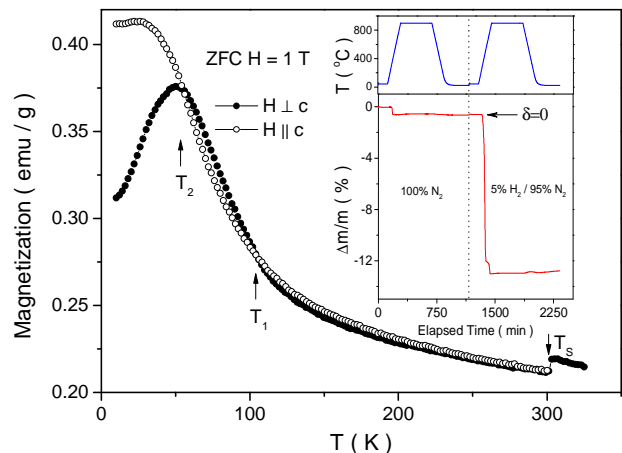
FIG. 1: (Color online) Magnetization of the stoichiometric \text{YBaCo}_4\text{O}_7 single crystal as a function of temperature measured for two directions of the field after cooling in zero field. Inset shows an example of TGA data measured on an as-made \text{YBaCo}_4\text{O}_{7+\delta} polycrystalline sample.
