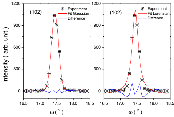
FIG. 4: (Color online) Example of \omega -scan profile for the (102) reflection measured at 5 K on the D10 diffractometer and fitted with a Gaussian (left) and Lorentzian (right) functions. The reflection, forbidden in the Pbn2_1 space group, has mainly a magnetic contribution (some small nuclear contribution can exist since it is allowed in P112_1 ).
