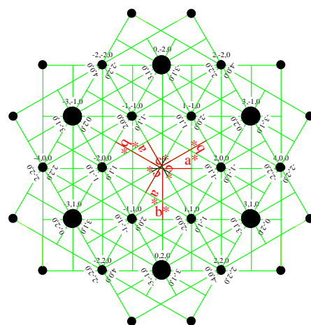
FIG. 2: (Color online) A part of the (hk0) reciprocal plane demonstrating superposition of the three types of 120° ferroelastic domains, expected in the case of the orthorhombic symmetry.
