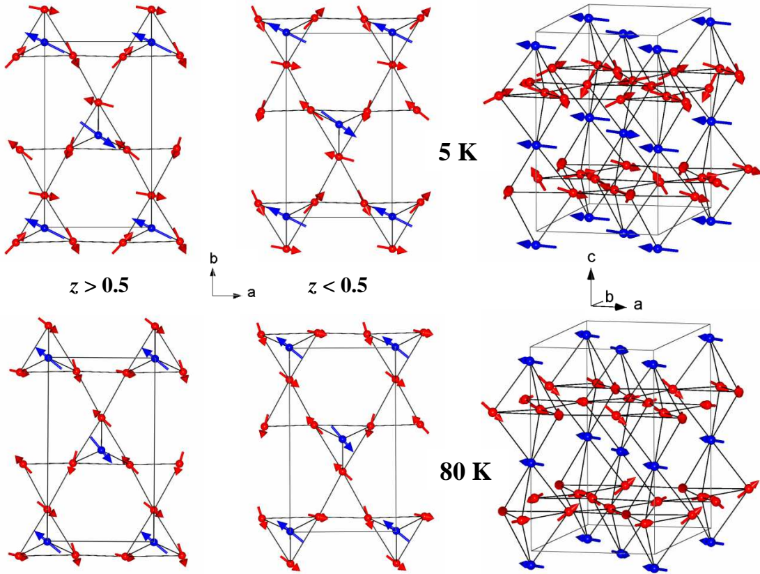
FIG. 7: (Color online) Schematic representation of the magnetic structure of \text{YBaCo}_4\text{O}_7 at different temperatures. The spins in triangular and Kagome sublattices are presented as large (blue) and small (red) arrows, respectively.
