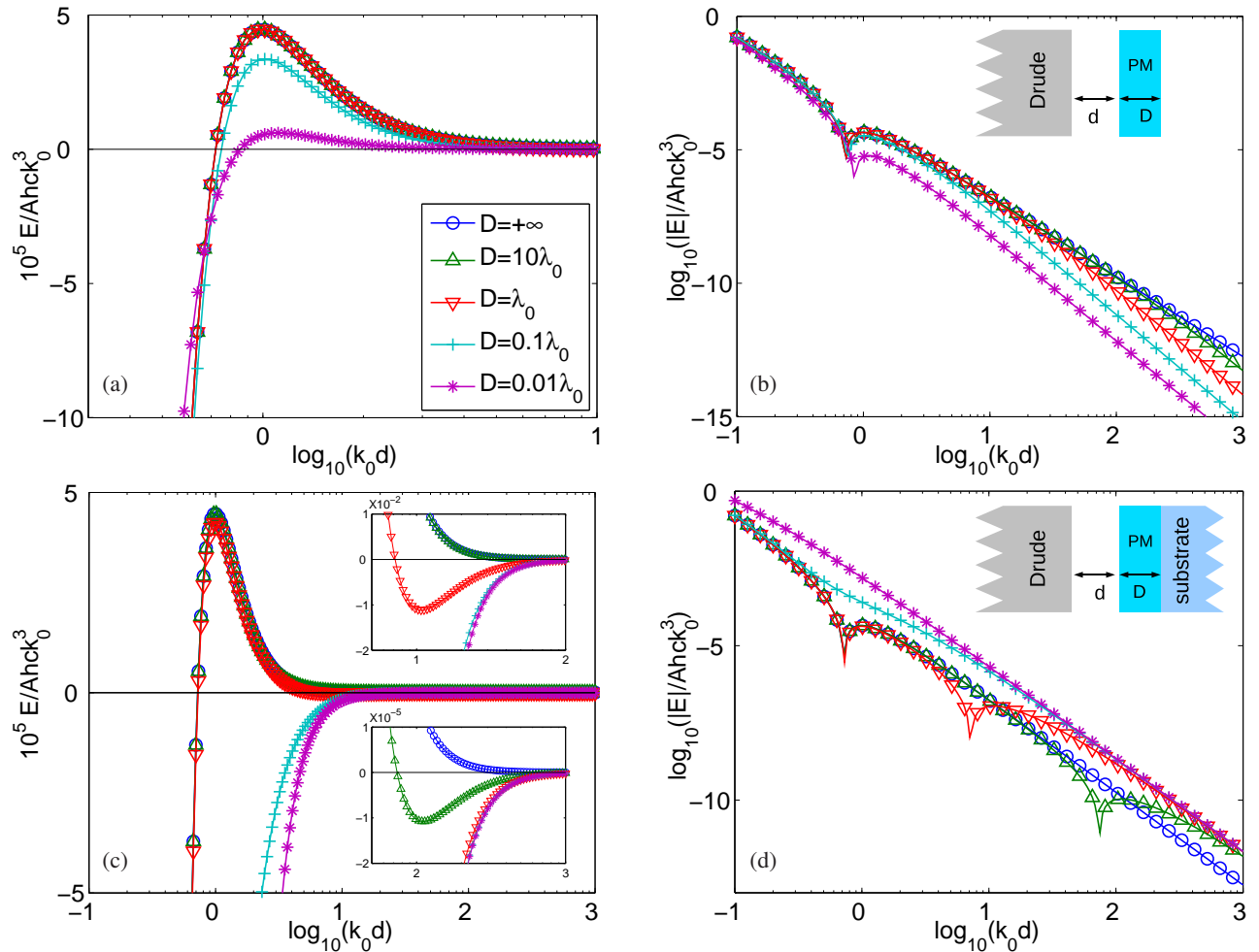
FIG. 1: (Color online) Casimir interaction energy per unit area E(d)/A (in unit of hc k_0^3 ) versus k_0d between a semi-infinite Drude metal plate and a finite magnetic slab without substrate ((a) and (b)) and with Drude metal substrate ((c) and (d)). The insets in (b) and (d) show the schematic figures depicting the arrangements of the slabs/substrates. The curves correspond to different values of the thickness D of the slab. The linear-log plot (left, (a) and (c)) and the log-log plot (right, (b) and (d)). The insets in (c) magnify the regions around k_0d \simeq 10 and k_0d \simeq 10^2 .
