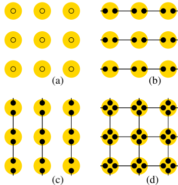
FIG. 5: Tensor-network – a graphic representation of the tensor-product wave function (27) on a 2D square lattice. The indices on the links are summed over.
