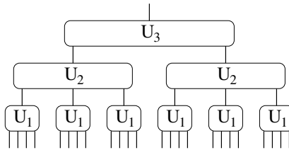
FIG. 3: A \{n_i\} -block TI LU transformation described by a quantum circuit of three layers. Here n_1 = 4 , n_2 = 3 , n_3 = 2 . The unitary transformations U_i on different blocks in the i^{\text{th}} layer are the same.
