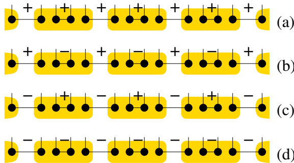
FIG. 4: (Color online) Representative states of the four parity symmetric phases, each corresponding to (a) \alpha(P) = 1, \beta(P) = 1 (b) \alpha(P) = -1, \beta(P) = 1 (c) \alpha(P) = -1, \beta(P) = -1 (d) \alpha(P) = 1, \beta(P) = -1 . + stands for a parity even entangled pair (e.g. |00\rangle + |11\rangle ), - stands for a parity odd entangled pair (e.g. |01\rangle - |10\rangle ). Each site contains four virtual spins.
