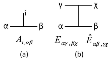
FIG. 8: Graphical representation of (a) matrices labeled by physical index i (b) double tensor denoted by \mathbb{E} or \hat{\mathbb{E}} . \mathbb{E} is a matrix with \alpha\gamma as row index and \beta\chi as column index. \hat{\mathbb{E}} is a matrix with \alpha\beta as row index and \gamma\chi as column index.
