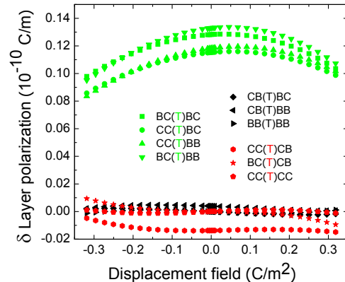
FIG. 1: (Color online) Dependence of \text{TiO}_2 layer polarizations (relative to the average of \text{TiO}_2 planes in bulk \text{BaTiO}_3 and \text{CaTiO}_3 ) on chemical environment in CTO/BTO supercells.
