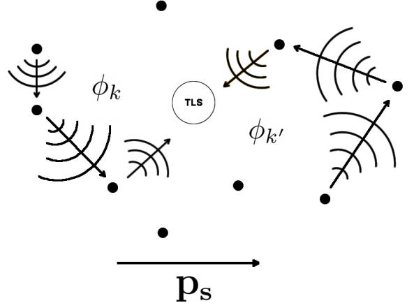
Figure 2: Illustration of the Friedel oscillations caused by interference of electron waves scattered from multiple impurities. The black dots represent randomly distributed impurities.
