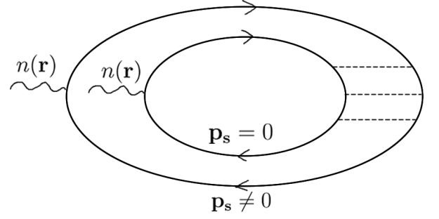
Figure 3: Feynman diagrams for calculating \langle (\delta n)^2 \rangle . The dashed lines represent disorder averaging. The solid line correspond to the electron Green's functions, which are matrices in the Gorkov-Nambu space.
