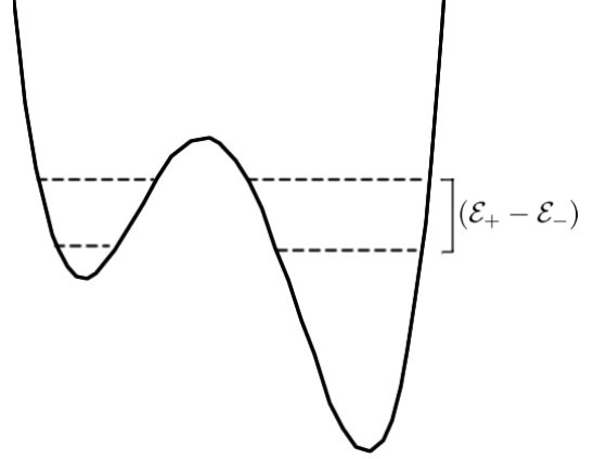
Figure 1: Qualitative picture of a TLS potential plotted as a function of the configurational coordinate. The dashed lines represent the energy eigenvalues in the two states of the TLS, which differ by (\mathcal{E}_+ - \mathcal{E}_-) .
