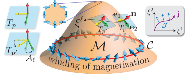
FIG. 1. Depiction of manifold \mathcal{M} . The winding of the magnetization \mathbf{m} (blue arrows) on the contour \mathcal{C} (red line) determines the vortex charge enclosed by \mathcal{C} . The local tangent planes T_p and T_{p'} are shown for points p and p' , along with the local frame \{\mathbf{e}_1, \mathbf{e}_2, \mathbf{n}\} . The leftmost tangent planes depict the gauge potential \mathcal{A}_\ell at point p' , which captures changes of \mathbf{e}_1 and \mathbf{e}_2 along \xi^\ell . The inset shows vorticity flux \mathcal{J} being pumped transverse to a metallic wire (purple curve) carrying electric current density \mathbf{j} .
