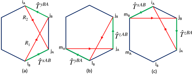
FIG. 1. The configurations that give CS terms. The green lines represent the \hat{T} matrices and red lines are associated with Green function elements.
