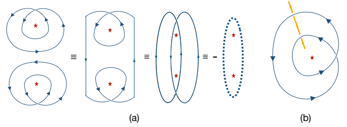
FIG. 2. Illustration of fusion rules for twist defects. The blue and yellow line represent the string e^{i \int \vec{a}^* \cdot d\vec{l}} and e^{i2 \int \vec{a}^* \cdot d\vec{l}} respectively. In (a) fusion of two closed strings that wind twice are shown. The dotted line measures the fermion number parity within. The fusion between the quasiparticles \psi and \sigma is shown in (b).
