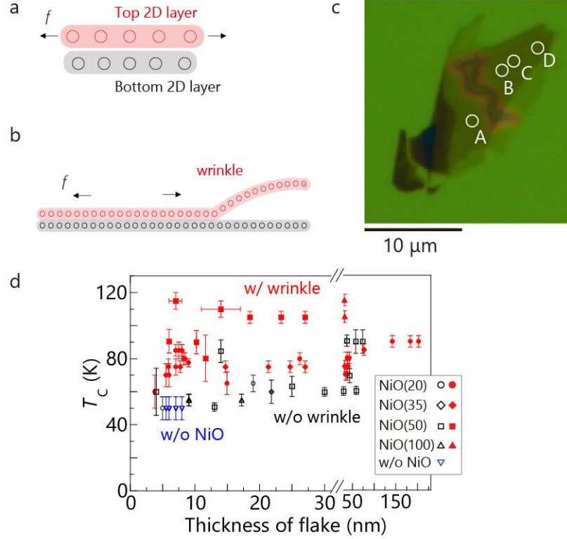
FIG. 1. Wrinkle formation in \text{Cr}_2\text{Ge}_2\text{Te}_6/\text{NiO} and impact on magnetic T_c a , Schematic mechanism to form wrinkle in 2D layers (focusing on two representative layers represented by red and black shaded regions). Each circle represents an atom. In the top layer, an in-plane tensile force f is applied and result in a lateral displacement of atoms from the original positions (indicated in the bottom layer in black). b , In other regions than the part shown in a , the low density of atoms may induce a deformation of the layer (such as wrinkles), especially when the coupling to the adjacent layers is weak, which is the case in 2D materials. c , Optical micrograph of a \text{Cr}_2\text{Ge}_2\text{Te}_6 flake with a 50-nm-thick NiO overlayer. Wrinkles appear as wavy patterns near the center of the flake. Several representative positions are marked as circles (A, B, C and D). d , Curie temperatures of \text{Cr}_2\text{Ge}_2\text{Te}_6 flakes of different thickness (bottom axis), with (data in red and black) and without (blue) NiO layer. The results for flakes with (without) wrinkles are indicated by closed red (open black) symbols. The symbols reflect the NiO thickness: 20 nm (circle), 35 nm (diamond), 50 nm (rectangle), and 100 nm (triangle).
