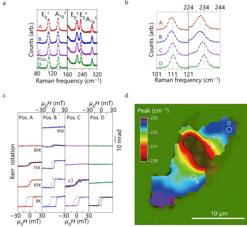
FIG. 2. Raman spectra and magnetic properties of a wrinkled flake. a , Raman spectra of the flake at positions A (red), B (blue), C (purple), and D (green) shown in Fig.1c, in the 80 – 320 \text{cm}^{-1} range. According to theoretical calculations, five peaks E_g^1 , E_g^3 , E_g^4 , ( A_{1g}^2 , A_{1g}^5 ) are expected in this frequency range, three (two) of which are nearly doubly degenerated (non-degenerated) modes. b , Zoomed-in spectra from (a) around the E_g^1 (left) and A_{1g}^2 (right) peaks (vertical dotted lines mark the Raman peak for position D). The solid lines connecting the data points represent fitted curves. c , Kerr rotation at positions A (red), B (blue), C (purple) and D (green), from left to right. The hysteresis curves for magnetic fields (applied perpendicular to the sample plane) are presented for several temperatures (8 K, 65 K, 75 K, 85 K and 95 K). The curves are shifted vertically for clarity. Sweeps from positive to negative fields (or reverse) are indicated by dotted or black (or solid) lines. The vertical scale bar indicates 10 mrad. d , Spatial distribution of the Raman “ E_g^4 ” peak position (plotted as color, except the green background color outside the flake). The color and contour plot were generated by interpolating values measured every 0.8 \mu\text{m} .
