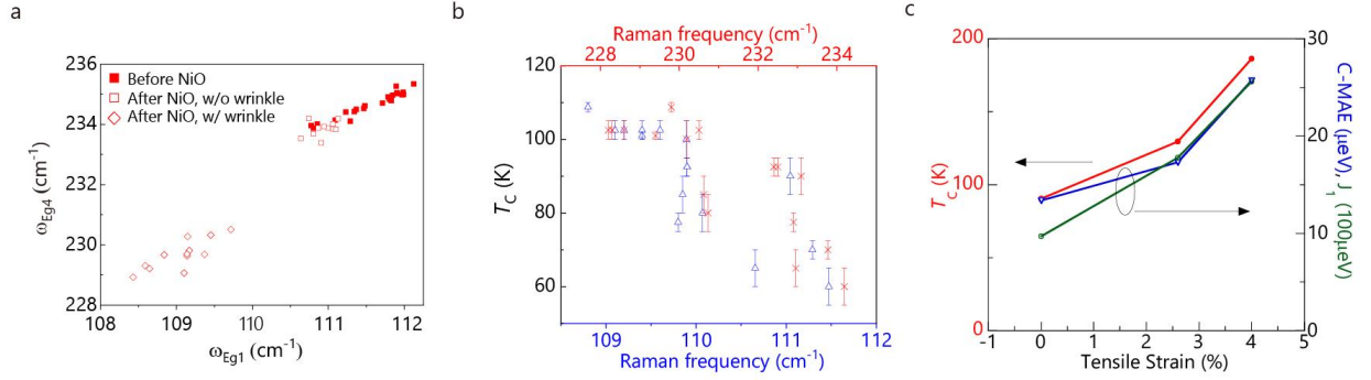
FIG. 3. Correlation between tensile strain and enhanced magnetism. a , The correlation between peak positions of two in-plane Raman modes ( E_g^4 vs. E_g^1 ) for \text{Cr}_2\text{Ge}_2\text{Te}_6 . Samples (before) after depositing NiO which do not show wrinkles are indicated as (open) solid rectangles and circles. Samples after depositing NiO which show wrinkles are indicated by diamonds. b , Relationship between the measured Curie temperature ( T_C ) and the two in-plane Raman modes peak positions (top ( E_g^4 ) and bottom ( E_g^1 ) axes) for \text{Cr}_2\text{Ge}_2\text{Te}_6 samples with a NiO overlay. c , Curie temperature T_C (red filled circle), crystalline magneto anisotropy energy C-MAE (blue triangle), and first exchange coupling J_1 (green empty circle) with respect to the in-plane tensile strain, from DFT calculations.
