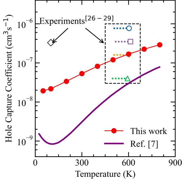
FIG. 2. The equilibrium hole-capture coefficient for C impurities at N sites in GaN. The hole-capture coefficient reported by A. Alkauskas et al. 7 at W_{if} = 1.02 eV ( \Delta E in their notation) is also displayed in purple. Reported experimental values of capture coefficients are displayed as empty symbols, and dotted lines indicate the range of temperatures in which they are reliable. 26-29 The four different symbols in the dashed-line rectangle are data extracted from four different samples.
