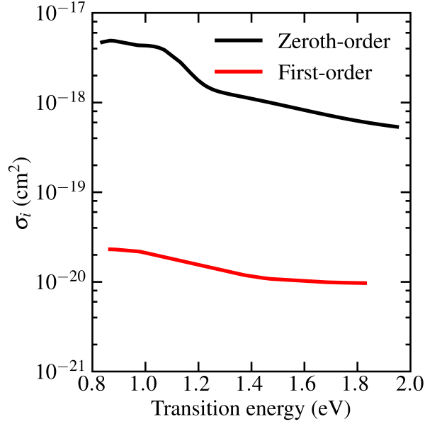
FIG. 1. Zeroth- and first-order contribution to electron-capture cross section ( \sigma_i ) of a triply-hydrogenated, positively charged vacancy in Si (a model dangling bond) as a function of the transition energy, namely the total electronic energy difference E_f(\{\mathbf{R}_k^{(i)}\}) - E_i(\{\mathbf{R}_k^{(i)}\}) as defined in Eq. (58).
