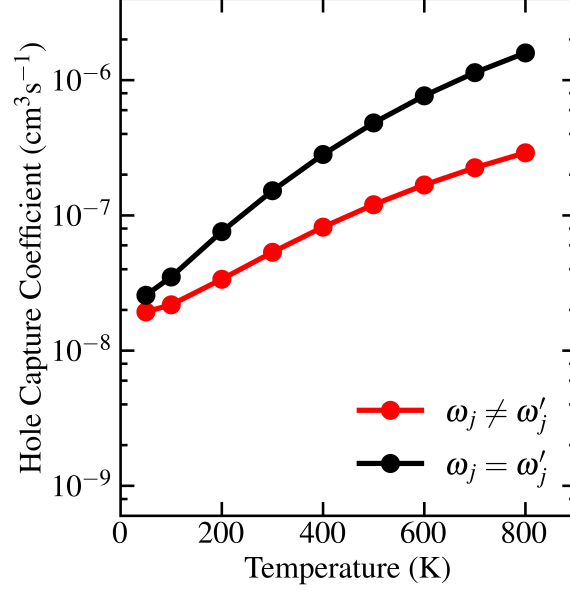
FIG. 3. Comparison plot of the hole-capture coefficient calculated using the phonon frequencies of the initial and final configurations ( \omega_j \neq \omega'_j ) and invoking the approximation of using the phonon frequencies of the final configuration for both configurations ( \omega_j = \omega'_j )
