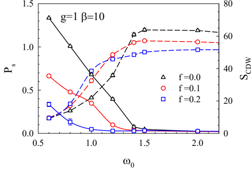
FIG. 3. Pairing and CDW correlations as functions of \omega_0 for different dilution fractions. Dashed lines represent P_s while solid lines represent S_{\text{cdw}} . The inverse temperature is fixed at \beta t = 10 . CDW and SC compete, but coexistence is possible in the region of transition between them.
