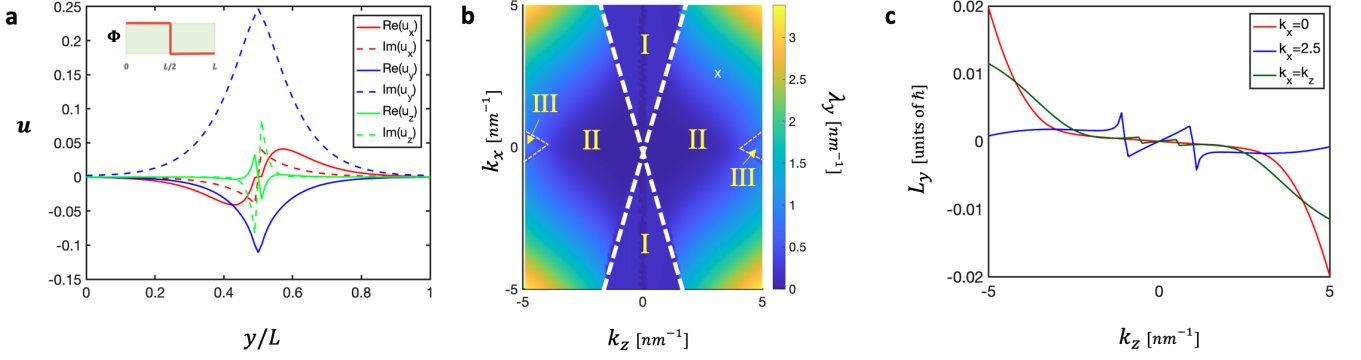
FIG. 2. (a) The spatial distribution of the real and imaginary parts of the displacement field of the interface phonon mode at point X where (k_x, k_z) = (2.5, 3)\text{nm}^{-1} . The u_y component (both real and imaginary) is even across the axion domain wall whereas the x and z components are odd. (b) The inverse decay length ( \Lambda ) of the dominant u_y component of the displacement as a function of (k_x, k_z) (c) The out of plane ( y direction) phonon angular momentum of the interface mode at k_x = 0 (red), k_x = 2.5\text{nm}^{-1} (blue) and k_x = k_z (dark green). We use r = .8 ; s = .713 ; t = .9 in units of 10^{-12}m^4/s^2 and a = 6.75, b = 3.17, c = 1.01, d = 1.93, f = 11.02 in units of 10^6 m^2/s^2 .
