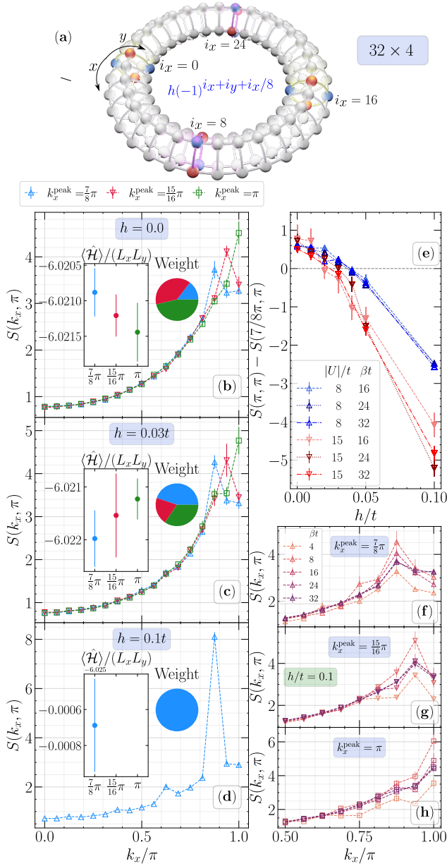
FIG. 3. (a) Schematic representation of the 32 \times 4 ladder with periodic boundary conditions and the antiphase staggered pinning field at i_x = 0, 8, 16, 24 . (b–d) Structure factor S(k_x, \pi) for the fermionic model at \beta t = 24 with increasing magnitude of the modulated pinning potential h/t = 0; 0.03 and 0.1 , respectively; here the realizations are filtered according to the peak location k_x^{\text{peak}} — the pie chart gives the fraction of the total number of realizations exhibiting a given peak in S(k_x, \pi) and the remaining inset the average energy per site for each corresponding k_x -value. (e) The difference between the CDW structure factor and the one that gives a period-8 stripe averaged over all realizations: only after imposing a large pinning potential can a single-mode stripe be formed. (f–h) The temperature dependence of S(k_x, \pi) with h/t = 0.1 for realizations exhibiting k_{\text{peak}} = \frac{7}{8}\pi, \frac{15}{16}\pi and \pi , respectively.
