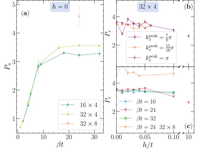
FIG. 4. (a) Saturation of the s-wave pair structure factor with the inverse temperature for three different system sizes without antiphase staggered pinning potentials h(-1)^{i_x+i_y+i_x/8}\hat{n}_i . The effect of h on the pairing for the 32 \times 4 lattice, resolved by k_x^{\text{peak}} (b) or by temperature and system size (c). Note the broken axis with a value included at a large h , showing an overall reduction of the pairing once stripes become increasingly pinned. Data are shown for |U|/t = 15 ; imaginary-time discretization is t\Delta\tau = 0.05 as in Fig. 3.
