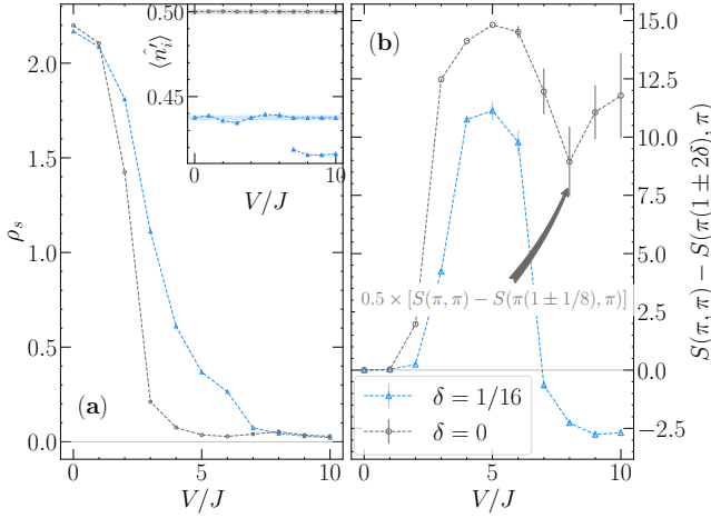
FIG. 2. (a) The superfluid weight vs. interaction strength V with ( \delta = 1/16 ) and without ( \delta = 0 ) doping on the hardcore boson model shows that in the presence of stripes, \rho_s \simeq 0 . These are seen in the inset, the shaded horizontal area gives the average total density target, and the markers the calculated density – once charge stripes are formed for V \gtrsim 7J , these lead to a second lower density for \delta = 1/16 at certain regions (b) The difference in the density structure factor for two values of k_x , \pi and \pi(1 \pm 2\delta) ; when negative, it signals the emergence of stripes with anti-phase density ordering — the undoped ( \delta = 0 ) case is rescaled by 0.5 for easier visualization.
