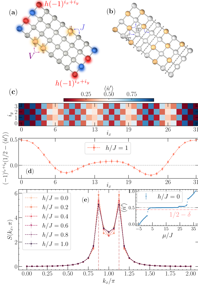
FIG. 1. (a) Schematic representation of the lattice with relevant terms of the hardcore boson Hamiltonian annotated, including staggered pinning potential at the edges with magnitude h . (b) Representation of the ‘charge \pi -phase shift’ that emerges in the strongly interacting limit ( V/J \gg 1 ), with contributions in second-order perturbation theory indicated. While the kinetic energy gains within a checkerboard domain are \propto t^2/nV ( n = 2, 3 ) for a given site, bosons can freely hop across the dashed lines marking the stripe locations. (c) density profile in 32 \times 4 ladder exhibiting four hole-regions in its short-direction; here h/J = 1 . (d) The average staggered hole-density profile. (e) The density structure factor S(k_x, \pi) shows robust peaks at k_x = \pi(1 \pm 2\delta) , \delta = 1/16 , even in the absence of pinning potential ( h = 0 ); the inset shows the phase separation characteristics for the studied densities emerging in the equation of state ( \langle \hat{n}' \rangle vs. \mu ). All data are obtained for V/J = 8 .
