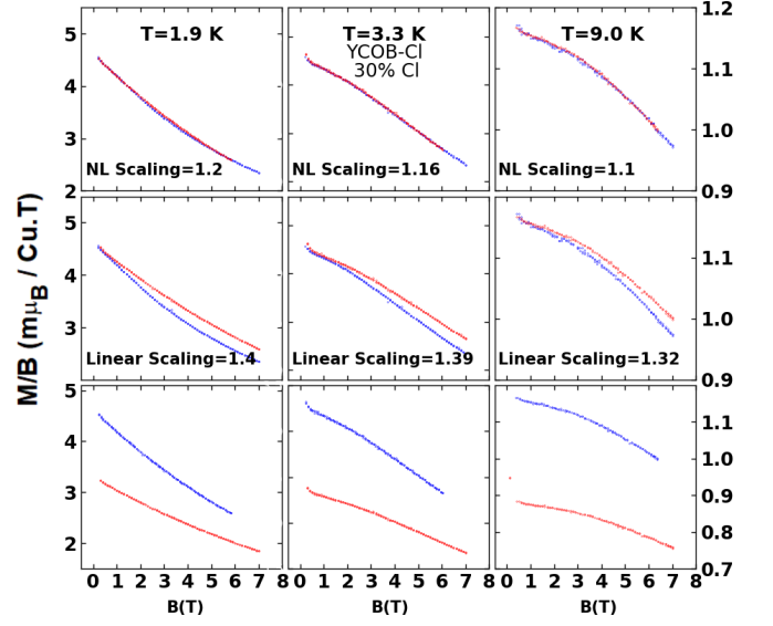
FIG. 3. Shows the anisotropy of the linear and nonlinear magnetization responses of the 30% Cl sample. Results for three separate temperatures are shown each arranged in vertical panels. The bottom panel shows the unscaled raw data for B \parallel c -axis (blue) and B \perp c -axis (red). In the middle panel the B \perp c -axis data is scaled up to match the B=0 values (linear susceptibility scaling). In the top panel the nonlinear susceptibilities merge when the B axis for B \perp c -axis is scaled by a scaling constant labelled as NL (nonlinear) in the figure. For T=3.3\text{K} the vertical scale begins as shown on left but is expanded by a factor of two. The scale on the right applies only to the 9.0K data.
