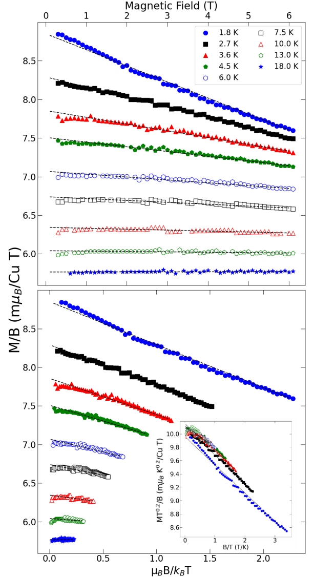
FIG. 1. Magnetization M/B isotherms obtained on the pure Bromine sample. Top: Shows M/B vs B at different temperatures as indicated. The slopes at high temperature are nearly zero but turn rapidly negative and diverge strongly as T \rightarrow 0 . Similar isotherms are obtained on the 21% and 30% chlorine doped crystals (see supplementary information). We also verified that both field cooled (FC) and zero field cooled (ZFC) procedures gave identical isotherms. Bottom: M/B plotted against a dimensionless ratio of magnetic field and temperature. Inset: Same data as in the bottom main panel to show that the curves collapse when scaled by T^{0.2} .
