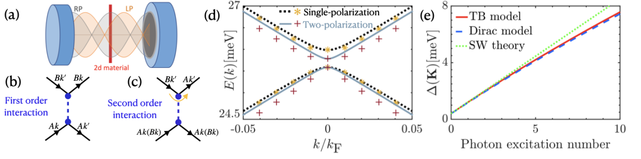
Figure 1. (a) Chiral cavity setup with right and left polarizations are shifted with respect to each other. (b-c) The cavity mediated electronic interactions in graphene with strengths proportional to (b) 1/\omega_\lambda and (c) 1/\omega_\lambda^2 . (d) The focus on the lowest two bands of two- and single-polarization Dirac models showing the match between analytical SW theory and exact diagonalization (ED) with a truncated photonic Hilbert space of maximum photon number \langle a_j^\dagger a_j \rangle_{\max} = 4 . Single-polarization bands (dotted-black) are shifted upwards for comparison by \omega_L/2 . The x-axis is defined in terms of radial distance to the Dirac nodes k = \sqrt{k_x^2 + k_y^2} normalized by Fermi momentum k_F = mv_F . The parameters are \omega_c = 6.28 THz, \chi = 5 \times 10^{-4} [31] and m = 0.02m_e . Fermi velocity is found to be v_F = 0.21 a.u. (atomic units) by fitting the band structure of the Dirac model to the TB model. The red-pluses and yellow-stars are the prediction of the analytical SW theory in vacuum. (e) The gap at \mathbf{K} point when the cavity is prepared in a Fock state, increases with the photon number populated in the cavity. SW theory can predict the gap until \langle a_R^\dagger a_R \rangle \sim 5 . The ED results with \langle a_j^\dagger a_j \rangle_{\max} = 4 on Dirac and TB models match.
