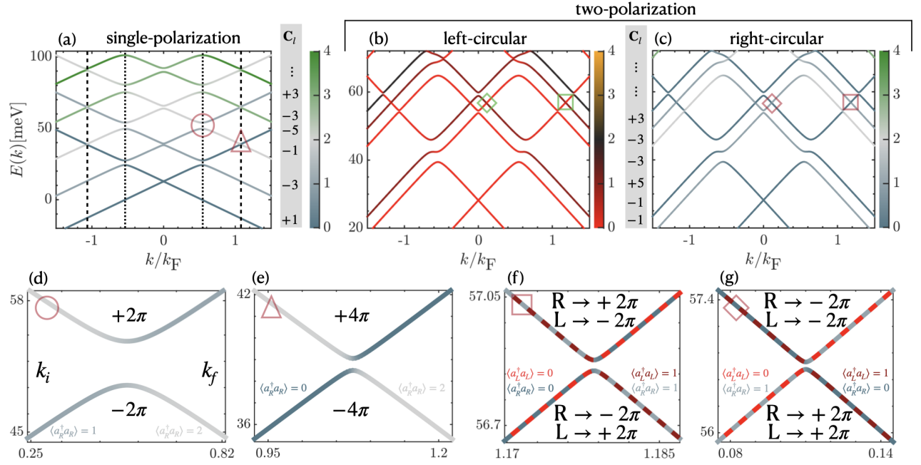
Figure 2. The exact diagonalization Dirac bands of graphene around the \mathbf{K} point coupled to a cavity with (a) single polarization and (b-c) two-polarization of cavity frequency \omega_c = 6.28 THz with color coding denoting the photon populations and \langle a_j^\dagger a_j \rangle_{\max} = 4 . We use m = 0.02m_e , \chi = 5 \times 10^{-4} [31] and \gamma = 1.2 as the free parameters of the theory that have to be fixed by the experiment. The light-red shapes highlight the light-matter avoided crossings with chiral photon exchanges. The Chern numbers for both models are given in boxes under C_l for band l and calculated in the full BZ with the TB model. (d-g) Focus on chiral photon exchange processes with Berry phases for each band denoted. The photon numbers are written only for the lower bands. Subfigures (d-e) show the role of photon number, whereas (f-g) show also the role of polarization in determining the Berry phase of the photo-electron wave function at a light-matter avoided crossing.
