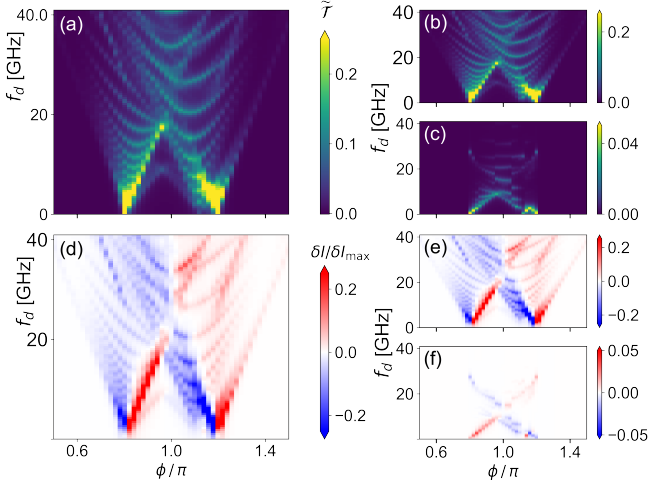
FIG. 4. (a)-(c) The transition lines and (d)-(f) \delta I(f, \phi) for the ABS from Fig. 2(c) with suppressed higher-energy single-particle transitions. The lines \tilde{T}(f, \phi) in (a) are resolved into (b) pair and (c) single-particle transitions. The remaining transition lines in (c) are due to the energy-split overlapping MBS. (d) \delta I(f, \phi) displays the gap closing and reopening. \delta I(f, \phi) shown from (e) pair and (f) single-particle transitions, reveals the gap closing and opening as well as the transitions from E \approx 0 split MBS.
