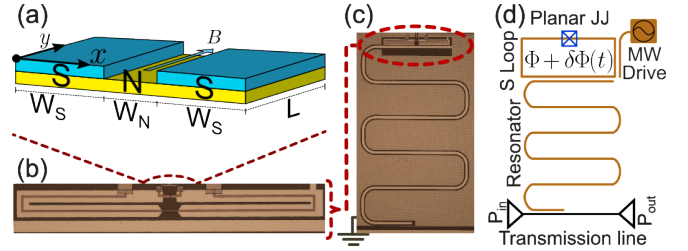
FIG. 1. (a) A planar JJ formed by two Al superconducting (S) regions covering InAs-based 2DEG normal region (N). Coordinate axes and JJ dimensions are indicated. Alternating current, I , flows along \pm\hat{x} ; the applied magnetic field is \mathbf{B} . (b)–(d) Optical images of an example fabricated SQUID resonator, which we consider in our theoretical results. Gold: Al, dark brown: the etched mesa, and light brown: gate and a flux line. (c) Device diagram with resonator capacitively coupled to a transmission line and inductively to a superconducting loop with a flux \Phi and a single JJ. (d) Schematic description from (c) of the JJ, SQUID, microwave drive line inducing fluctuations in \Phi \rightarrow \Phi + \delta\Phi(t) , resonator, and transmission line with input (output) power P_{\text{in}} ( P_{\text{out}} ).
