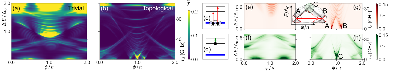
FIG. 3. (a), (b) Transition lines \tilde{T}(f, \phi) , calculated using Eq. (4), corresponding to hf_d = \Delta E = |E_n - E_m| between ABS from Figs. 2(a) and (c), with a Lorentzian broadening parameter \varepsilon = 30 mK. In the schematic of pair (c) and single-particle (d) transitions where the ground state is denoted by a blue line, the sum of the arrow lengths in (c) gives \Delta E . Resolving (e) pair and (f) single-particle transitions from (a) up to 40 GHz shows no gap closing and opening. In contrast a similarly resolved (g) pair and (h) single-particle transitions from (b) reveal signatures of topological superconductivity. The inset: an enlarged part of the Fig. 2(c) spectra. The transitions in the circles “A” and “B” of the inset lead to the “V”-shaped features “A” and “B” in (g), signaling a gap closing and reopening. Transitions in the circle “C” lead to the “V”-shaped feature “C” in (h).
