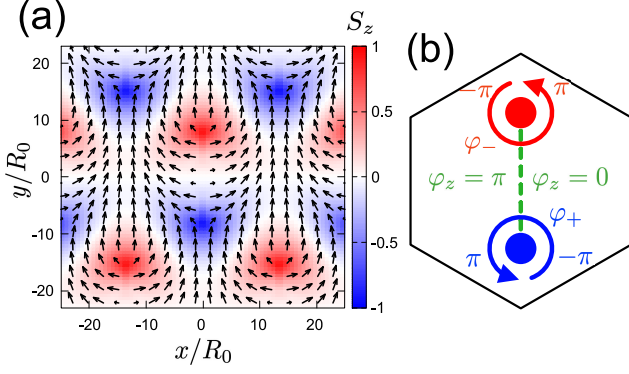
FIG. 1. (a) Spin texture \mathbf{S} = i(\mathbf{d} \times \mathbf{d}^*)/|\mathbf{d}|^2 with \bar{B} = 0.01B_0 , \mu = 1 , and T = 0.2T_c . (b) Schematic picture for phases of d-vector components in a unit cell of the hexagonal vortex lattice. The green dotted line indicates the phase string across which the phase of d_z jumps by \pi . Both ends, indicated by red and blue dots, correspond to the half-quantized vortices.
