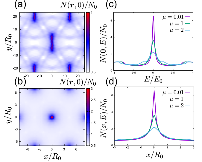
FIG. 3. Zero energy LDOS for the spin texture under \bar{B} = 0.01B_0 (a) and singular vortex structure with uniform spin parallel to the y -axis under \bar{B} = 0.1B_0 (b) with \mu = 1 and T = 0.2T_c . Energy profiles of the LDOS N(0, E) at the vortex core (c) and spatial variations of the zero energy LDOS N(x, 0) along the x -axis (d) for the singular vortex structure with \mu = 0.01 , \mu = 1 , and \mu = 2 .
