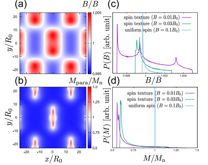
FIG. 2. Spatial variations of internal field B(\mathbf{r}) (a) and paramagnetic moment M_{\text{para}}(\mathbf{r}) (b) with \bar{B} = 0.01B_0 , \mu = 1 , and T = 0.2T_c . Distributions of internal field P(B) (c) and paramagnetic moment P(M_{\text{para}}) (d) with \mu = 1 and T = 0.2T_c . The distributions are shown for spin textures under \bar{B} = 0.01B_0 and \bar{B} = 0.03B_0 , and singular vortex structure with uniform spin parallel to the z -axis under \bar{B} = 0.1B_0 .
