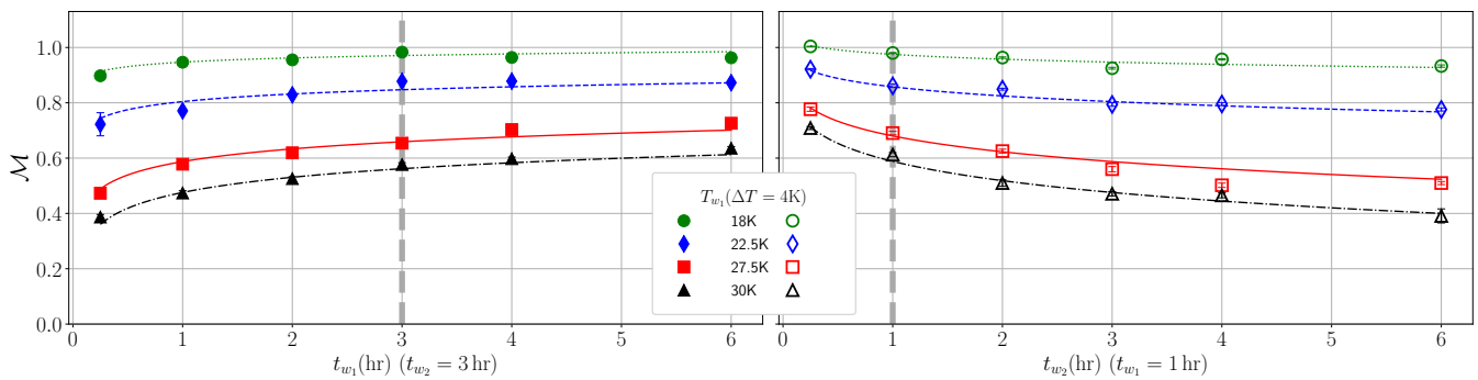
FIG. 2. Memory versus waiting time with four different first waiting temperatures. For both (a) and (b), the first and second waiting temperatures are the same: T_{w_1} = (18, 22.5, 27.5, \text{ and } 30 \text{ K}) and T_{w_1} - T_{w_2} = 4 \text{ K} . In both cases either t_{w_1} (a) or t_{w_2} (b) were varied from 0 – 6 hours (the horizontal axis), while the other waiting time was fixed at 3 and 1 hour, respectively. Closed (open) markers with statistical error bars indicate a variation of t_{w_1} ( t_{w_2} ). The lines are predictions based on our model described by Eq. 5. As discussed in the text, the vertical dashed lines are where we expect a crossing if memory only depends on the ratio of the spin glass correlation lengths.
