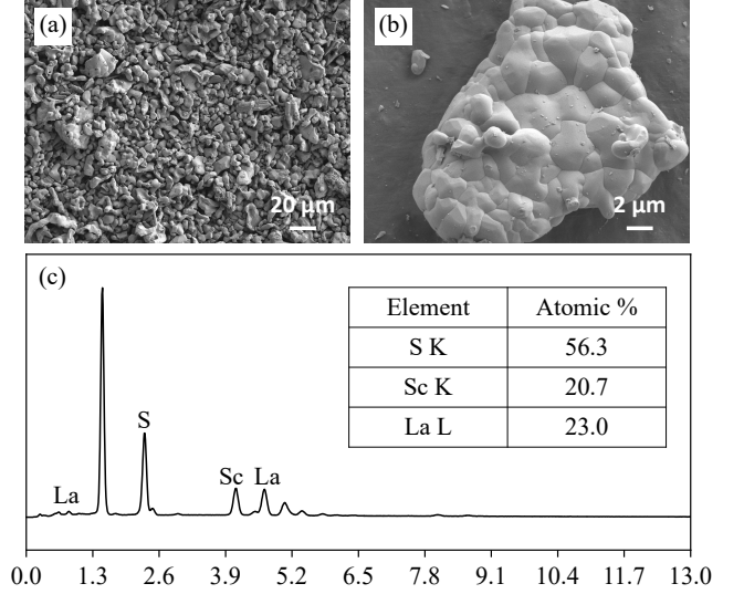
FIG. 3. SEM images of the synthesized \text{LaScS}_3 sample magnified by 500 (a) and 5000 times (b) and EDS spectrum (c) acquired from the sample in (b). The table of the inset lists the atomic ratio of the La, Sc, and S elements determined from the EDS measurement.
