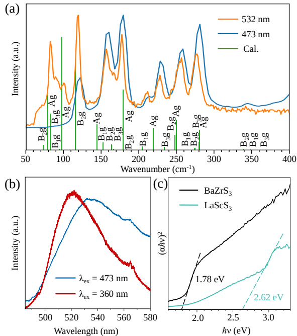
FIG. 4. (a) Raman spectra of \text{LaScS}_3 obtained using laser wavelengths of 532 nm and 473 nm. The calculated Raman peak positions and intensities, as well as the symmetry labels, are shown for comparison. (b) PL spectra of \text{LaScS}_3 using excitation laser wavelengths of 473 nm and 360 nm. (c) Optical absorption spectra of \text{LaScS}_3 and \text{BaZrS}_3 from diffuse reflectance spectroscopy.
