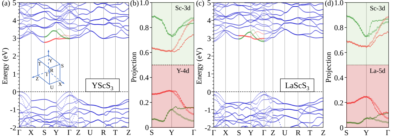
FIG. 1. (a) and (c) show the band structures of \text{YScS}_3 and \text{LaScS}_3 based on HSE06 functional calculations. The inset shows the irreducible Brillouin zone. (b) and (d) show the projection of bottom four conduction bands, as highlighted in (a) and (c), on the d orbitals of A-site and B-site cations along the S-Y- \Gamma path for \text{YScS}_3 and \text{LaScS}_3 , respectively.
