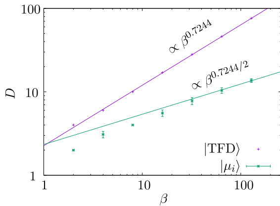
FIG. 3. Minimum bond dimension D necessary to approximate the TFD state and METTS with the truncation error less than 10^{-10} for the critical transverse-field Ising chain with N = 640 sites. The data points for METTS are the average of D of 10000 samples. The error bars indicate the standard deviation. We set the quantization axis \nu to z . Imaginary-time evolution is carried out using the second-order Trotter decomposition with time step \delta\tau = 0.04 .
