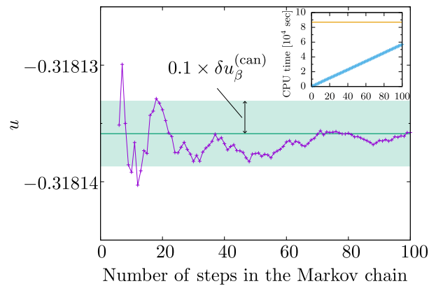
FIG. 4. Typical trajectory of the cumulative moving average of the energy per site u = E/N in the Markov chain of the METTS simulation for the critical transverse-field Ising chain with N = 640 sites at \beta = 128 . We set the quantization axis \nu to z for the odd-numbered steps and x for the even-numbered steps to reduce correlations between successive samples [22]. To avoid initial transients, we discard the first 5 samples when calculating the sample averages. The solid line shows the result of the TFD approach, considered exact, and the shaded region shows a range of 0.1 times the standard deviation \delta u_{\beta}^{(\text{can})} of u in \rho_{\beta}^{(\text{can})} from the exact value. The inset shows the total computation time in the METTS simulation as a function of the number of steps in the Markov chain. The solid line shows the computation time in the TFD simulation.
