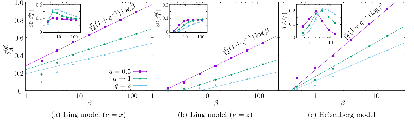
FIG. 2. Growth of the average entanglement Rényi entropy of METTS for the half-chain A = \{1, 2, \dots, N/2\} in the critical transverse-field Ising model of length N = 640 (a, b) and in the critical Heisenberg model with the next-nearest-neighbor interaction of length N = 1280 (c). The insets show the standard deviation of the entanglement Rényi entropy. Imaginary-time evolution is carried out using the second-order Trotter decomposition with time step \delta\tau = 0.04 for the Ising model and \delta\tau = 0.01 for the Heisenberg model. The data is average over 10000 samples for the Ising model and 5000 samples for the Heisenberg model.
