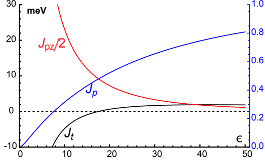
FIG. 3: The couplings in our effective model as a function of the dielectric constant \epsilon . The vertical axis on the left is for J_{pz} and J_t , and the vertical axis on the right is for J_p . In our calculation, the lattice constants are 0.328nm for WSe_2 , 0.315nm for WS_2 , and the moiré lattice constant is a_M = 7.9nm at zero twist angle. m = 0.42m_e is the effective mass for the valence band of WSe_2 . The distance of the top layer and bottom layer is d = 2nm [65]
