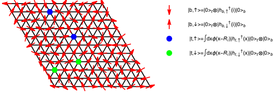
FIG. 2: Illustration of the moiré lattice and the four-dimensional local Hilbert space. The local moments represent the spin degree of freedom in the bottom layer. The solid disks represent the doped excitons with density x . Different colors correspond to different spins in the top layer of the exciton state. If we polarize the spin in the top layer, there is one flavor for exciton and the model reduces to a bosonic version of t - J model.
