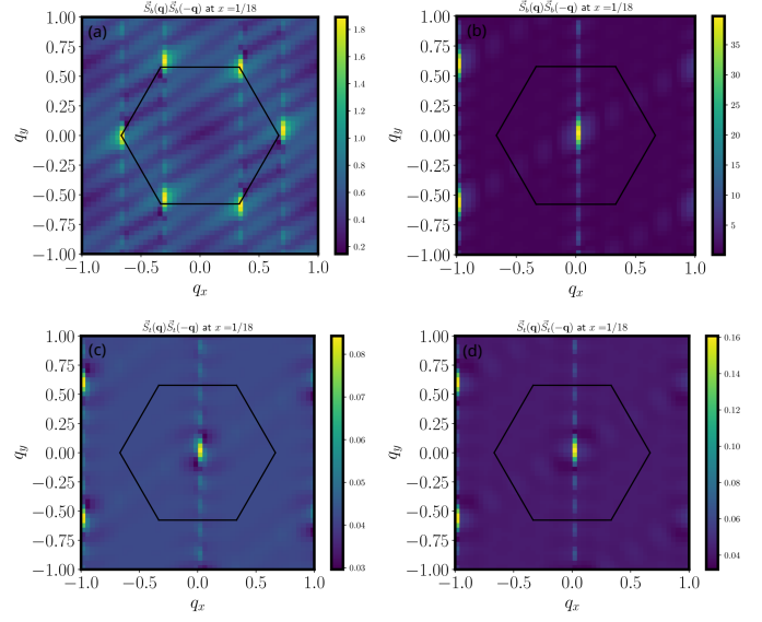
FIG. 4: The spin-spin correlation function for fixed J_b = J_t = 0 , J_{pz} = 5 , x = \frac{1}{18} . (a) and (b) are the spin correlation function \langle \vec{S}_b(\mathbf{q})\vec{S}_b(-\mathbf{q}) \rangle in the bottom layer, and (c), (d) are the spin correlation function \langle \vec{S}_t(\mathbf{q})\vec{S}_t(-\mathbf{q}) \rangle in the top layer. (a) and (c) results for J_p = 1 . (b) and (d) results for J_p = -1 .
