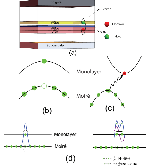
FIG. 1: (a) An illustration of the moiré ( \text{WS}_2/\text{WSe}_2 )+monolayer( \text{WSe}_2 ) system, (b)(c) Two different ways of doping excitons into a Mott insulator.
