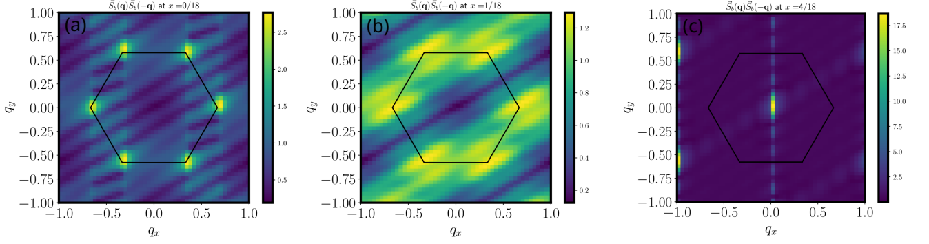
FIG. 5: (a) and (b) the spin correlation function \langle \vec{S}_b(\mathbf{q}) \vec{S}_b(-\mathbf{q}) \rangle for fixed J_t = 0 , J_{pz} = 5 , J_p = -1 , J_b = 0.06 . (a), (b), (c) correspond to the increasing of exciton density.
