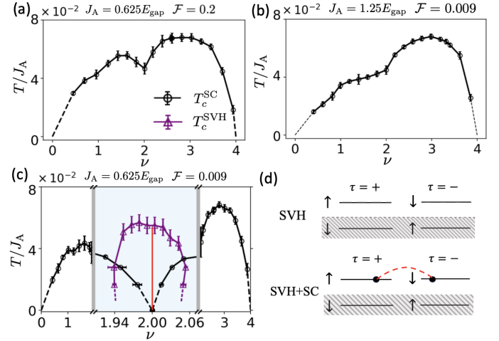
FIG. 1. Superconducting phase diagrams for |J_H| = J_A/2 with: (a) J_A/t = 2.5 and \mathcal{F} = 0.2 , showing a slight suppression of the superconducting T_c^{SC} near \nu = 2 , (b) J_A/t = 5 and \mathcal{F} = 0.009 , and (c) J_A/t = 2.5 and \mathcal{F} = 0.009 , where the zoomed-in blue-shaded region shows the competing SVH insulating state (red solid line) near \nu = 2 . The lightly doped regions near \nu = 2 exhibit a regime with coexisting SC and SVH order for T < \min(T_c^{SC}, T_c^{SVH}) ; see Fig. 2. (d) The top panel shows a schematic of the SVH insulator at \nu = 2 with the shaded regions denoting fully filled electronic bands. The bottom panel is a schematic for the coexisting SVH and SC phases for \nu = 2 + \delta\nu , where the excess electrons (black circles) form spin-singlet Cooper pairs (red dashed line).
