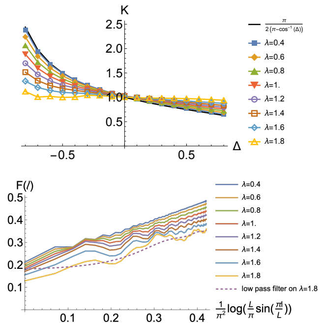
FIG. 1. Upper panel: Luttinger parameter K extracted from subsystem charge fluctuations, as a function of the interaction strength \Delta , for various values of the quasiperiodic potential strength \lambda . At \lambda = 0 there is a known analytic value, plotted as a solid line [41]. Note that as \lambda is increased the curves get increasingly flat, at the noninteracting value K = 1 . Lower panel: dependence of charge fluctuations on subsystem size for interactions \Delta = -0.5 and various values of \lambda . At higher values of \lambda stronger oscillations appear, we thus feed the data through a low pass filter (using 0.1 for the cutoff frequency) in order to smooth out oscillations and then perform a linear fit. DMRG simulations were done with L = 200 and a maximum bond dimension of 200. Data is averaged over 20 phase realizations.
