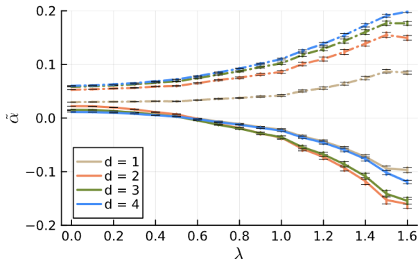
FIG. 4. Hartree (exchange) exponents \tilde{\alpha} characterizing Hartree (exchange) contribution to the Kane-Fisher effect in systems with increasing quasiperiodic potential strength \lambda . Data is computed for system size N = 2501 , filling fraction f = 0.31 , repulsive interaction v_{int} = 0.6 , and averaged over 100 phase realizations. Solid lines: Hartree exponent. Dash-dot lines: Exchange exponent.
