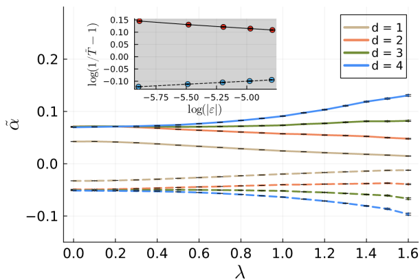
FIG. 3. Exponents \tilde{\alpha} characterizing the Kane-Fisher effect in systems with increasing quasiperiodic potential strength \lambda . Data is computed for system size N = 2501 , filling fraction f = 0.31 , v_{int} = \pm 0.6 , and averaged over 100 phase realizations. Solid lines: \tilde{\alpha} from repulsive interactions; dashed lines: \tilde{\alpha} from attractive interactions. Inset: power-law relationship between \epsilon and 1/\tilde{T}(\epsilon) - 1 for system with \lambda = 1.5 and interaction range d = 1 .
