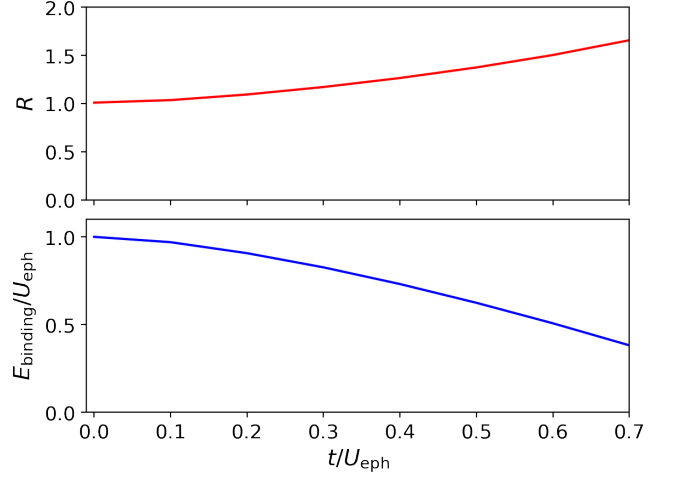
FIG. 2. The properties of bipolarons in the static limit \omega_0 = 0 . We plot the effective radius R of the bipolaron (Eq. 10) in the upper panel and the binding energy E_{\text{binding}} (Eq. 11) in units of U_{e-ph} in the lower panel as functions of the dimensionless constant t/U_{e-ph} .
