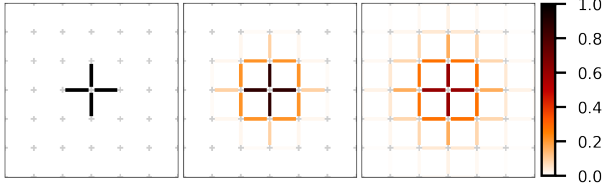
FIG. 1. The phonon configuration \{X_{ij}\} (measured in units of \alpha/K ) around a static bipolaron ( \omega_0 = 0 ) for different values of t/U_{e-ph} = 0.01 (left), 0.35 (middle) and 0.7 (right).
