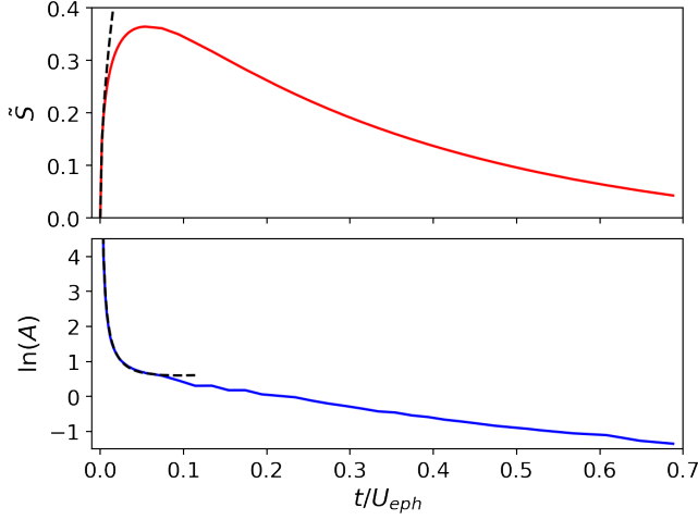
FIG. 4. The energetics of bipolaron hopping. We plot the normalized classical action of the nearest-neighbor tunneling process, \tilde{S} \equiv \frac{\hbar\omega_0}{U_{e-ph}} S_{\text{inst}} , in the upper panel, and the leading-order fluctuational correction to it, \ln(A) , in the lower panel. In the small t/U_{e-ph} limit, we find that the numerical results are well fitted by \tilde{S} \approx 3.2\sqrt{t/U_{e-ph}} (upper panel) and \ln(A) \approx \ln(2.4) + \frac{3}{4} \ln \frac{t}{U_{e-ph}} + 0.46\sqrt{\frac{U_{e-ph}}{t}} (lower panel) which are drawn as dashed lines.
