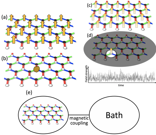
FIG. 1: Noiseless and noisy disturbances to the Kitaev honeycomb. (a) Kitaev honeycomb subject to a uniform magnetic field indicated by yellow arrows. (b) An impurity deposited onto the Kitaev model, shown as a brown speck of dirt, at some lattice point. We treat the case of a quenched magnetic impurity. (c) Kitaev honeycomb model coupled to a noisy but spatially uniform magnetic bath. We consider a uniform magnetic field subject to Gaussian white noise in the quantum master equation. (d) A hole in the system's magnetic shielding couples it locally to a noisy magnetic environment. We model this situation using a noisy magnetic impurity quench. (e) Coupling to a bath, similar to a noisy but spatially uniform magnetic field, is a physical scenario leading to a Lindblad operator in the Quantum Master Equation.
