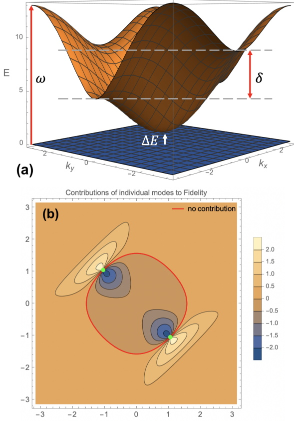
FIG. 2: (a) Oscillation-determining energy scales. The natural energy scales ( \Delta E , \omega , and \delta ) of the problem determine the frequencies of oscillation for the Loschmidt echo. \Delta E and \omega are the band minima and maxima respectively, with \Delta E also being half the band gap. \delta is the energy difference between saddle points in the spectrum, and is inherently 2D. (b) Spinon contributions to stability. Map of regions giving positive (yellow) and negative (blue) contributions to the fidelity relative to the ground state coherence for magnetic field quench. This is shown for the specific case of \mathbf{J} = (1, 1, 1) . Dirac points (green) at \mathbf{k} = (\pm\pi/3, \mp\pi/3) give singular contributions to the integral in Eq.(5), and regions around them contribute most heavily to modifying the fidelity relative to the ground state result. In particular, the plot is of the integrand in Eq.(5) at a particular time; the contribution only becomes more heavily localized around the Dirac points at later times. By virtue of being near the Dirac points, the heaviest contributions also occur in the regions of lowest energy.
