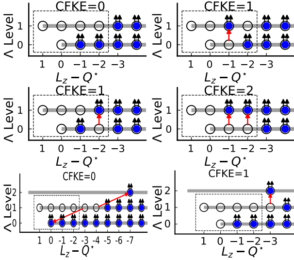
FIG. 2. The top four panels depict the minimal basis that fully captures the hole added to the incompressible state at \nu = 2/5 . The red arrows indicate how these states are obtained starting from the minimum energy state (top left). All excitations are confined to a localized region depicted by the dashed box. The bottom two panels give examples of CF basis states beyond the minimal basis. Their inclusion in CFD broadens the delta function peaks of the minimal basis.
