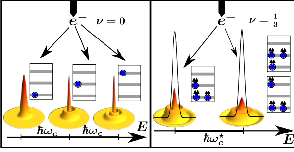
FIG. 5. The left panel shows the density profile of the final state of an electron tunneling into an empty LL. (The states are shown schematically in rectangular boxes.) The right panel shows the density profile (relative to the uniform density ground state) of the final state of an electron tunneling into the 1/3 FQH state for each of the two peaks in Fig. 3. (In the right panel, the density has been multiplied by a factor of two for clarity, and the black curve shows the density profile of an electron tunneling into an empty LLL.) The configurations of the excited CFs that contribute most significantly to the two peaks are also shown schematically. The radius of each disk is \sim 9l_B .
