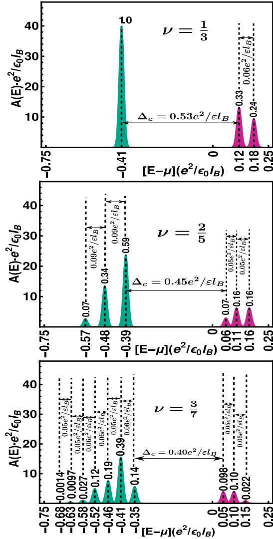
FIG. 3. The spectral function A(E) for \nu = \frac{1}{3}, \frac{2}{5} and \frac{3}{7} calculated using CF theory. The energy is measured in units of e^2/\epsilon l_B , where \epsilon is the dielectric constant, measured relative to the chemical potential \mu . With the exception of the electron side ( E > \mu ) of \nu = 3/7 , the energy and the spectral weight under each peak (shown near its top) represents the thermodynamic value (obtained by extrapolation [19]). The heights of the peaks are proportional to their spectral weights. For ease of viewing, we have substituted the \delta function in Eq. 1 by a normal distribution of width 0.01e^2/\epsilon l_B . For E > \mu at \nu = \frac{3}{7} , results are shown for a system of N = 34 particles; the spectral weights are even smaller in the thermodynamic limit.
