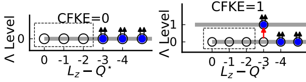
FIG. 1. Left panel: The minimal basis for a hole at \nu = 1/3 enclosed by a dashed box. Right panel: A typical configuration of a basis state with unit CF kinetic energy (CFKE). Here and in the following figures the horizontal lines represent the \Lambda levels, the available CF orbitals are shown by open circles, and the occupied orbitals have CFs, shown as blue dots decorated by two flux quanta (arrows). The spherical geometry is assumed, where L_z is the angular momentum of the orbital and Q^* is the monopole strength experienced by CFs.
