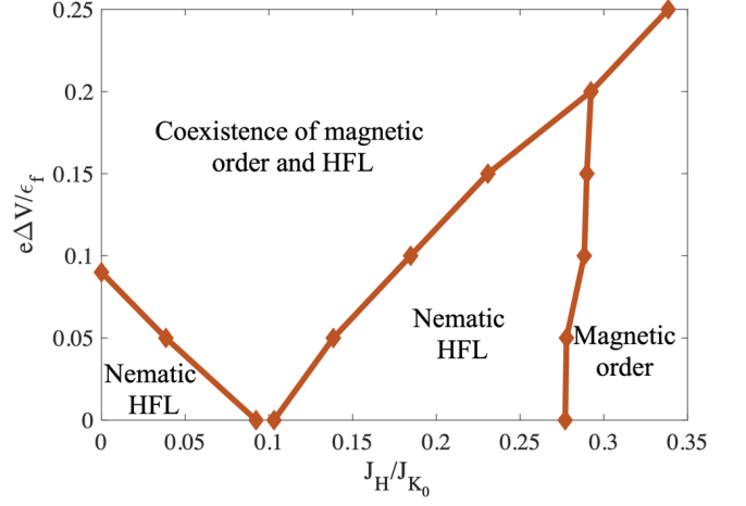
FIG. 4. Effects field tuning of the phase diagram for J'_H/J_K = 0.01 : Electric field shifts the energy levels of the local moments and therefore increases the Kondo interaction on one layer while decreasing it on the other layer. This significantly enhances the stability of the coexistence of magnetic order and HFL.
