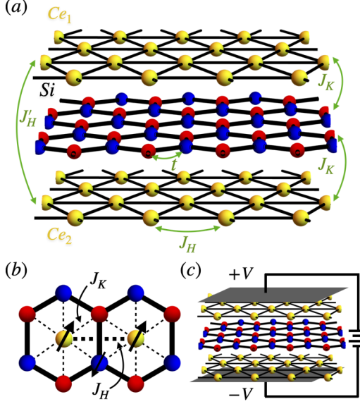
FIG. 1. (a) Schematic of the model: Ce sites (yellow) form two layers of triangular lattice. The silicene layer – a honeycomb lattice formed by Si atoms (red and blue for the A and B sublattice) – is sandwiched between the Ce layers. The arrows indicate the interaction terms in our model including the Kondo interaction ( J_K ) between the local moments and the conduction electrons as well as intra ( J_H ) and interlayer ( J'_H ) Heisenberg exchange between the local moments. Iodine layers do not play a significant role in the low energy model and therefore they are omitted on the schematic. (b) Top view of the model that shows the local moment interacting with 6 conduction electron sites via Kondo interaction. (c) Electric field tuning of the monolayer: applying +V, -V potential, shifts the energy levels of the Ce layers, increasing the Kondo coupling on one layer while decreasing on the other. Electric field does not affect the chemical potential of the conduction electrons.
