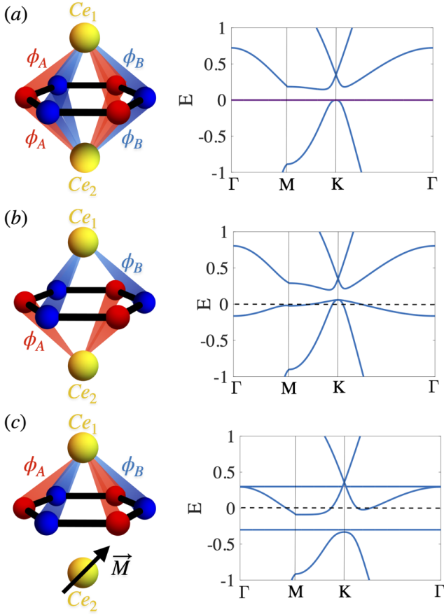
FIG. 2. Schematic of different phases and the corresponding excitation spectra: (a) a uniform HFL phase where all \phi 's are equal. This phase has flat bands at zero energy and therefore it is unstable. (b) A nematic heavy Fermi liquid where local moments in layer 1 primarily couple to one sublattice whereas the layer 2 couples to the other sublattice. (c) A coexistence of magnetic order and a uniform heavy Fermi liquid.
