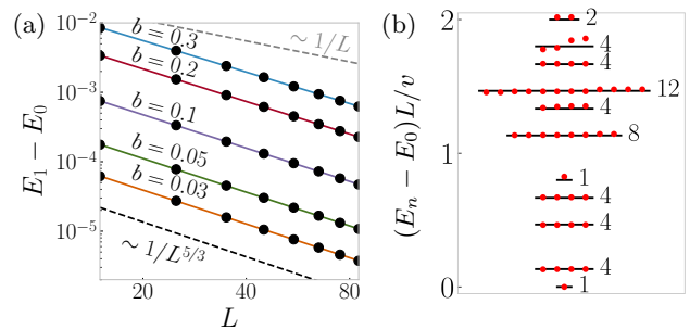
FIG. 2. Edge modes and boundary dissolution at SPT criticality. We consider Eq. (5) with open boundaries. (a) For b < 1 , the boundary spontaneously breaks U^o . This degeneracy’s finite-size splitting matches the CFT prediction \sim L^{-5/3} . Edge modes become exactly degenerate in the CFT limit. (b) At b = 1 , the boundary undergoes a transition between two distinct symmetry-breaking phases. Here, we find a unique ground state. Red dots denote the numerically extracted universal finite-size spectrum (for L = 25 ; here v = 3\sqrt{3}\pi ). Remarkably, this matches the spectrum of Potts CFT without boundaries (black lines). This signifies that at this point, the bulk-boundary distinction is blurred (see main text).
