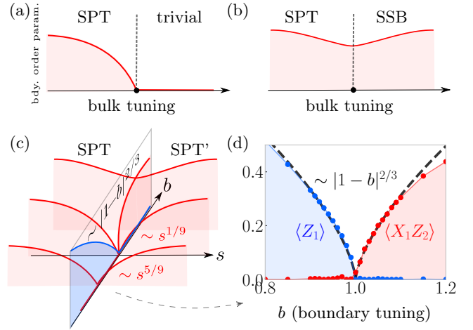
FIG. 1. SPT edge modes, criticality, and boundary DQCP. Panels highlight what happens to SPT edge modes when tuning to quantum criticality. Based on end-to-end long-range order 1 of boundary order parameters: (a) Tuning to trivial phase destroys edge modes. (b) Edge modes can persist upon tuning toward a non-trivial phase, like a symmetry-breaking phase [28, 37, 53]. (c) In this work, we show a richer phenomenology at a transition between two distinct SPT phases protected by \mathbb{Z}_3 \times \mathbb{Z}_3 symmetry (Eq. (5)); there are distinct symmetry-breaking boundary conditions at criticality. (d) Moreover, there is a direct continuous transition (‘DQCP’) between these two by tuning a boundary parameter.
