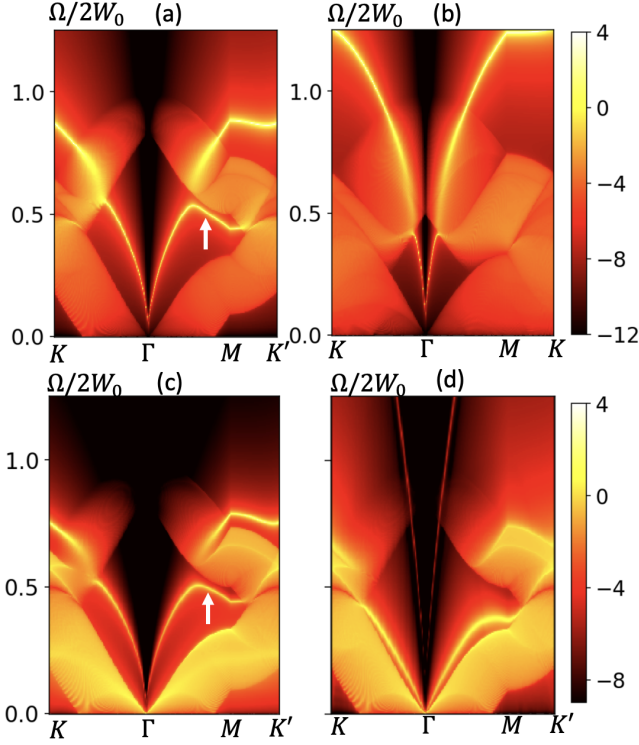
FIG. 2. Numerical results for the spectral function, \log \text{Im}[\chi(q, \Omega)] , for graphene (without substrate in a, b) with 2D Coulomb interaction with \tilde{e}^2 = 15 \simeq 6\tilde{e}_{\text{real}}^2 . The Fermi-energies are (a) E_F/W_0 \simeq 0.83 (b) E_F/W_0 \simeq 0.5 , respectively, where E_F is measured relative to charge neutrality. The plasmon is repelled from the inter-band continuum, and its dispersion develops a negative slope in the region indicated by the white arrows. Numerical results for \log \text{Im}[\chi(q, \Omega)] for graphene on a metallic substrate (without direct electron tunneling) coupled through Coulomb interaction with \tilde{e}^2 = 7 for (c) v_F^{\text{sub}} < v_F^G , and (d) v_F^{\text{sub}} > v_F^G . The red line with the largest slope is the plasmon mode of the substrate.
