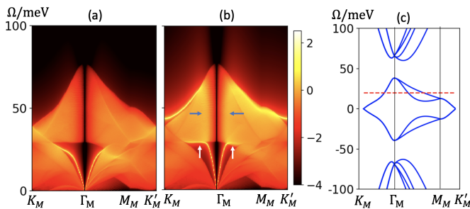
FIG. 3. Numerical results for the dielectric function (Eq. 10), \log \text{Im}[\epsilon^{-1}(q, \Omega)]_{\mathcal{G}=0} , for the model with interactions projected to flat-bands, for twisted bilayer graphene at \theta = 1.4 for (a) realistic parameters, and (b) enhanced Coulomb interaction (see main text). The level-repulsion associated with the plasmon is marked by white arrows. (c) Band structure at \theta = 1.4 , with dashed line denoting the chemical potential E_F = 20 meV.
