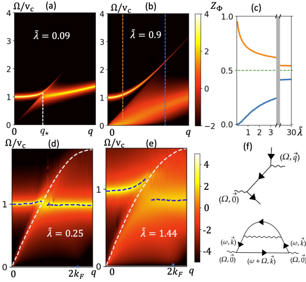
FIG. 1. The response function \log[\text{Im}D(\mathbf{q}, \Omega)] in Eq. 3 obtained from Eq. 1, evaluated at (a) weak ( \tilde{\lambda} = 0.09 ) and (b) strong ( \tilde{\lambda} = 0.9 ) coupling, respectively. We introduce a small broadening, \eta = 0.01 , for visualization purpose when evaluating \text{Im}D(\mathbf{q}, \Omega + i\eta) . The white vertical dashed line in (a) labels the momentum q_* at which the collective mode crosses the onset of the ph continuum when \lambda = 0 . (c) Numerically obtained Z_\Phi as a function of \tilde{\lambda} for two different q values (vertical colored dashed lines in (b)). We set \tilde{\Delta} = 0.5 to be in the regime where the asymptotic limit in Eq.5a is justified. (d)-(e): Disorder-averaged results for \log[\text{Im}D(\mathbf{q}, \Omega)] for the random flavor model with t_c = 1 , \Delta = 1 , \mu = -1.25t_c and interaction strengths (d) \lambda = 0.5 , and (e) \lambda = 1.2 , respectively. The corresponding \tilde{\lambda} is defined as described in the main text. White dashed lines denote the onset of the continuum. Blue dashed lines denote the peak associated with \text{Im}[D(\mathbf{q}, \Omega)] , corresponding to the renormalized collective mode. The quasiparticle residue, Z_c , is obtained self-consistently by solving the saddle point equation [9], with (d) Z_c \sim 0.9 , and (e) Z_c \sim 0.8 , respectively. (f) Feynman diagrams for multi-particle scattering processes and the leading order self-energy for the collective mode.
