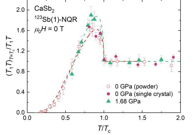
FIG. 4. (Color online) T/T_c dependence of normalized 1/T_1T in low temperature region at ambient pressure and 1.68 GPa. Dashed curves show the fitting results using the BCS model.
