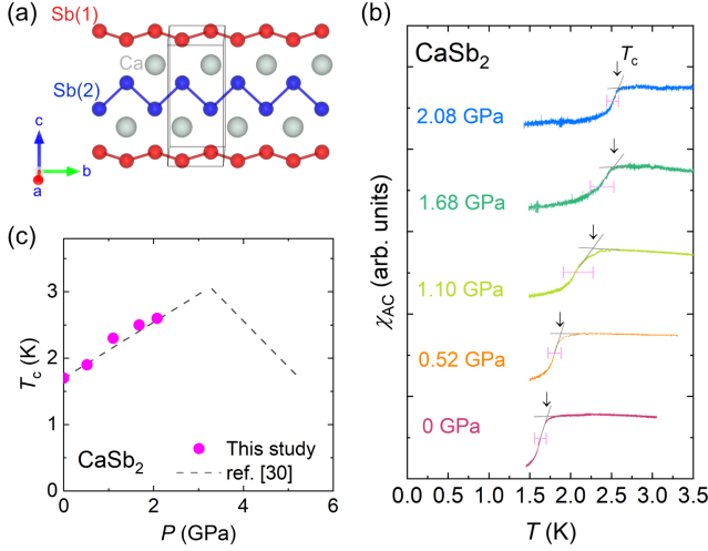
FIG. 1. (Color online) (a) Crystal structure of CaSb 2 with two nonequivalent Sb sites drawn by VESTA [32]. (b) Temperature dependence of the AC susceptibility \chi_{AC} measured by a self-inductance method using a frequency range of 83.5-89.7 MHz under various pressure values. (c) Pressure dependence of T_c . The broken lines are visual guidance identical to those in Ref. [30].
