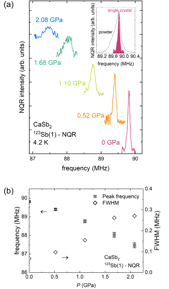
FIG. 2. (Color online) (a) ^{123}\text{Sb}(1) -NQR spectrum of \text{CaSb}_2 measured at 4.2 K under various pressure values. Inset: ^{123}\text{Sb}(1) -NQR spectrum at 0 GPa with that of powder samples. (b) Pressure dependence of peak frequency and FWHM of the NQR spectrum.
