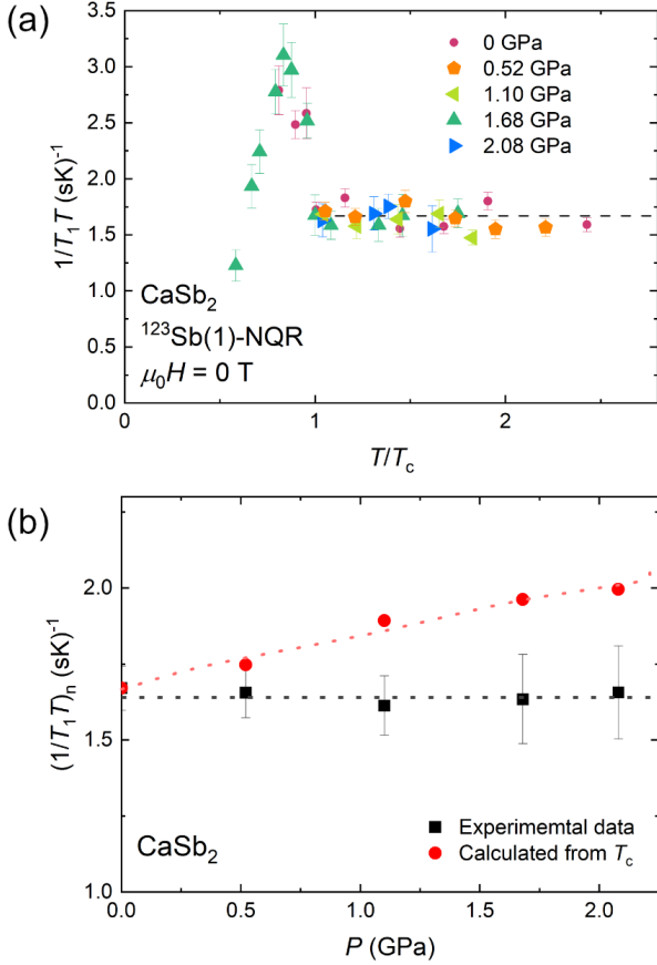
FIG. 3. (Color online) (a) T/T_c dependence of 1/T_1T under various pressure values. (b) Pressure dependence of observed Korringa value (black squares) and calculated ones (red circles).
