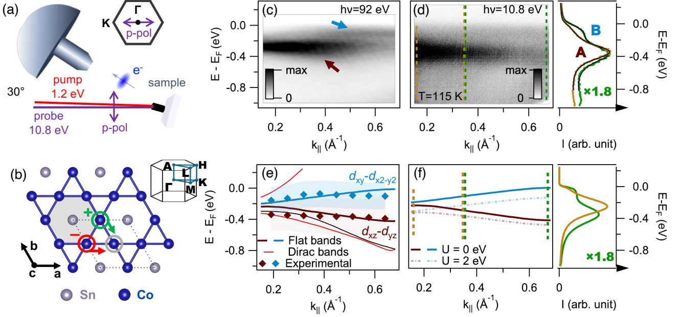
FIG. 1. (a) Scheme of the experimental geometry (top view). Inset: relative orientation of the crystal Brillouin zone and the direction of the p polarization in the geometry of the experiment. (b) Schematic lattice of a CoSn kagome layer. Colored circles denote the adjacent sites with opposite-sign phase of the wavefunction (green and red), causing hopping to the nearest-neighbor (grey) to vanish. The grey-shaded area indicates the real space region of electron confinement. Inset: first Brillouin zone of CoSn. (c) Band structure of CoSn along the \Gamma - K direction measured with 92 eV photons. The blue (brown) arrow indicates the upper (lower) flat band. Data from measurements reported in [30]. (d) Dispersion measured with p -polarized photons at 10.8 eV and 115 K along \Gamma - K (A - H). In the right panel, EDCs extracted in the momentum regions of corresponding color: orange for small momentum values, green for large momentum values. The best fit is overlaid as a black line. A and B identify two Lorentzian peaks used to fit the EDCs. (e) DFT calculations of the band structure of CoSn along the \Gamma - K direction in the vicinity of the Fermi level, already reported in [30]. The upper and lower flat bands are indicated with blue and brown lines respectively, the Dirac band in red and a non-kagome derived band in black. The degrees of freedom of the 3d orbitals from which the two bands originate are also reported. The square markers indicate the position of the two peaks resulting from the fit of the EDCs extracted from the measurement at 10.8 eV. The EDCs are integrated in the momentum region centered at the marker position, with the resulting Lorentzian width indicated as a shaded area. (f) DFT+U [32] calculations for U = 0 eV (solid lines, same as reported in (e)) and U = 2 eV (dashed-dotted lines). The side panel displays the EDCs obtained using the peak positions from the U = 0 eV case and applying the same functional form and parameters (area, width, Gaussian broadening and temperature) obtained from the fits of the experimental data.
