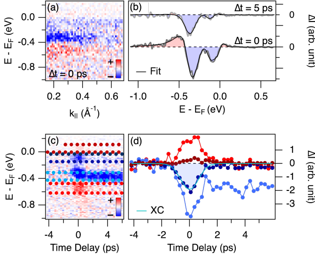
FIG. 2. (a) Difference between the map at time zero and the average before time zero. (b) Differential EDCs integrated in the whole momentum region at 0 and 5 ps time delay. The black superimposed line is the fit, described in the main text. (c) Differential EDCs plotted in a color map as a function of time delay. (d) Time traces extracted in the energy region marked by the dotted lines in (c). The light-blue trace is the gaussian fit to the dark-blue curve.
