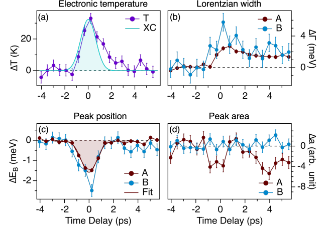
FIG. 3. Variation with respect to equilibrium of the parameters extracted by fitting the dEDCs, as a function of time delay. Bars indicate the uncertainty of the fitting procedure on the parameters. (a) Electronic temperature. The solid line is the gaussian fit reported from Fig. 2(d). (b) Lorentzian width of peak A (brown) and B (light blue). (c) Position (binding energy) of peaks A and B. The solid line is the best fit of the A position dynamics to a Gaussian. (d) Area under each Lorentzian peak.
