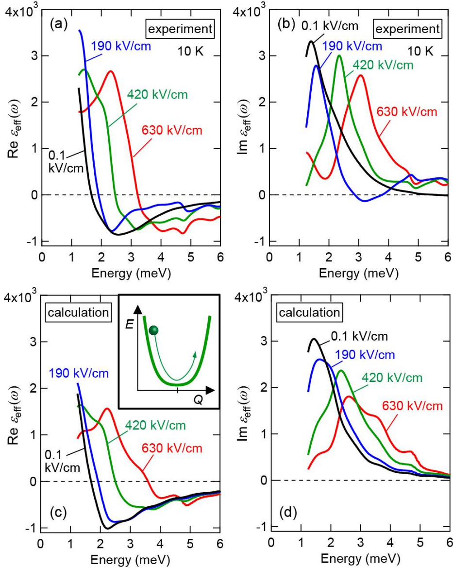
FIG. 2: (a,b) The real (a) and imaginary (b) parts of effective dielectric spectra \epsilon_{\text{eff}}(\omega) at each peak terahertz field at 10 K. (c,d) The model calculation of the effective dielectric spectra \epsilon_{\text{eff}}(\omega) ; the real (c) and imaginary (d) parts. (inset of (c)) Schematic illustration of the positional free energy for phonon including the quartic anharmonic term in addition to the harmonic term.
