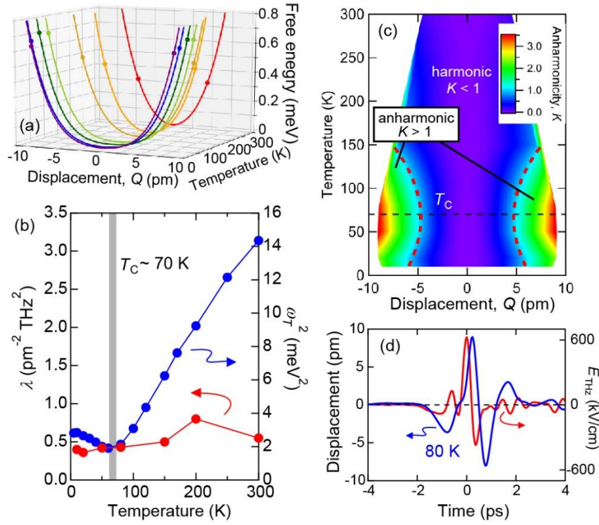
381 FIG. 4: (a) The positional free energy for phonon retrieved from the effective dielectric 382 spectra. The solid circles represent the maximal displacement induced by the terahertz 383 field. (b) Temperature dependence of \omega_T^2 and \lambda . These are coefficients for the harmonic 384 quadratic and anharmonic quartic terms. (c) The contour map of the anharmonicity K . 385 The colored area is limited to the range of actual displacement Q realized by the highest 386 terahertz field. The red dotted curve shows the boundary between the harmonic and 387 anharmonic regimes, where K = 1 . The black horizontal dotted line is the ferroelectric 388 transition temperature T_C \sim 70 K. (d) The time evolution of calculated atomic 389 displacement at 80 K (blue curve) and incident terahertz light field (red curve).
