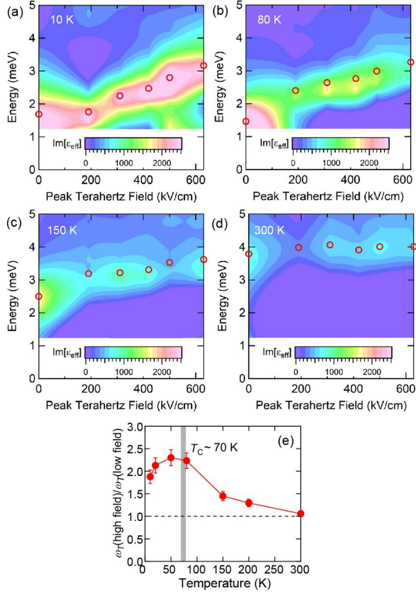
373 FIG. 3: (a-d) Color coded spectra of \text{Im} \epsilon_{\text{eff}}(\omega) under strong terahertz field at 10 K (a), 80 374 K (b), 150 K (c), and 300 K (d). The red open circles represent the resonance energies of 375 the soft phonon. (e) The temperature dependence of the resonance energy at the highest 376 terahertz field ( E_{\text{THz}} = 630 kV/cm) normalized by that at the lowest terahertz field ( E_{\text{THz}} 377 \sim 0.1 kV/cm). The gray bar represents the T_C \sim 70 K. The error bar represents the 378 statistical error in ten measurements.
